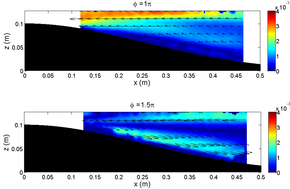
Figure 3: Velocity field data from experimental simulation of Luzon. (top) peak westward tidal current. (bottom) zero tidal current.
