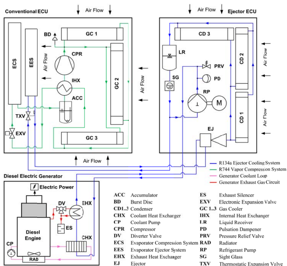
Figure 2: Schematic of the trailer-mounted integrated waste heat recovery ejector system
