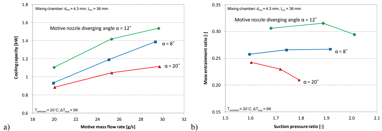
Figure 4: a) Experimental results of cooling capacity for various motive nozzle diverging angles as a function of the motive mass flow rate; b) experimental results of mass entrainment ratio for various motive nozzle diverging angles as a function of the suction pressure ratio
