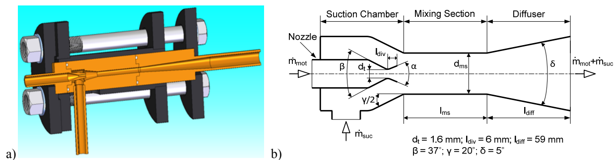
Figure 3: a) 3-D CAD cut-away view of the modular ejector; b) schematic of ejector with characteristic dimensions
