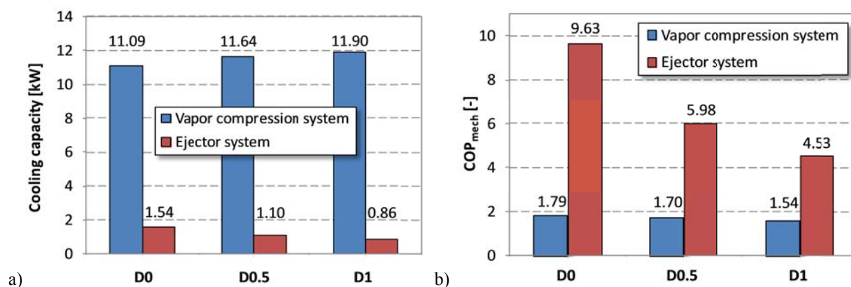
Figure 8: Comparison of a) cooling capacity and b) COP mech between the conventional and vapor jet ejector system at various ambient temperature conditions
