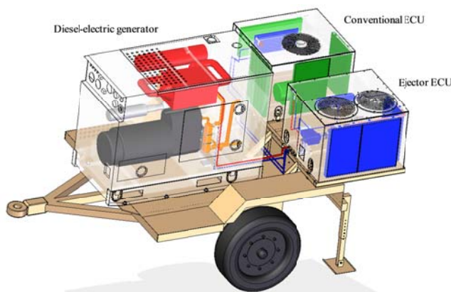
Figure 1: 3-D CAD drawing of the trailer-mounted technology demonstrator
