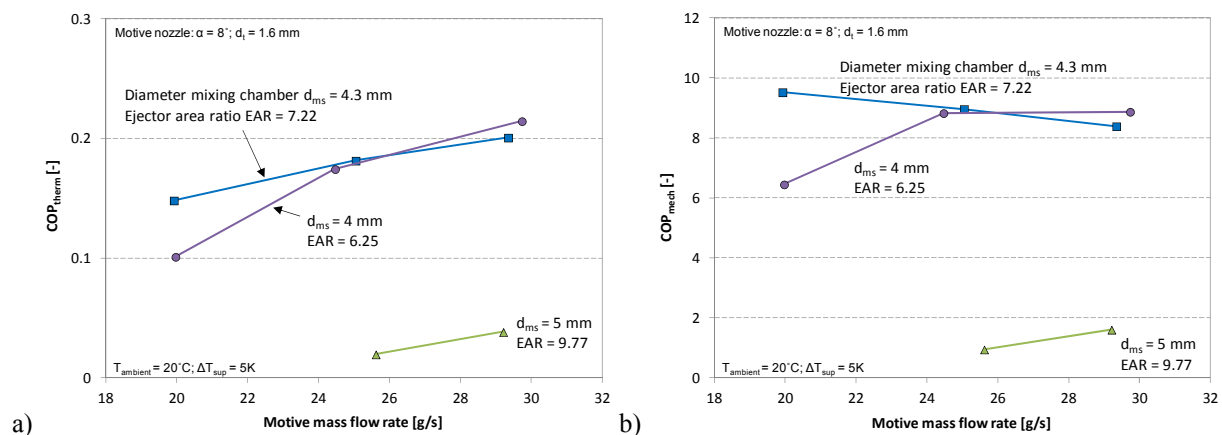
Figure 7: Experimental results of a) COP_{therm} and b) COP_{mech} for different ejector area ratios as a function of the motive mass flow rate
