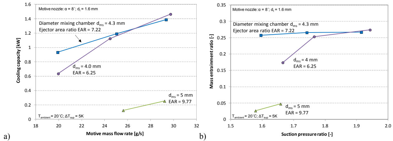
Figure 6: a) Experimental results of cooling capacity for different ejector area ratios as a function of the motive mass flow rate; b) experimental results of the mass entrainment ratio for different ejector area ratios as a function of the suction pressure ratio
