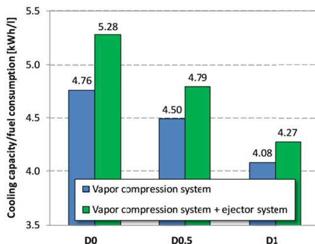
Figure 9: System comparison of cooling output per fuel consumption
