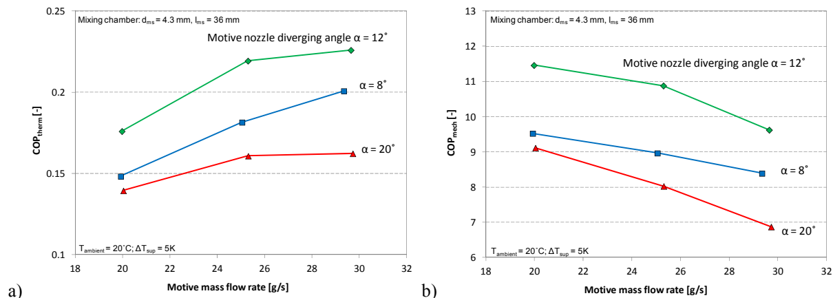
Figure 5: Experimental results of a) COP_{therm} and b) COP_{mech} for various motive nozzle diverging angles as a function of the motive mass flow rates
