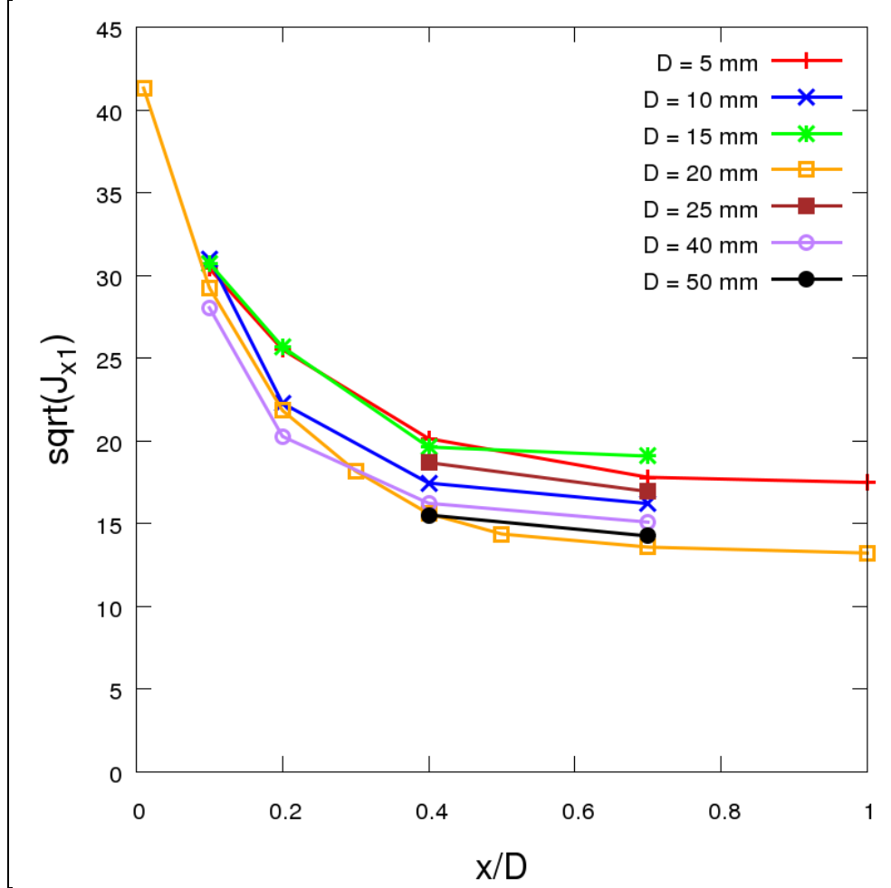
Figure 6. Square root of J_{x1} at the center-plane vs. friction coefficient for several specimen thicknesses.
