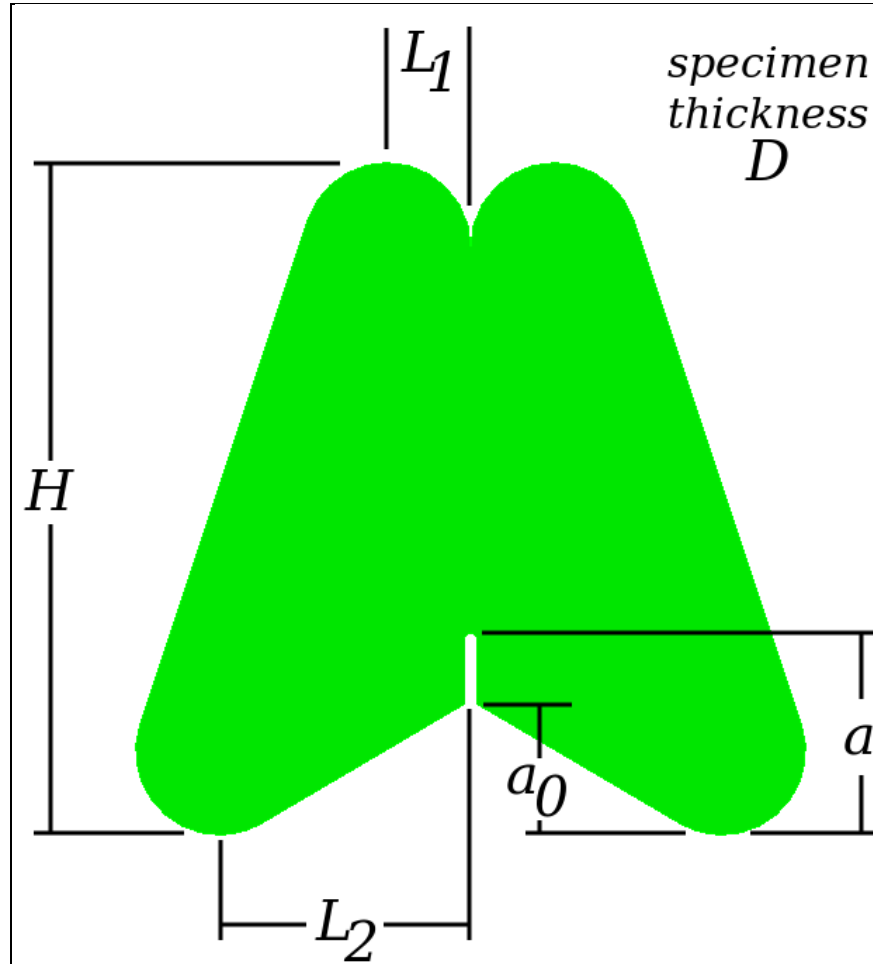
Figure 2. Generalized geometry for butterfly bending specimen.
