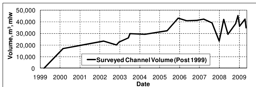
Figure 4. Volumetric change of the entrance channel to Shark River Inlet after 1999.
