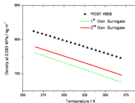
Figure 2.37. Measured density for Jet-A POSF 4658 at 0.083MPa (symbols [36]) and calculated densities [100] at 0.083MPa for 1 st generation (n-decane/iso-octane/toluene 42.7/33.0/24.3 mole %, dashed line) and 2 nd generation (n-dodecane/iso-octane/1,3,5 trimethylbenzene/n-propylbenzene 40.41/29.48/7.28/22.83 mole %, solid line) POSF 4658 surrogate fuels.
