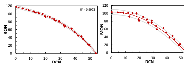
Figure 2.8. Research Octane (RON)-DCN and Motored Octane (MON)-DCN correlations based on IQT experimental data for ternary (n-heptane/iso-octane/toluene) reference gasoline mixtures. Gray bands are \pm 3.5 and \pm 6.5 units from best fit polynomials, respectively. From [46].
