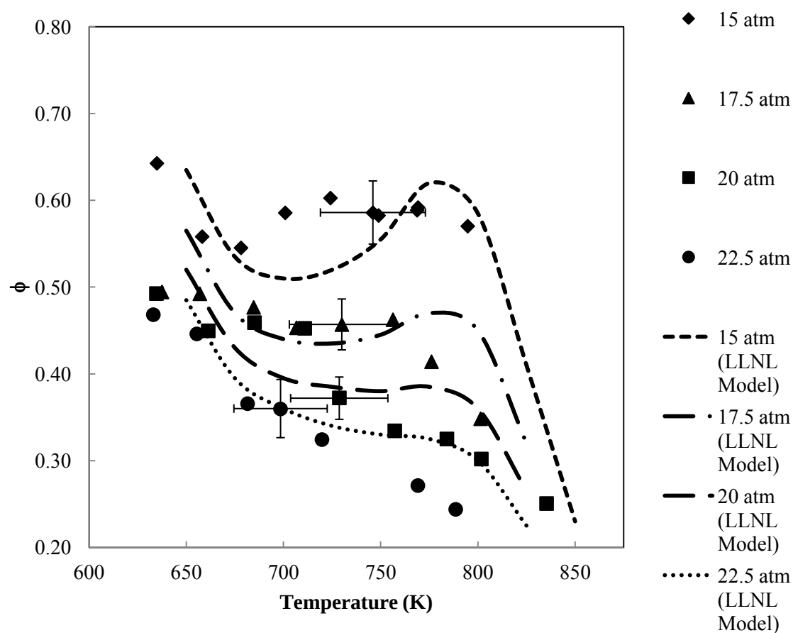
Figure 5.50 Experimental results and model predictions for the threshold equivalence ratio as a function of temperature at a residence time of 125 ms. Symbols represent experimental results from the current study and black lines represent model results using the LLNL mechanism [35].
