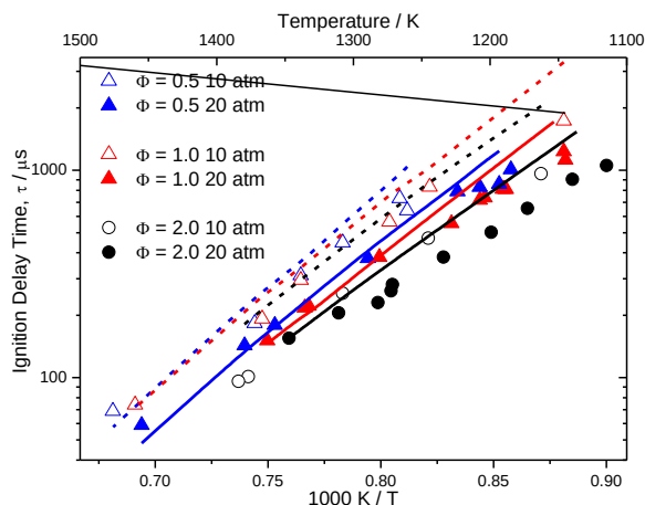
Figure 3.19. Measured (symbols) and computed (lines) reflected shock ignition delays for 1,3,5-trimethylbenzene/air mixtures. Hollow symbols and dashed lines are ~10 atm conditions, solid symbols and solid lines are ~20 atm conditions. Stoichiometric combustion is identified by an equivalence ratio of unity.
