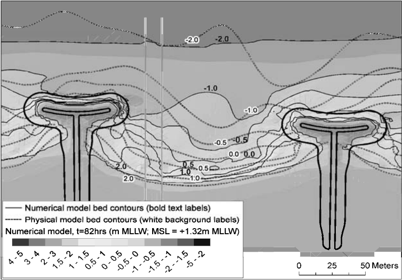
Fig. 9. Numerical Model 2 plan morphology vs. physical model at time t=82\text{hrs} .
