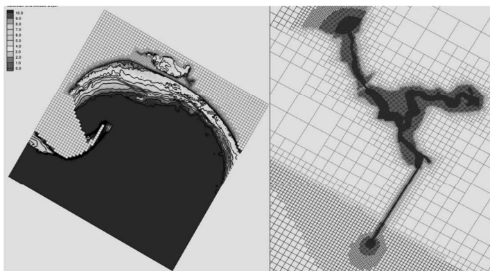
Fig. 4. CMS Grid Doman (a, left), and Moon Pond Quadtree grid (b, right)
