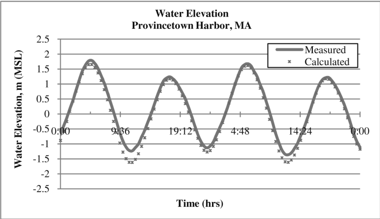
Fig. 5. Water elevation calibration curve, 12 hour snapshot
