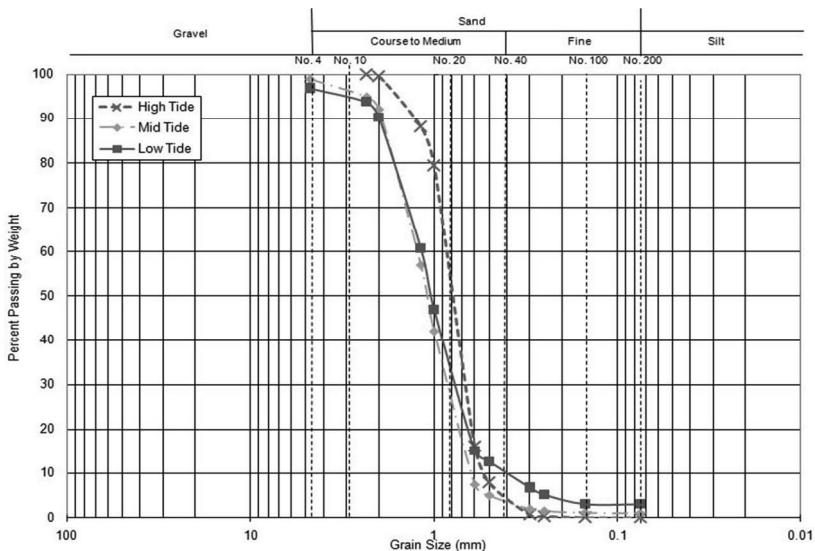
Fig. 3. Grain Size Analysis
