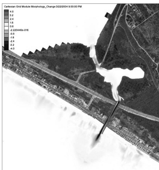
Fig. 6. Morphology change for 15.2 m wide inlet alternative
