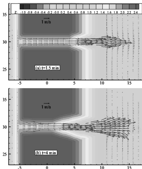
Fig. 5. Simulated flow pattern and breach topography (background as bed elevation contours in meter; x and y coordinates in meter).
