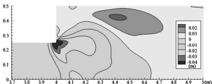
Fig. 2. Calculated total bed changes near the sudden expansion.
