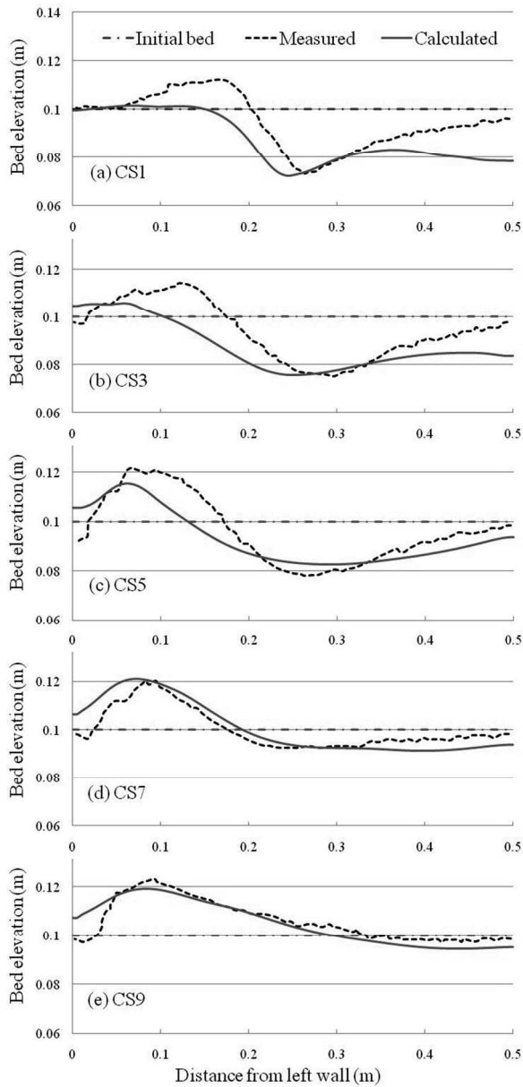
Fig. 3. Measured and calculated final bed levels at cross-sections CS1, CS3, CS5, CS7, and CS9.
