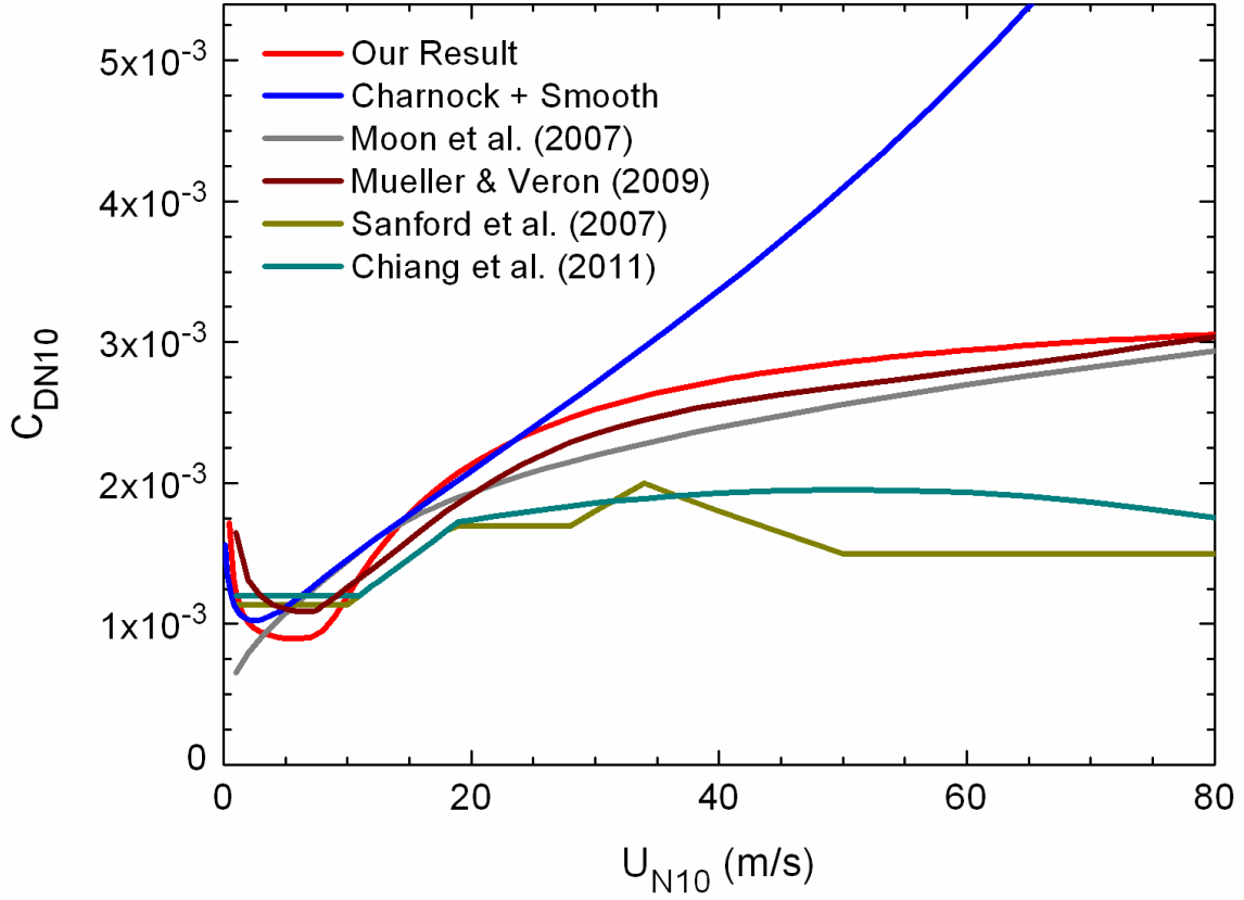
Figure 4. The neutral-stability, 10-m drag coefficient, C_{DN10} , is plotted against U_{N10} for U_{N10} between 0 and 80 m/s. Our hyperbola, (8), and the theoretical results of Moon et al. (2007) and Mueller and Veron (2009) agree well; all predict that C_{DN10} rises rapidly for wind speeds up to about 20 m/s, then rolls off to values of about 3.0 \times 10^{-3} , and becomes nearly constant for U_{N10} above 100 m/s. The commonly used “Charnock + Smooth” relation, on the other hand, predicts that C_{DN10} rises without bound. The Sanford et al. (2007) and Chiang et al. (2011) curves, which are based on Powell et al. (2004), roll off to much lower values, of order 1.5 \times 10^{-3} to 1.9 \times 10^{-3} , and are probably too low in hurricane-strength winds.
