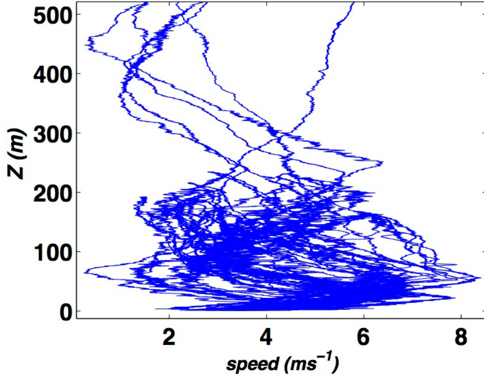
Figure 3. Fifty vertical profiles of wind speed that the Long-EZ aircraft measured between the sea surface and 500 m on 8 August 2001 during the CBLAST weak wind pilot experiment near Martha’s Vineyard. The vast majority of the soundings include a wind maximum (jet) below 100 m. Sometimes the jet is quite sharp.
