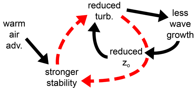
Figure 2. Warm air advection off a coast over cooler water leads to stable stratification in the near-surface air. This stratification inhibits the downward momentum flux from aloft such that the turbulence is reduced in the off-shore flow. In turn, wave growth and the associated surface roughness ( z_0 ) are limited. Consequently, the stability increases further in a feedback loop that can ultimately decouple the atmosphere and the sea surface.
