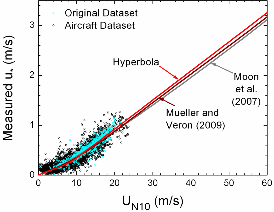
Figure 1. The “original” and “aircraft” datasets [see Andreas et al. (2012) for descriptions] are plotted as u_* versus U_{N10} for U_{N10} up to 60 m/s. In aerodynamically smooth flow—low U_{N10} —the data tend to follow the straight line implied by (7). In aerodynamically rough flow— U_{N10} above 9 m/s—the data follow (6). We thus smoothly joined these two lines with the hyperbola (8). The theoretical results from Moon et al. (2007) and Mueller and Veron (2009) are not much different from our main straight-line result (6) for U_{N10} above 20 m/s.
