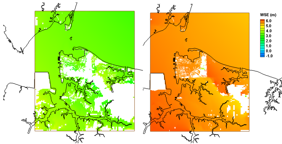
Figure 10. The maximum water surface elevation due to the 100-year return tropical storm under the existing condition and the 2.0-m sea level rise scenario.
