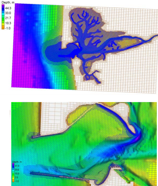
Fig. 5. The telescoping grid and refinement near Damon Point.
