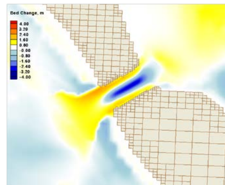
Fig. 19. Calculated morphology change due to hypothetical breach.
