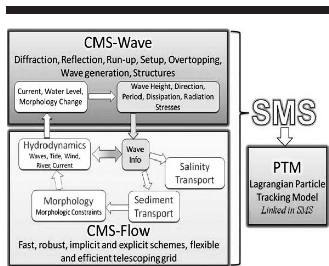
Figure 1. The CMS operational flow chart.
