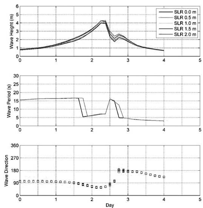
Figure 7. Wave parameters of the 100-year return storm under the existing condition and four sea-level-rise scenarios. (Color for this figure is only available in the online version of this paper.)
