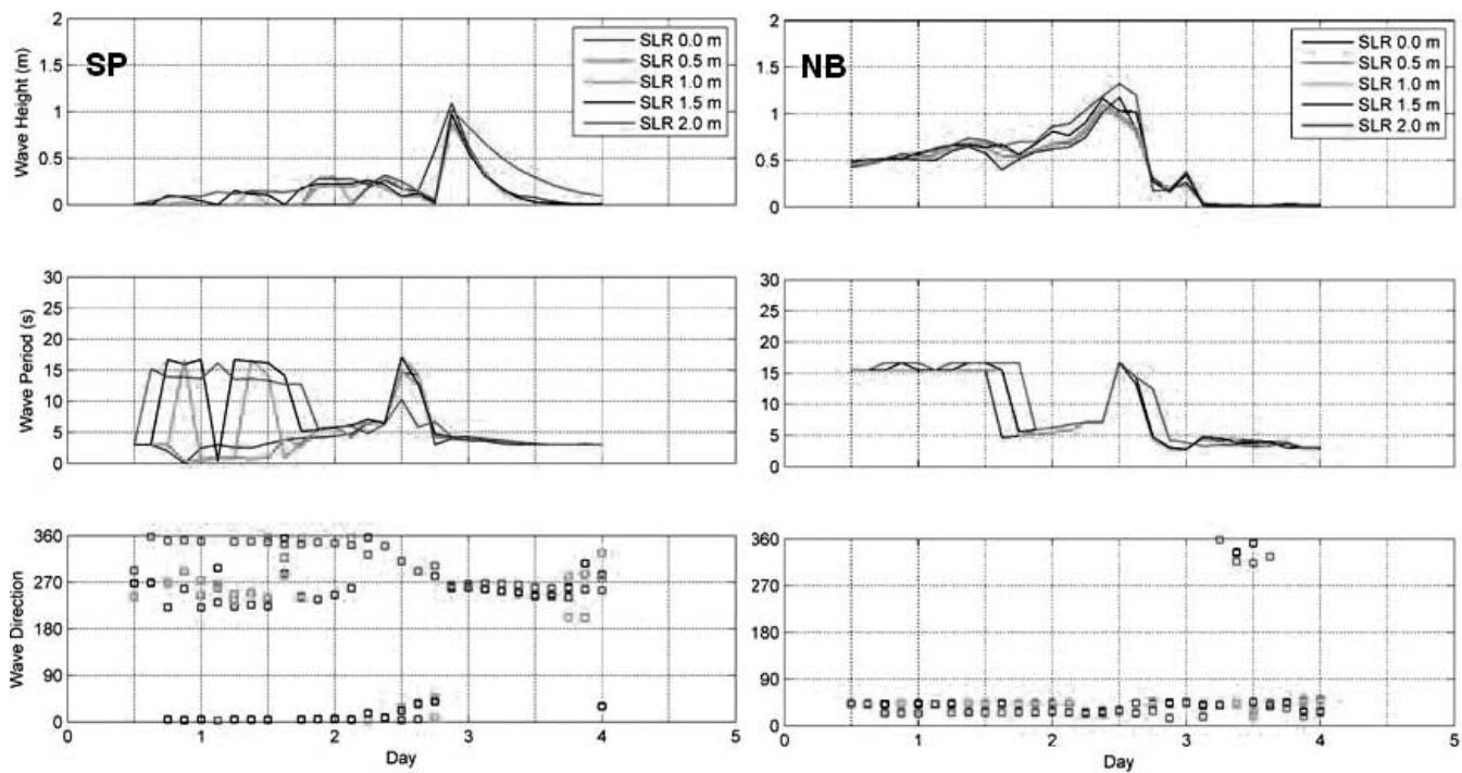
Figure 18. Wave parameters of the 100-year return tropical storm under the existing condition (0 m) and the four sea-level-rise scenarios at sites SP and NB. (Color for this figure is only available in the online version of this paper.)
