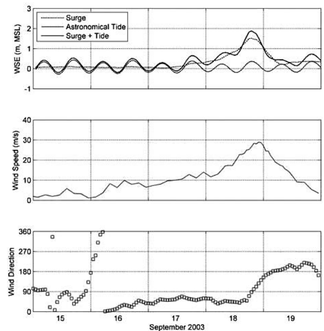
Figure 10. Surge, tide, and wind of Hurricane Isabel at NOAA gauge 8638610 (Sewells Point, Virginia).
