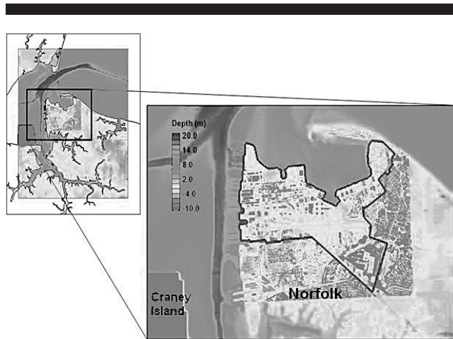
Figure 2. Topographic map of the study area. The blue line outlines Naval Station Norfolk. (Color for this figure is only available in the online version of this paper.)
