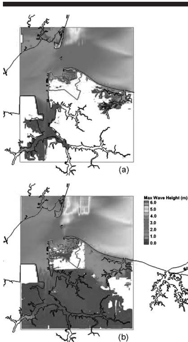
Figure 17. The maximum wave height due to 100-year return tropical storm under (a) the existing condition and (b) the 2-m RSLR scenario. (Color for this figure is only available in the online version of this paper.)
