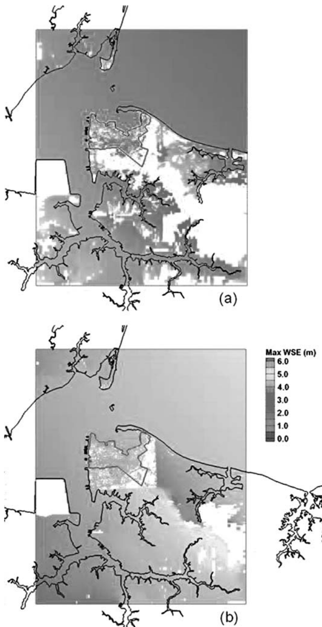
Figure 15. The maximum water-surface elevation due to 100-year return tropical storm under (a) the existing condition and (b) the 2-m RSLR scenario. (Color for this figure is only available in the online version of this paper.)
