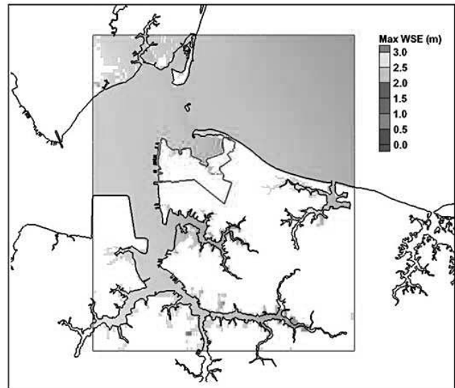
Figure 13. The maximum water-surface elevation due to Hurricane Isabel. (Color for this figure is only available in the online version of this paper.)
