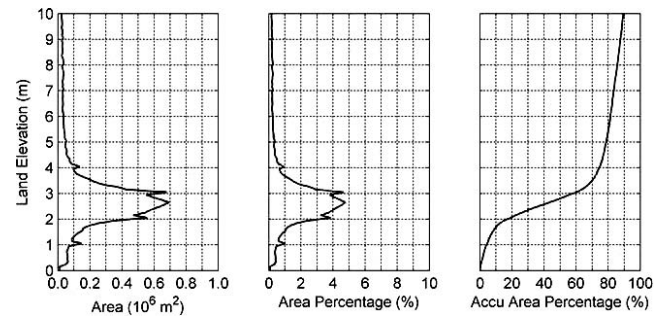
Figure 3. Areal distribution as a function of land-surface elevation (relative to MSL) in Naval Station Norfolk
