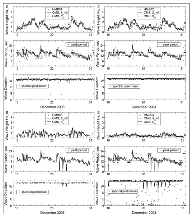
Figure 2. Measured and calculated waves at HMB1 to 4, 10-31 December 2003.
