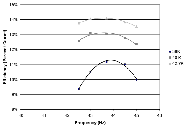
FIGURE 4. Frequency vs. Efficiency (TR 290K).
