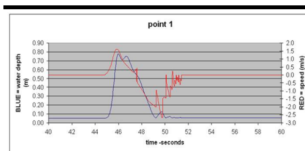
Figure 12: Surge response at Point 1.
