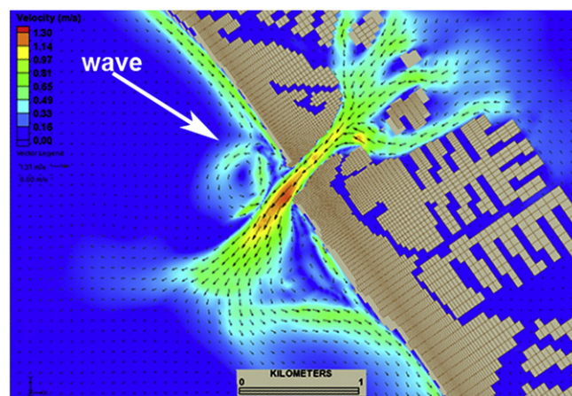
Fig. 16. Calculated wave-current interaction at John's Pass, under a high northerly approaching (arrow) wave with H_s = 2.0 m and T_p = 6.1 s, during a peak ebbing tide. Note the large eddy developed at the converging longshore current and the ebb jet, which is likely responsible for the development of the channel margin linear bar.
