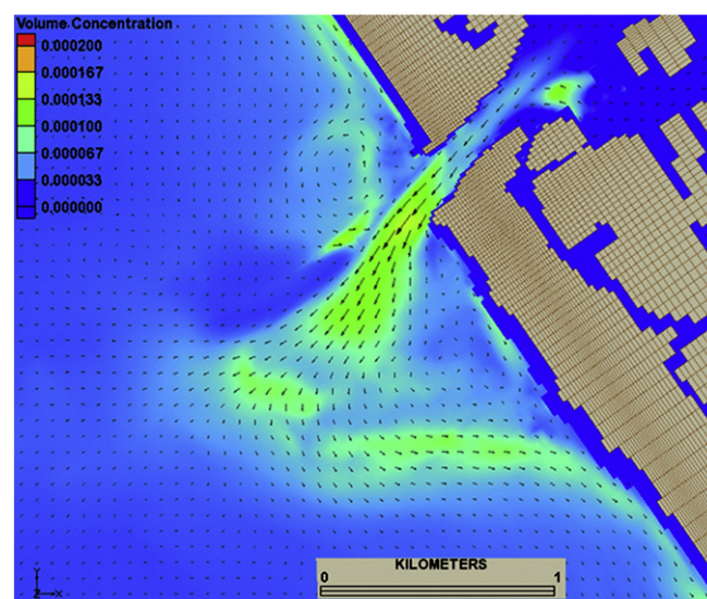
Fig. 20. Calculated depth-averaged sediment volume concentration (dimensionless) and transport vectors at John's Pass, under a high northerly approaching wave with H_s = 2.0 m and T_p = 6.1 s, during a peak ebbing tide. Note the elevated sediment concentration over the shallow part of the ebb delta, indicating the active sediment suspension by breaking waves. The converging sediment flux along the north side of the inlet channel is likely responsible for the development of the channel margin linear bar.
