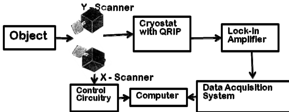
Figure 4. Schematic measurement setup system.
