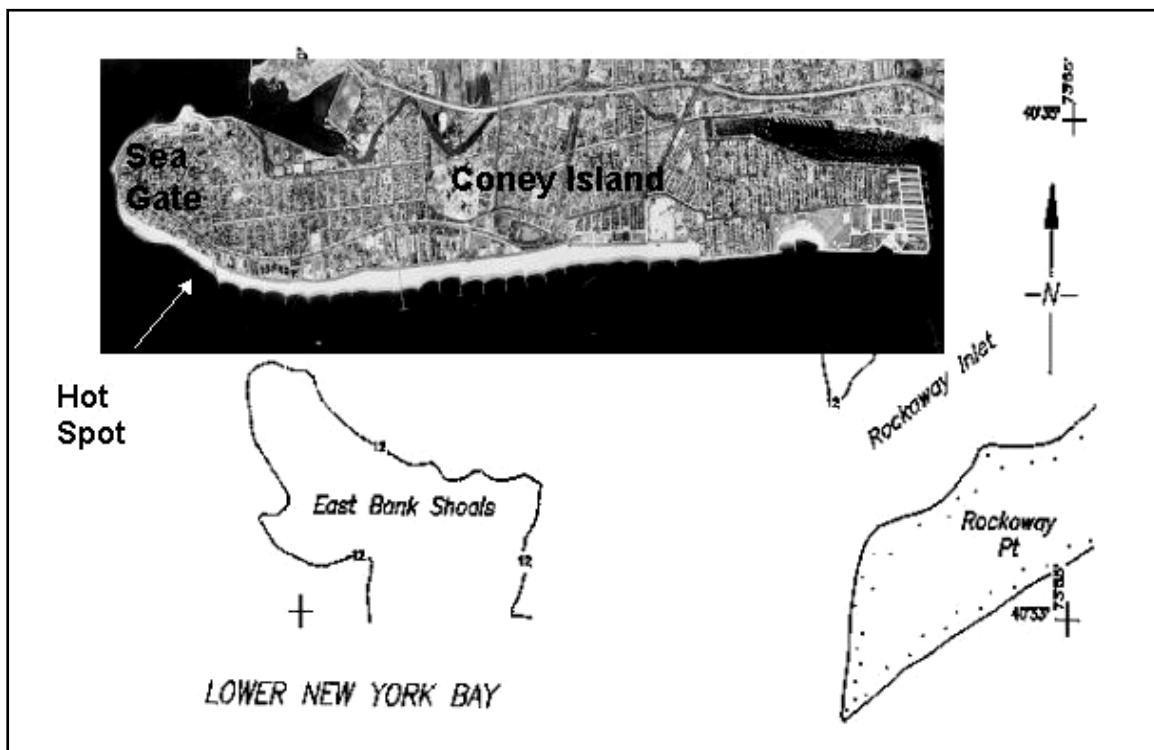
Figure 2. Coney Island, NY hot spot location
