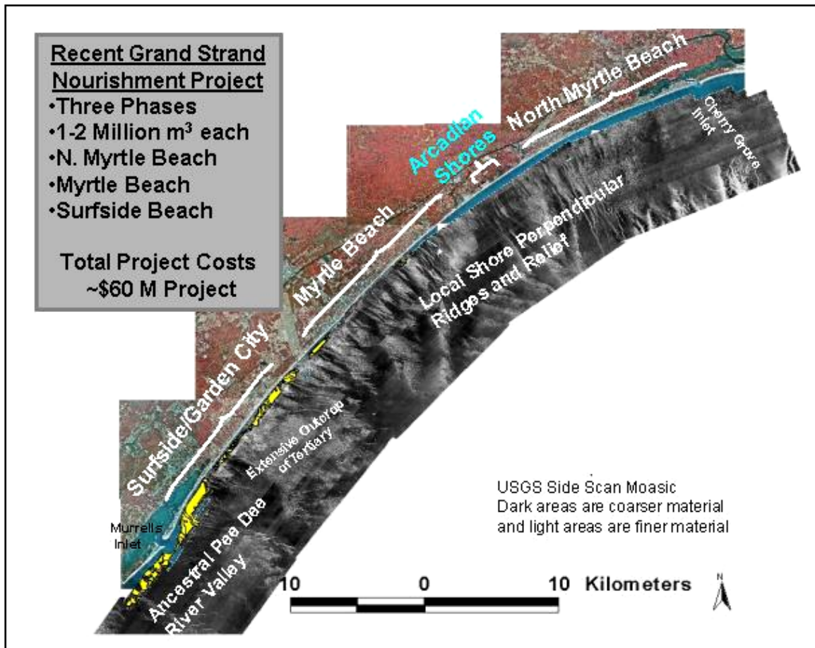
Figure 12. Variation in nearshore geology along the three phases of the Myrtle Beach, SC project (courtesy of Paul Gayes, Coastal Carolina University)
