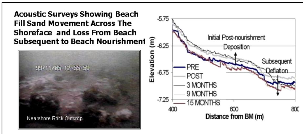
Figure 13. Nearshore rock outcrop and deflation of fill profile at Myrtle Beach, SC (courtesy of Paul Gayes, Coastal Carolina University)
