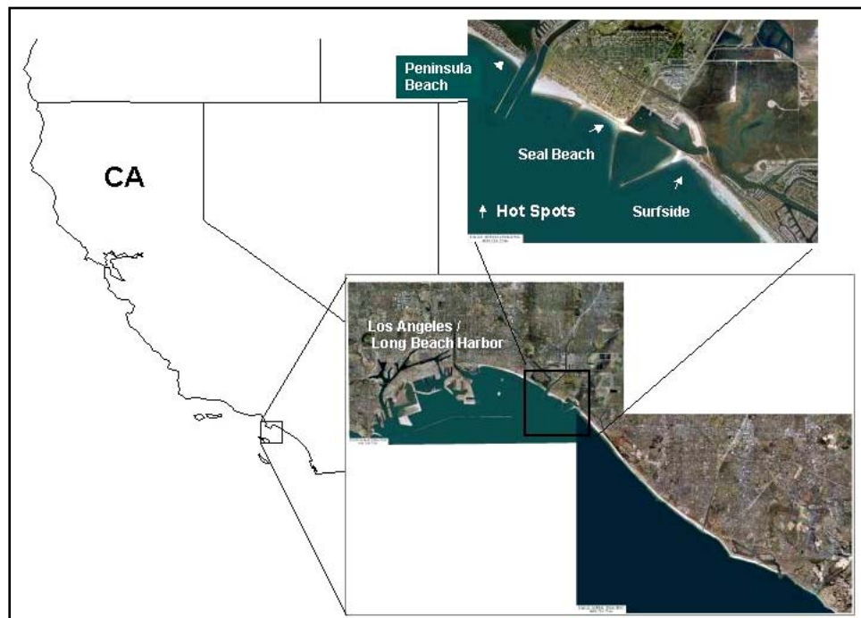
Figure 21. Location of three hot spots at Surfside, Seal Beach, and Peninsula Beach along southern California coast (courtesy of Chuck Mesa, Los Angeles District)
