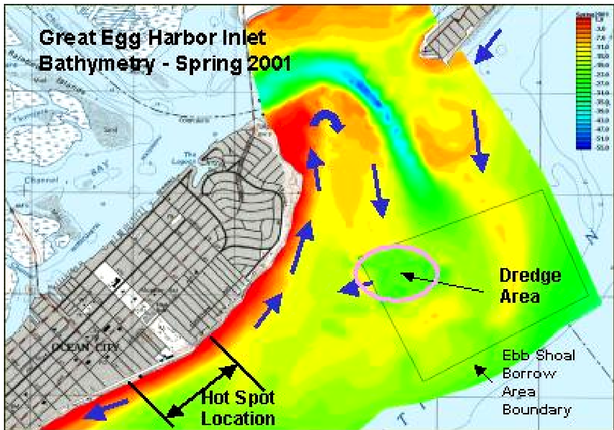
Figure 6. Location of hot spot area, designated borrow area with dredged area on western edge and suspected longshore circulation at Great Egg Harbor Inlet, NJ (courtesy of Monica Chasten and Rob Lowinski, Philadelphia District)
