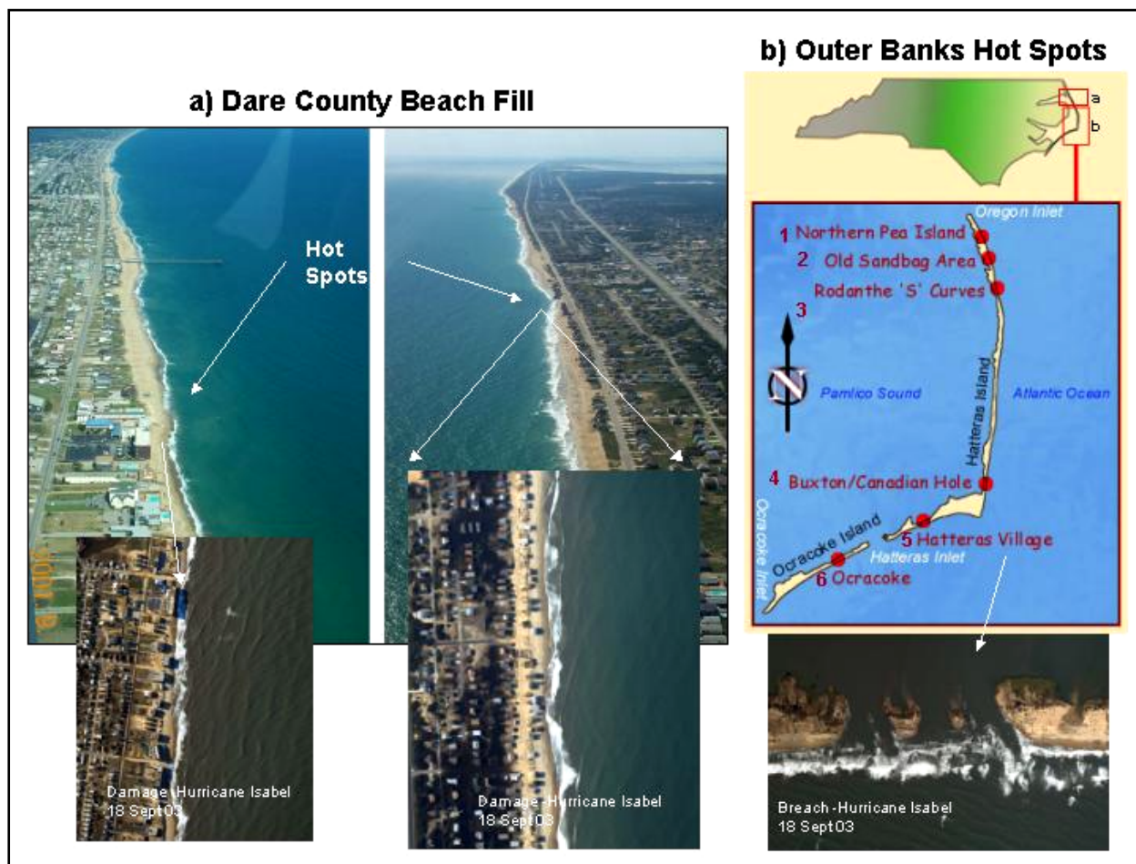
Figure 11. Hot spot locations: (a) along Dare County, NC coast (courtesy of William Birkemeier, CHL), and (b) Outer Banks (courtesy of John McCormick, Wilmington District), showing overwash and inlet breach at hot spot locations resulting from Hurricane Isabel (NCDOT)
