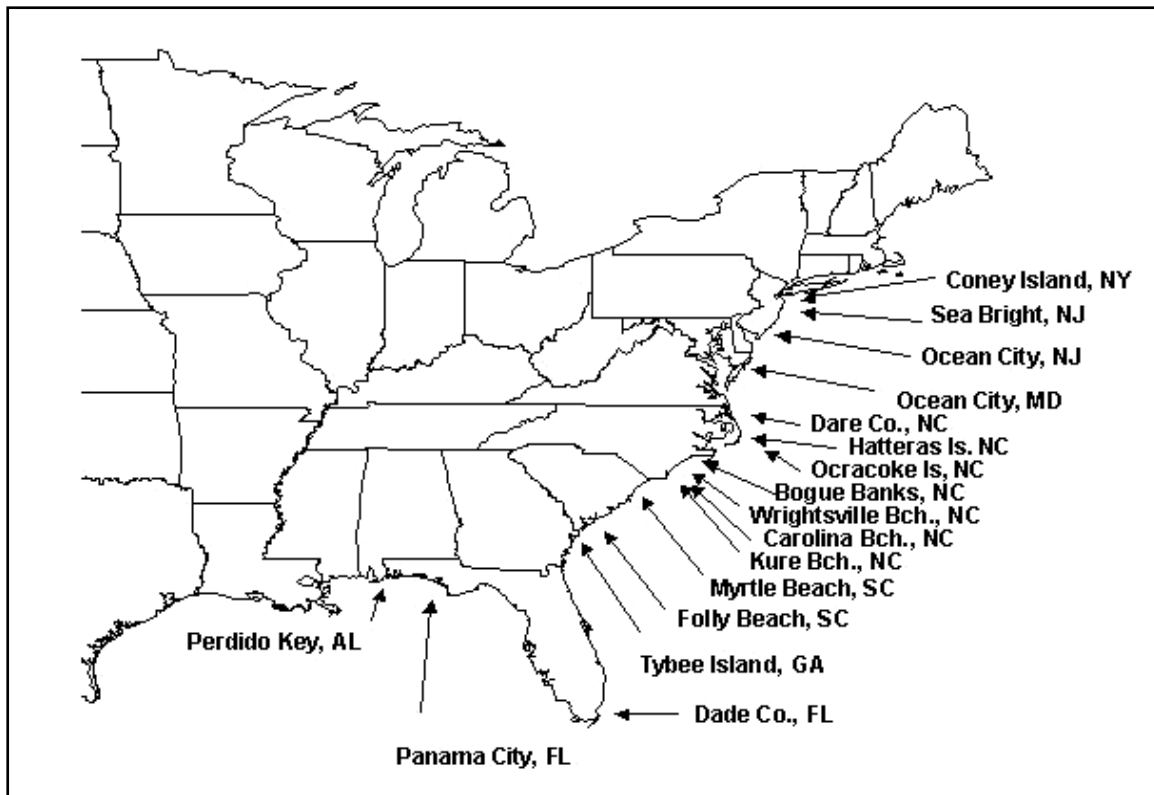
Figure 1. Location of beach-fill project hot spots discussed in paper
