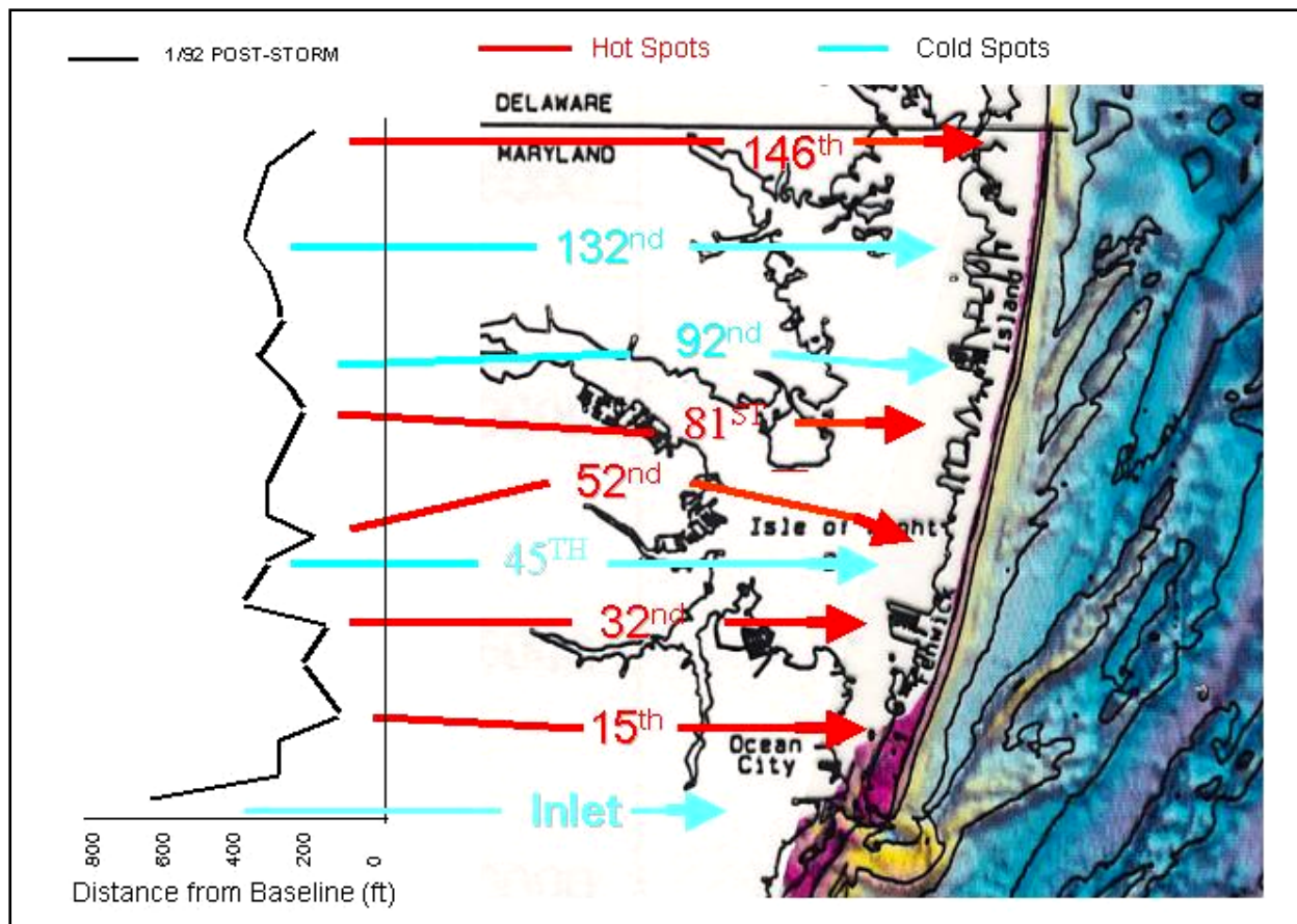
Figure 9. Plot of shoreline change after 1993 storm relative to 1991/1992 fill placement and location of hot (red) and cold (blue) spots relative to nearshore bathymetry of Ocean City, MD (Stauble and Bass 1999)
