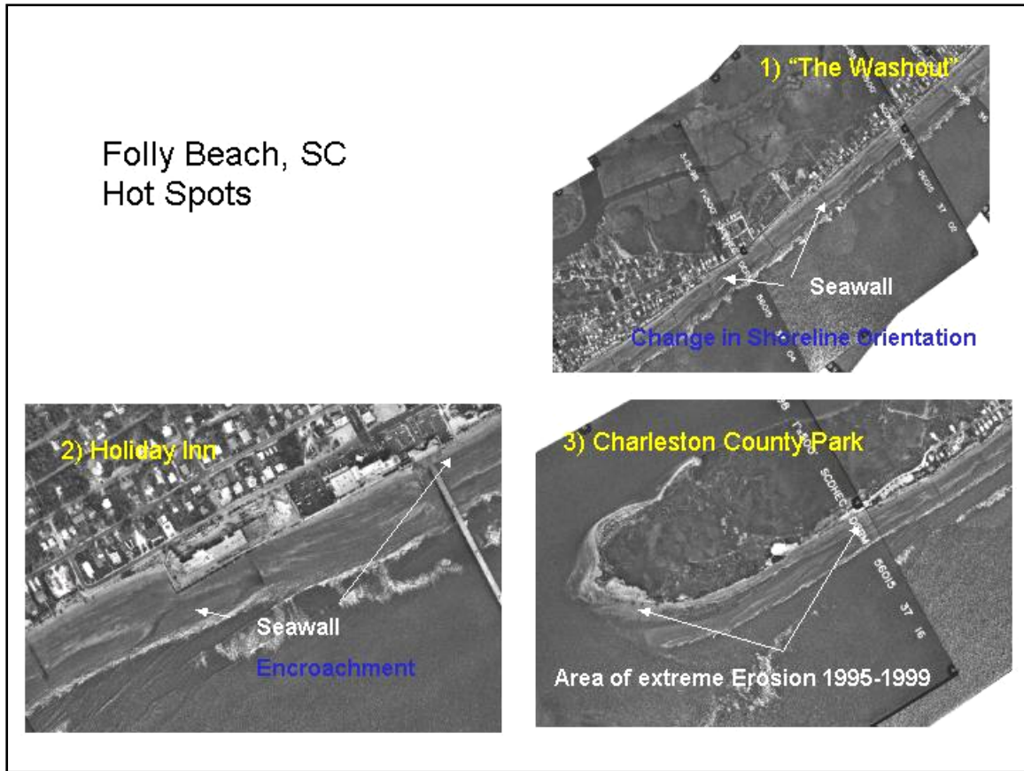
Figure 14. Location of three hot spots at Folly Beach, SC, fill project (courtesy of Paul Gayes, Coastal Carolina University)
