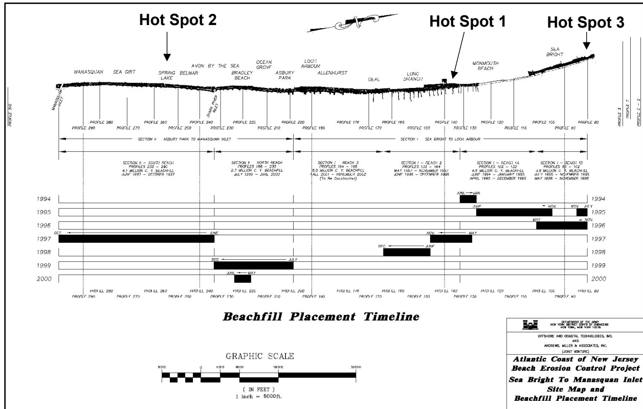
Figure 4. Construction sequence of the Sea Bright New Jersey project (courtesy of Lynn Bocamazo, New York District)
