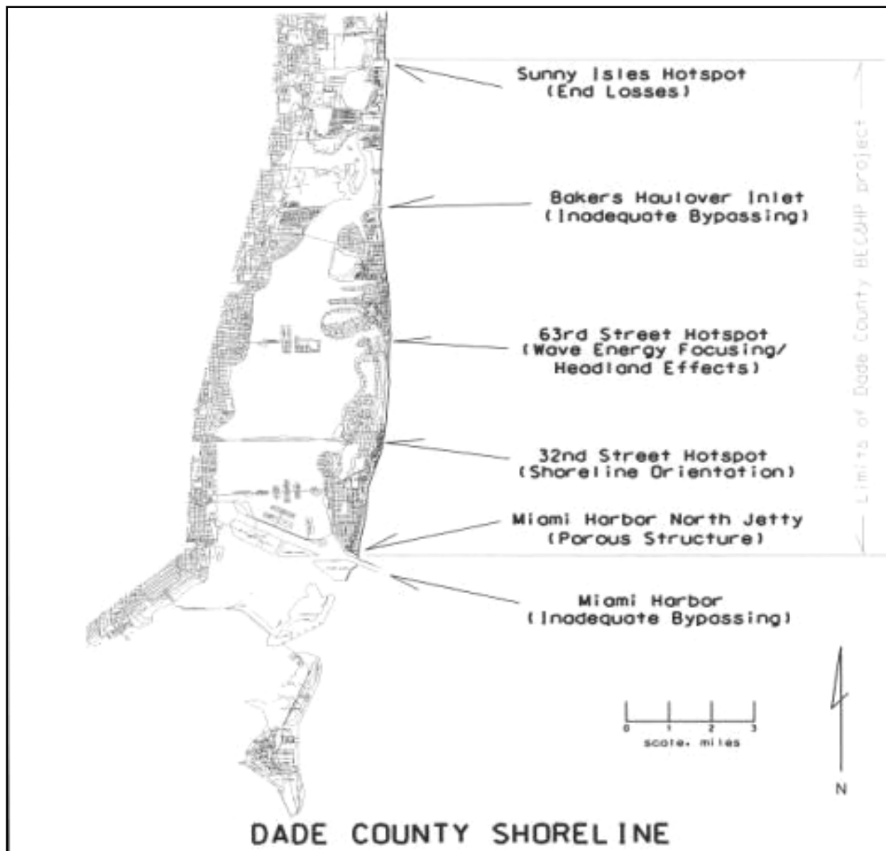
Figure 17. Hot spot locations along the Dade County, FL, fill project (courtesy of Tom Martin, Jacksonville District)
