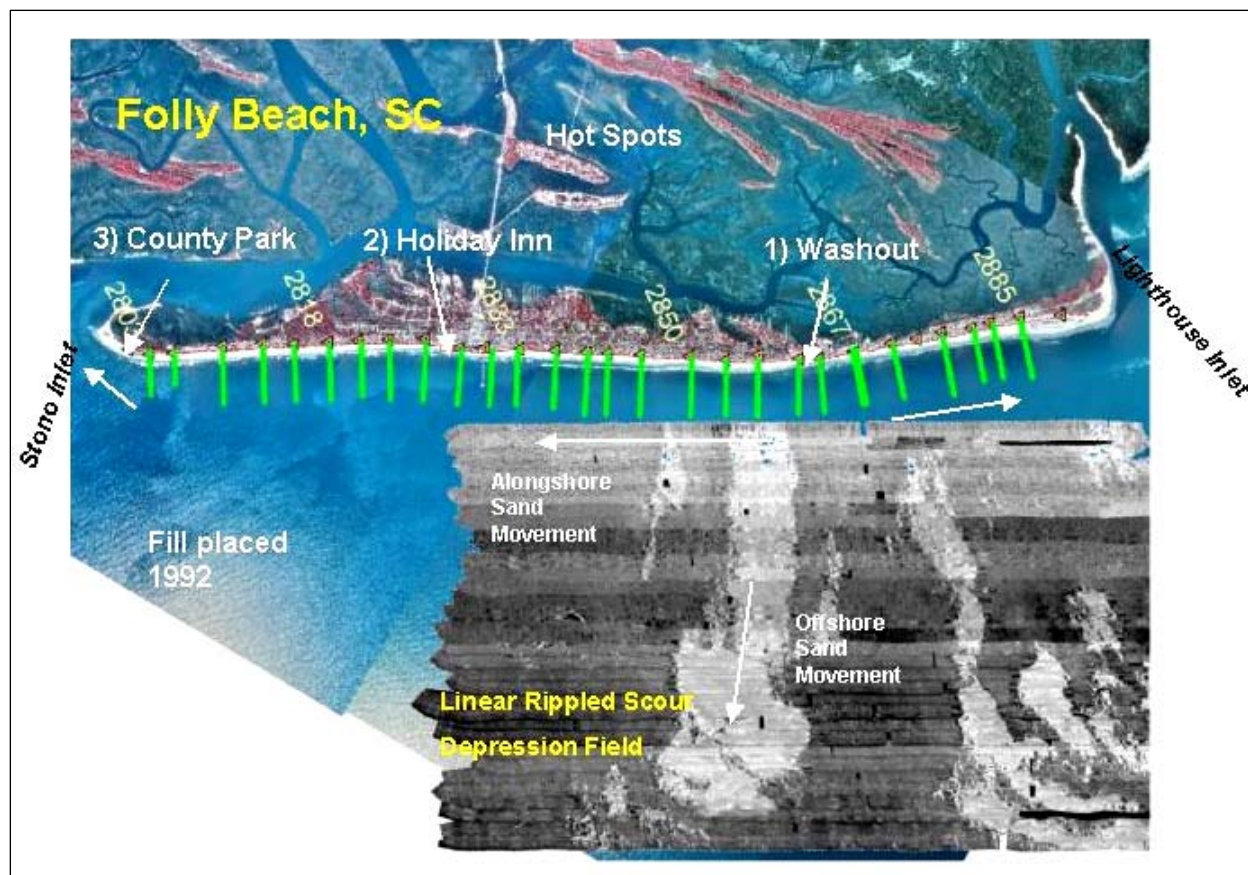
Figure 15. Nearshore geology of Folly Beach, SC, in relation to the three hot spots (courtesy of Paul Gayes, Coastal Carolina University)
