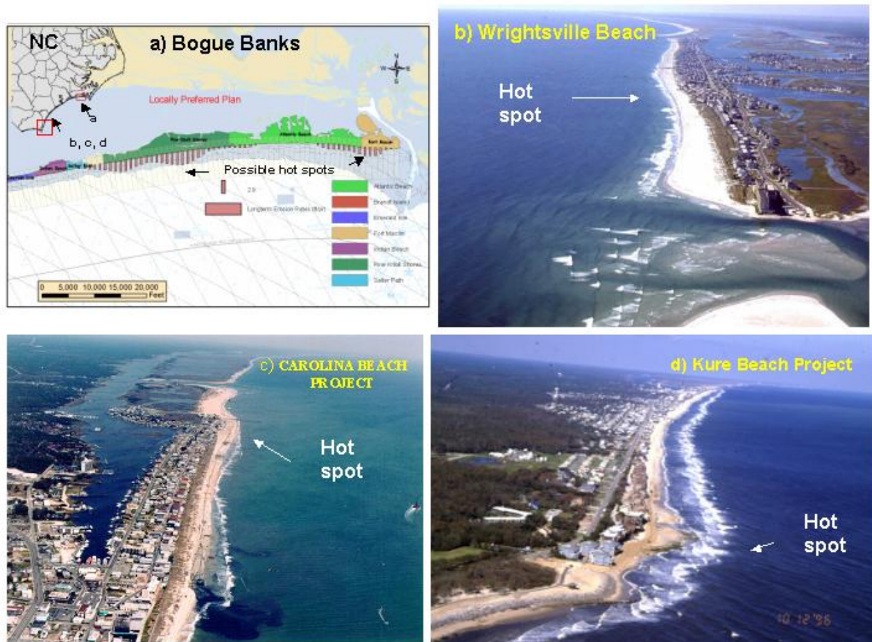
Figure 10. Hot spot location at four projects along the North Carolina coast (a) Bogue Banks at Morehead City near Cape Lookout, NC, (b) Wrightsville Beach, (c) Carolina Beach and (d) Kure Beach just north of Cape Fear, NC (courtesy of John McCormick, Wilmington District)
