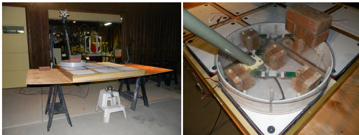
Figure 5: Initial data setup in Grand Junction CO in November, 2011. The MPV2 receivers were used as the Pedemis Rx cabling was incomplete.
