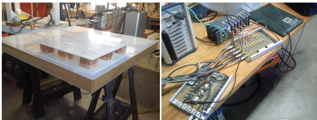
Figure 2: The Pedemis sensor's Tx and Rx arrays (left). The NI cRIO based control system with transmitter and filter boards (right). The Tx and Rx arrays can be detached. This bistatic configuration allows greater positioning accuracy, improved depth detection, deployment in difficult terrain, and flexible exploration of responses in the vicinity of the rig without relocating it.
