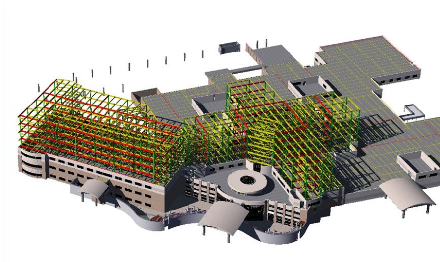
Figure 14. Steel Detailing.
