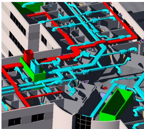
Figure 16. Mechanical BIM.
