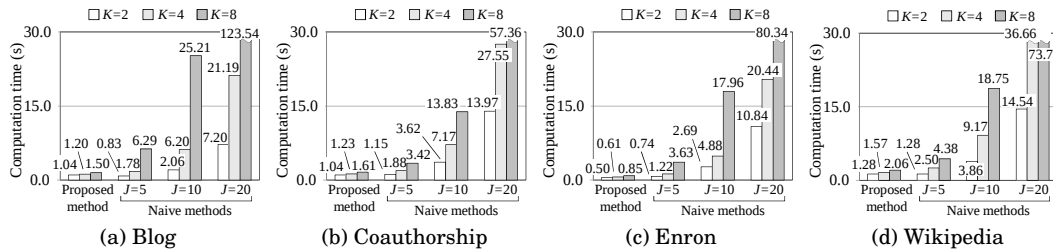
Fig. 12: Comparison of the computation time for the VwV model.
