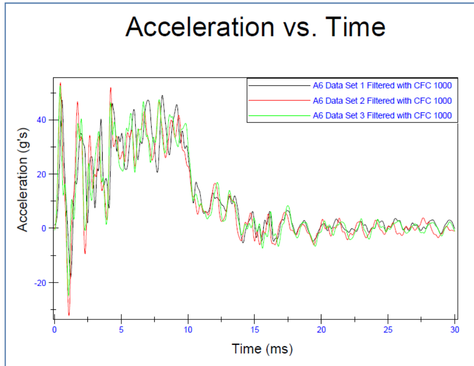
Figure C-15. Material A6 Impulse Graph.
