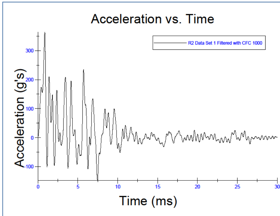
Figure C-1. Material R2 Impulse Graph.
