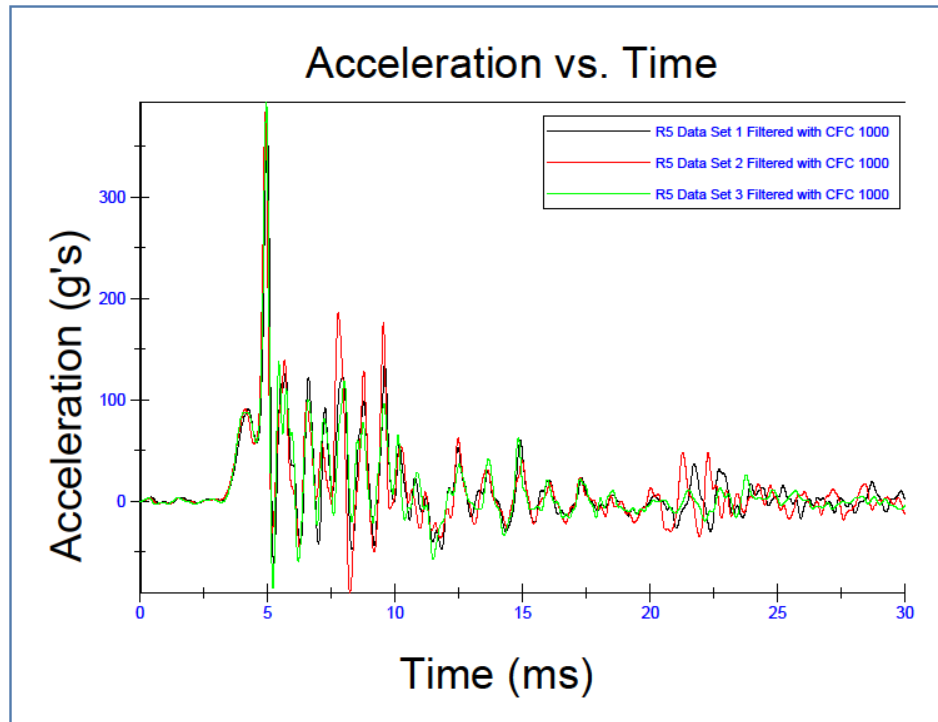
Figure C-3. Material R5 Impulse Graph.
