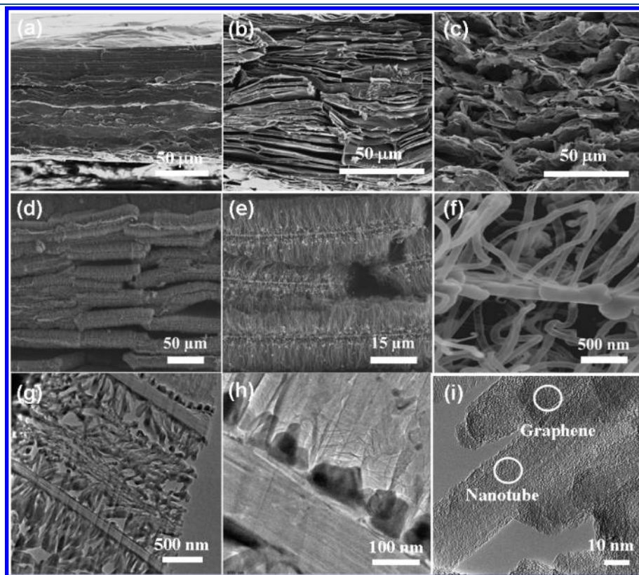
Figure 2. SEM images of (a) the pristine HOPG and the acid-treated, thermally expanded HOPG (b) without and (c) with SiO 2 coating. (d–f) Typical SEM images of the 3D pillared VACNT–graphene architectures under different magnifications. (g–i) Cross-sectional TEM images of the 3D pillared VACNT–graphene architectures under different magnifications.
