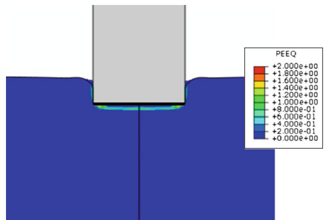
Fig. 5 Finite element calculation of equivalent plastic strain ( \epsilon^{eq} ) in vertically aligned carbon nanotube array material. The material is treated as an open-cell foam-like material
