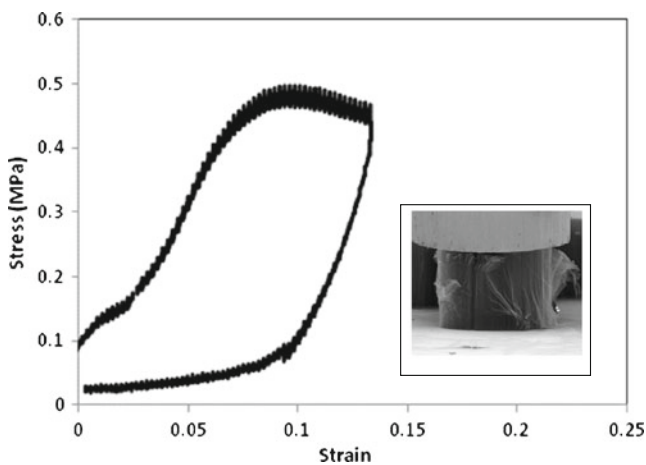
Fig. 3 Compressive stress-strain curve of the vertically aligned carbon nanotube arrays ( t=215 \mu\text{m} )
