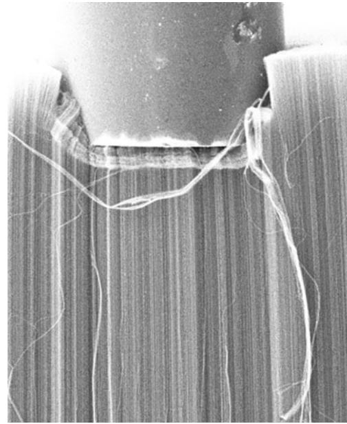
Fig. 4 SEM image showing the development of plastic collapsing of the vertically aligned carbon nanotube arrays under a flat cylindrical indenter ( t=1,100 \mu\text{m} )
