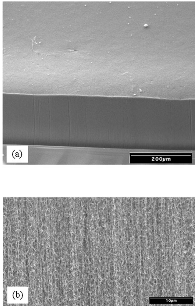
Fig. 1 SEM images showing the morphology of the side surface of the vertically-aligned carbon nanotube arrays ( t=215 \mu\text{m} )
