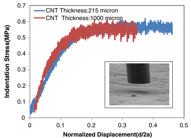
Fig. 2 Indentation stress-displacement curves of vertically aligned carbon nanotube arrays with cylindrical, flat-faced indenter
