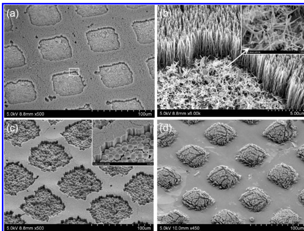
Figure 3. (a) SEM image of ZnO nanorods/VA-MWNTs pattern; (b) An enlarged view of the marked area in panel a; (c) SEM image of SiO 2 microspheres/VA-MWNTs pattern; (d) SEM image of the VA-MWNTs pattern embedded into a TiO 2 thin film.
