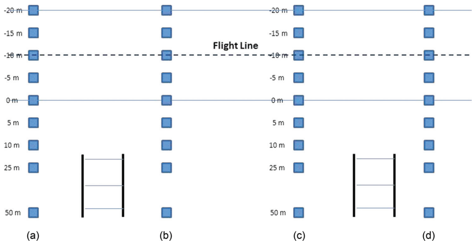
FIG. 1—Field drift study layout.
