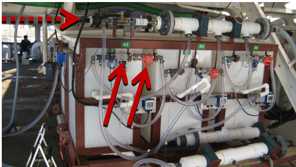
Figure 6. Sampling apparatus used by the Golden Bear Facility to concentrate organisms \geq 50 \mu\text{m} in plankton nets (inside the white tubs; not visible). The dashed, red arrow indicates the inlet to the sampling manifold from the sample port. The solid, red arrows indicate the flow meter (left arrow) and red manual flow control valve (right arrow) used to control sample flow rate to the individual white tubs.
