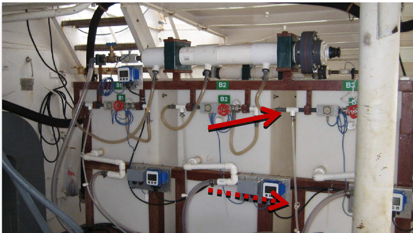
Figure 7. Sample collection tee (marked by the solid, red arrow) used by the Golden Bear Facility to collect organisms < 50 \mu\text{m} ( \geq 10 \mu\text{m} and < 50 \mu\text{m} as well as organisms < 10 \mu\text{m} ). The dashed, red arrow indicates the pinch valve used to control the sample flow.
