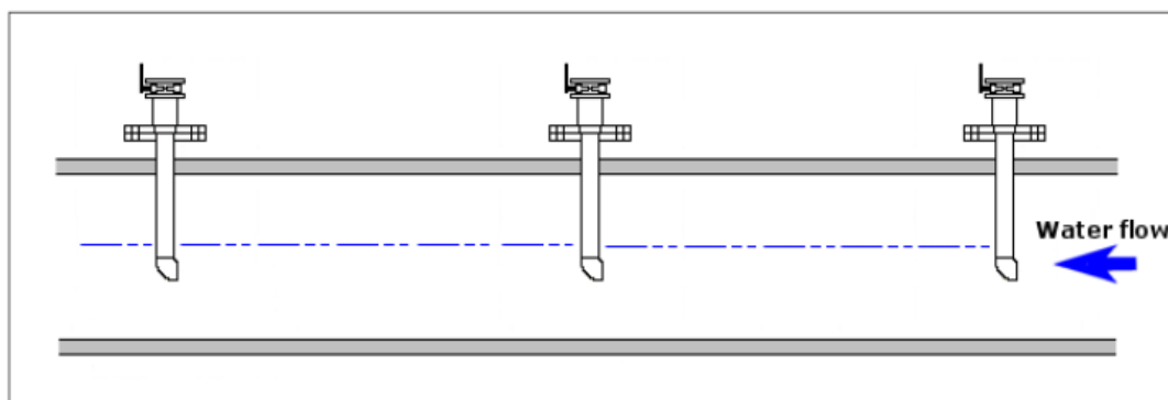
Figure 8. Sample ports used by the Great Ships Initiative to collect organisms \geq 50 \mu\text{m} (Great Ships Initiative, 2012).
