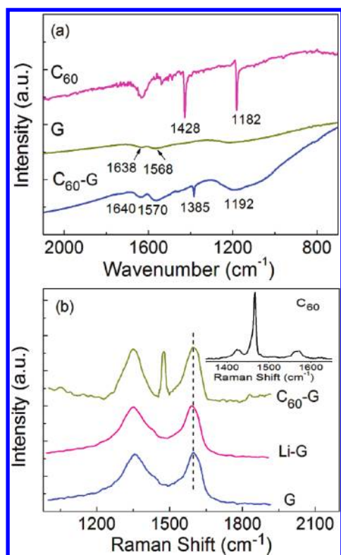
Figure 2. (a) FTIR and (b) Raman spectra of C 60 , the chemically reduced graphene (G), the lithiated graphene (Li-G) prepared under nitrogen protection, and the C 60 -grafted graphene (C 60 -G). All the spectra have been randomly scaled along the y-axes for an easy comparison.
