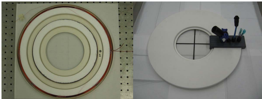
Figure 2. Construction details of the TEMTADS hand-held sensor (left panel) and the assembled sensor (right panel).
