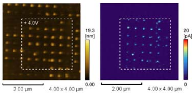
Fig. 2.3 Topographic image of c-AFM (Left) and corresponding current image (Right) scanned at V_{\text{read}} (-1.5 V) after scanned inside the dashed square area with applying at V_{\text{set}} (+4.0 V). The GNP
