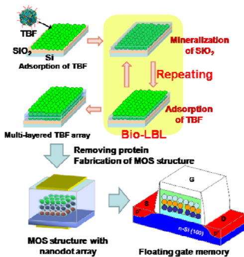
Fig. 1.1 Nanodot-type floating gate memory with multilayered nanodot array formed by Bio-LBL.
