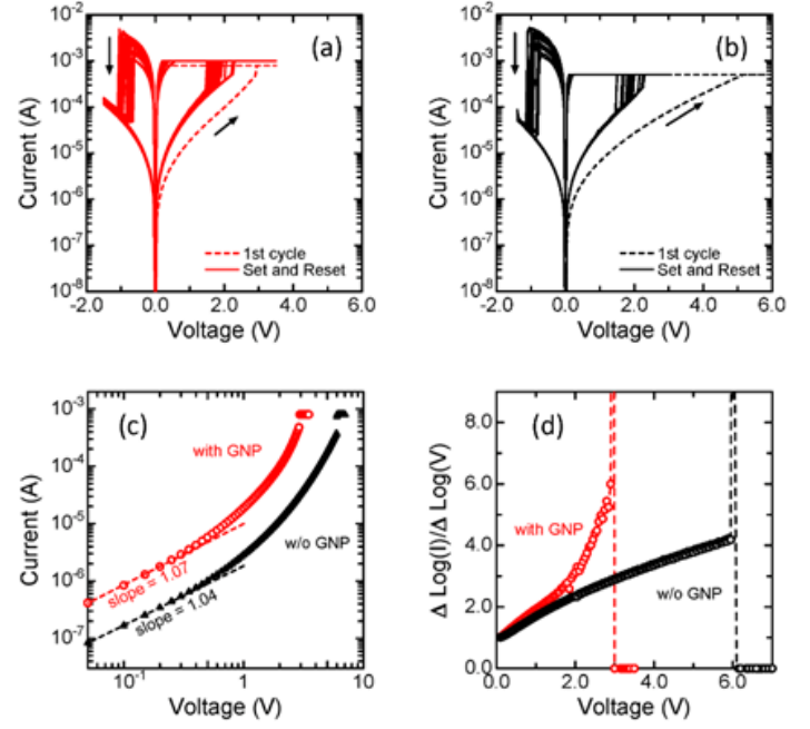
Fig. 2.5 Typical I - V characteristics of (a) the GNP embedded ReRAM and (b) without GNP. (c) The \text{Log}I\text{-Log}V plot at the forming process of NiO resistive memory with and without GNP. (d) The differential resistance d\text{Log}I/d \text{Log}V plot against voltage at the forming process. The curvature of the \text{Log-Log} plot increases differently at the high voltage region.
