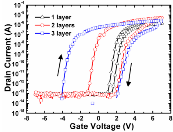
Fig. 1.3. I_D - V_G characteristics.
