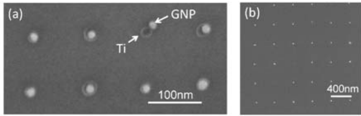
Fig. 2.2 SEM images of controlled placement of the GNP on bottom electrode before NiO deposition. (a) The selectively placed GNPs on Ti nanodisk with 100 nm pitch and (b) 400 nm pitch on n^+ Si substrate.
