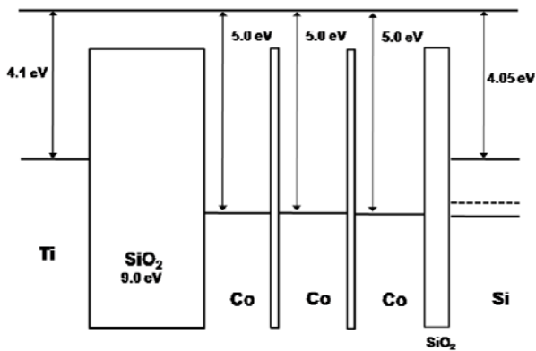
Fig. 1.6. Band structure of memory.
