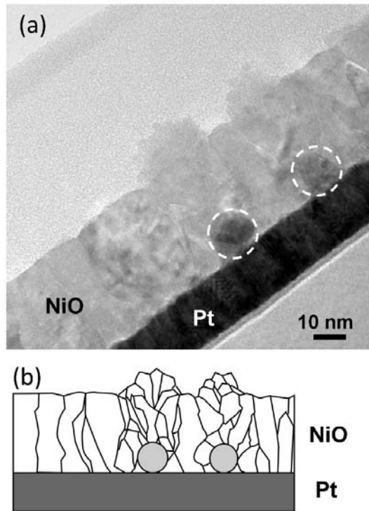
Fig. 2.7 (a) Cross-sectional TEM image of the GNP embedded NiO-GNP/Pt structure before top electrode formation. The thickness of NiO film was 30 nm. (b) Schematic image of cross-section of the device with the
