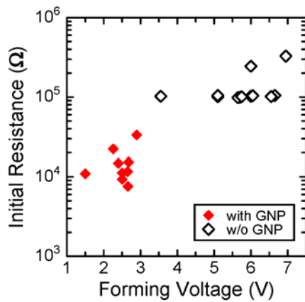
Fig. 2.6 Relation between the forming voltage and the initial resistance with and without GNPs. The forming voltage was reduced and the initial resistance also was decreased by the GNP.
