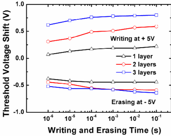
Fig. 1.4. Writing and erasing characteristics.
