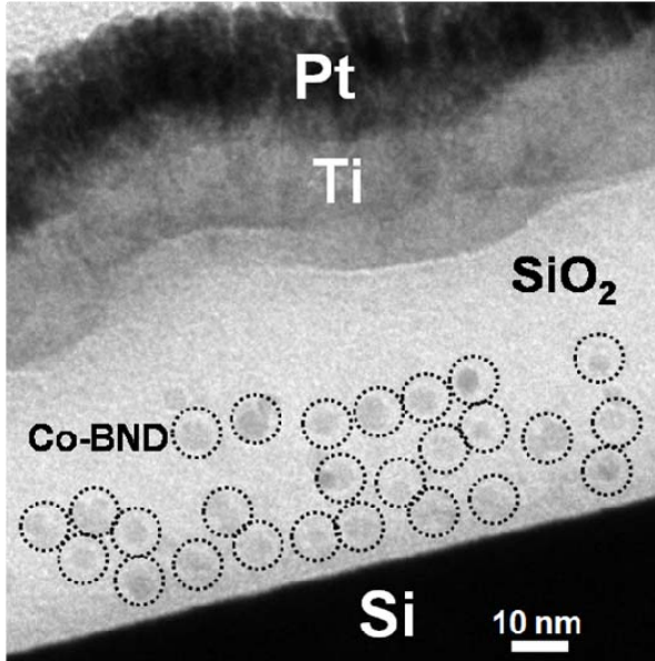
Fig. 1.2 Cross-sectional TEM image of memory.
