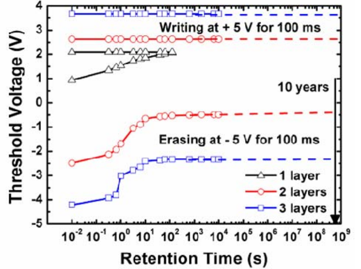
Fig. 1.5. Retention characteristic.
