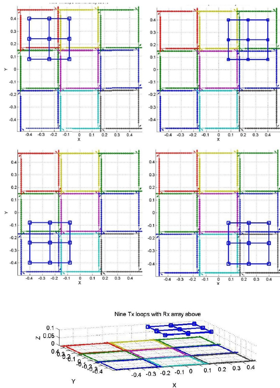
Figure 3.11: Pedemis beacon example with Rx array above the Tx array.
