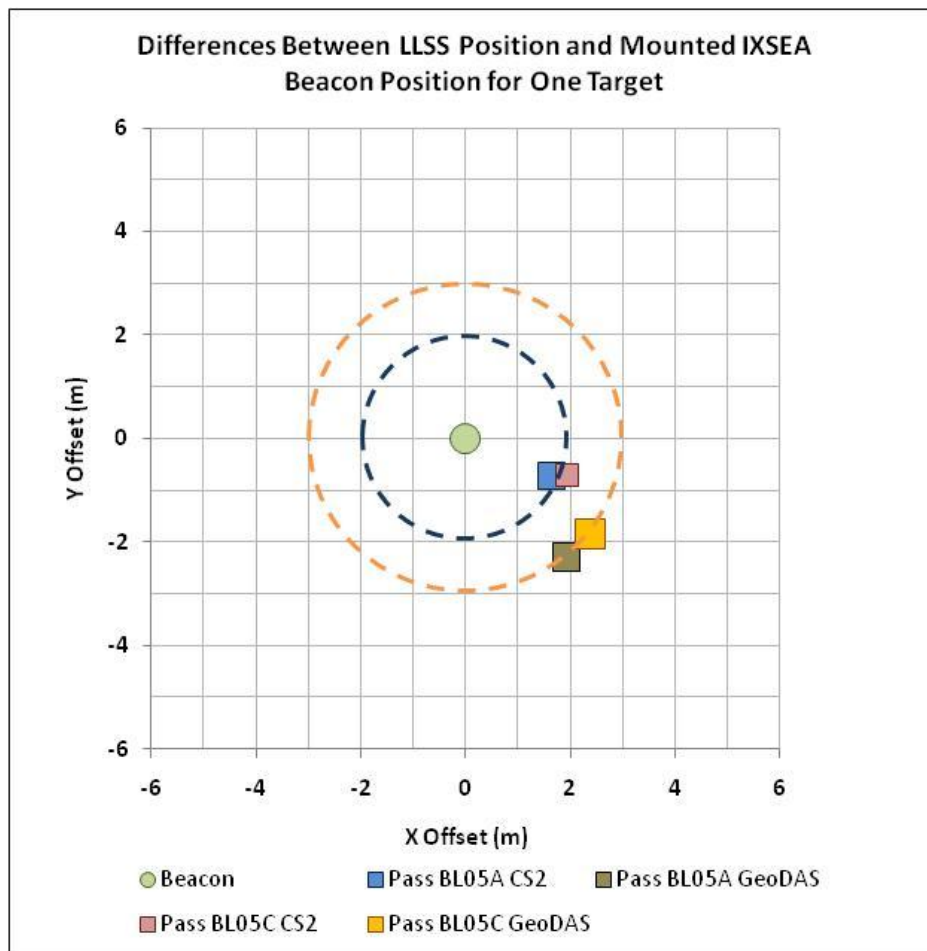
Figure 13. Corrected LLSS positions for one target on Year 2 Validation Line 3 as determined over multiple passes with both CleanSweep2 and GeoDAS software relative to the true position as determined with an IXSEA beacon.
