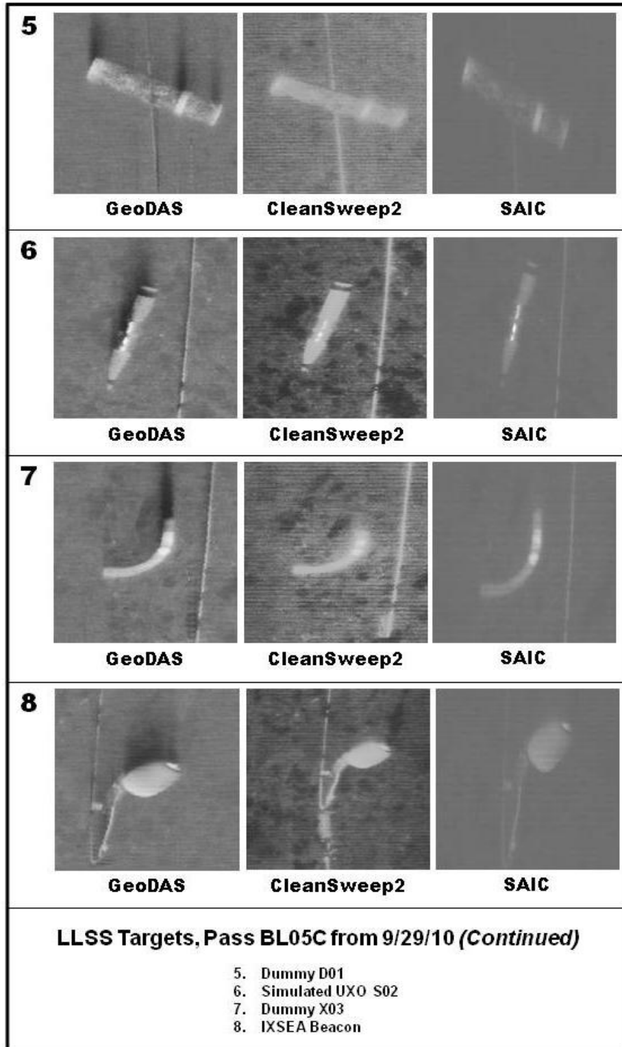
Figure 9. Comparison of the raw GeoDAS images and the post-processed CleanSweep2 and SAIC software images for all targets identified in Pass BL05C from Year 2 (continued).
