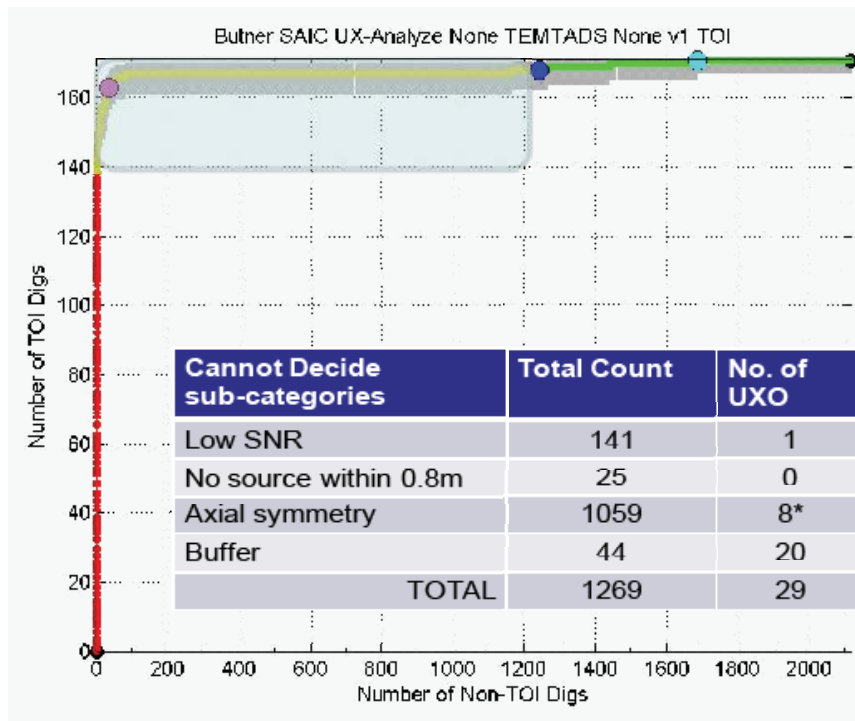
Figure 6-72. ROC curve of UX-Analyze TEMTADS analysis and associated Cannot Decide subcategories.
