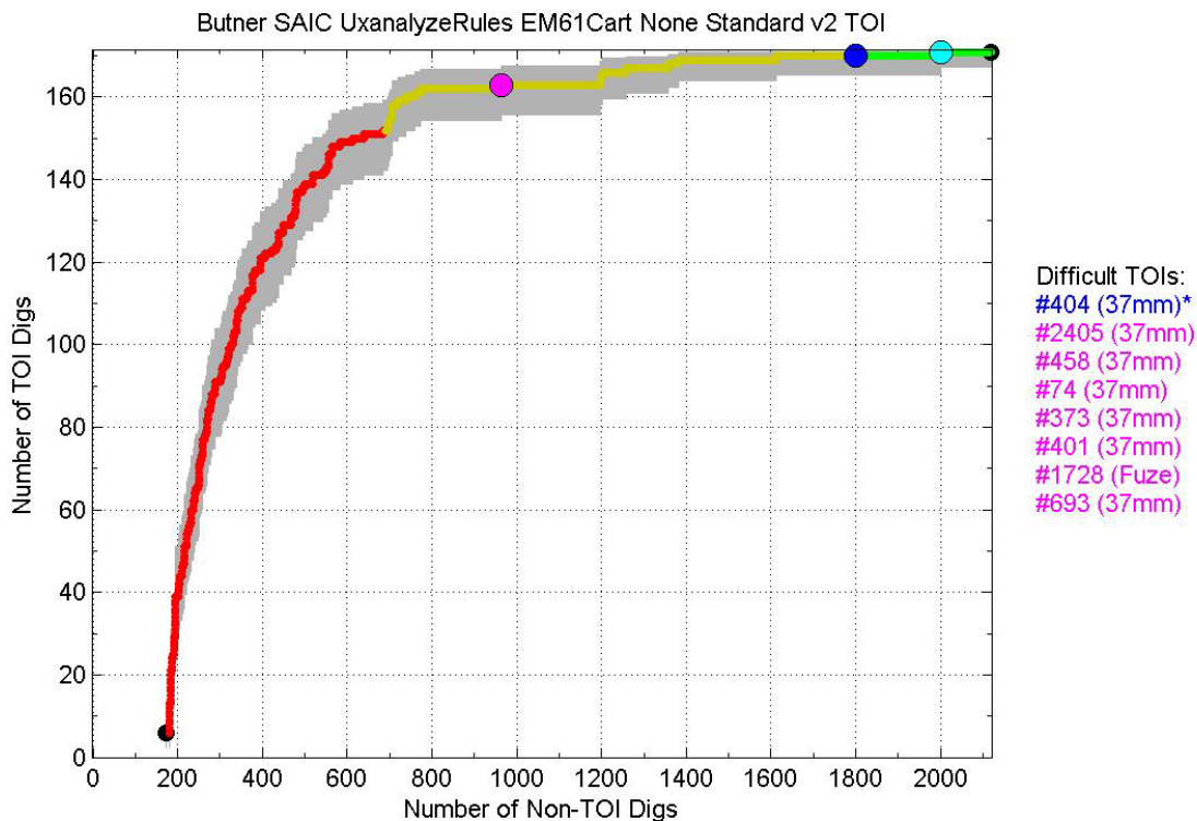
Figure 6-16. SAIC's EM61 MK2 Cart ROC chart.
