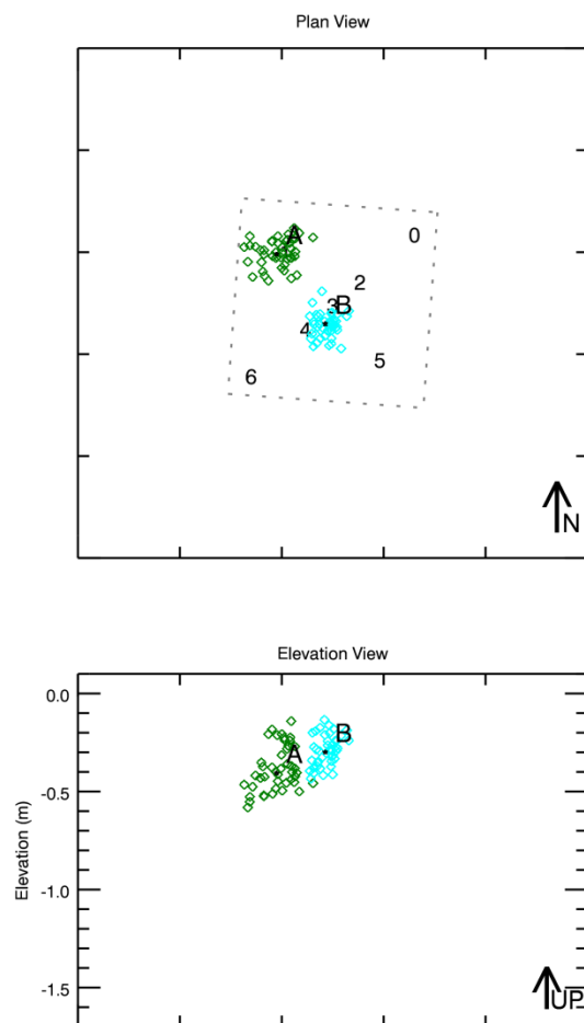
Figure 6-54. Fit results plot of Geometrics' MM anomaly 1346 after removing Rx3Y and adjusting the multi-dipole solver parameters.
