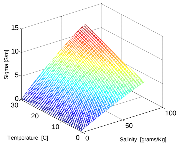
Figure 3-32: Seawater conductivity versus salinity and temperature.
