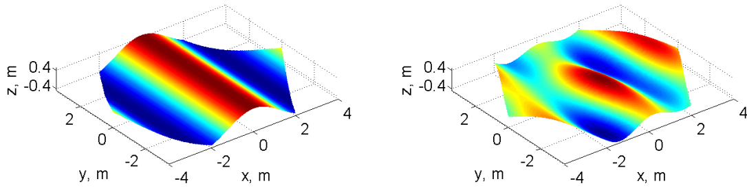
Figure 2-9: Simulated water surface in different cases.
