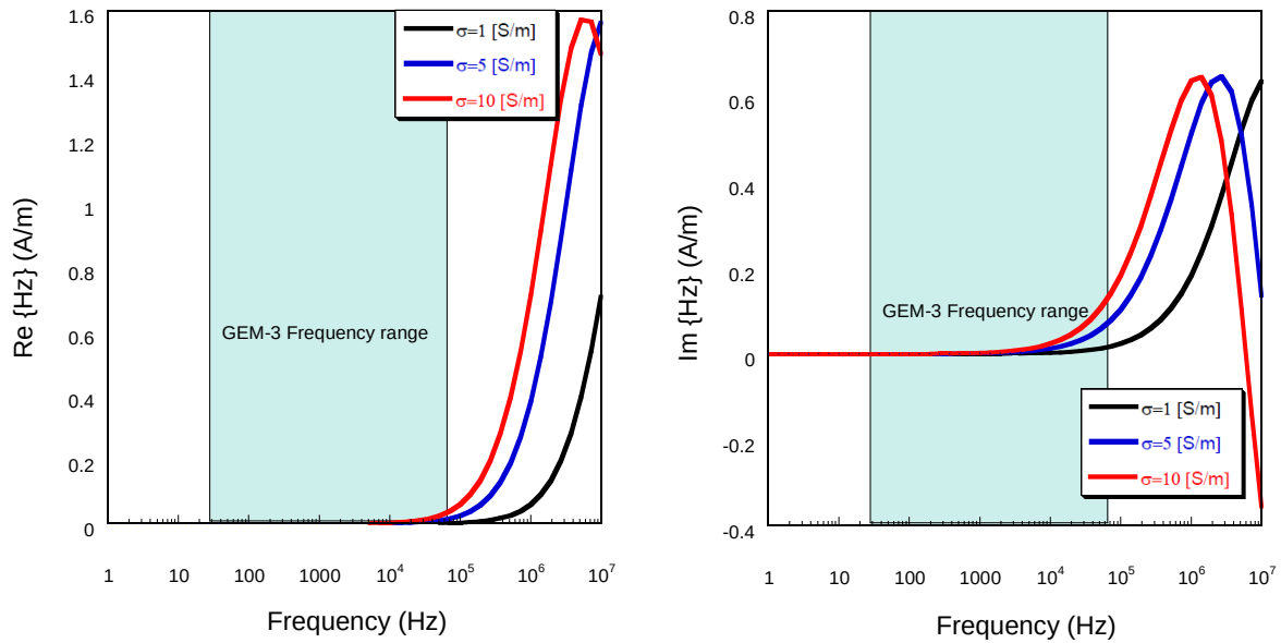
Figure 3-8: Scattered magnetic field versus frequency: (Left) Inphase part; (Right) Quadrature part.
