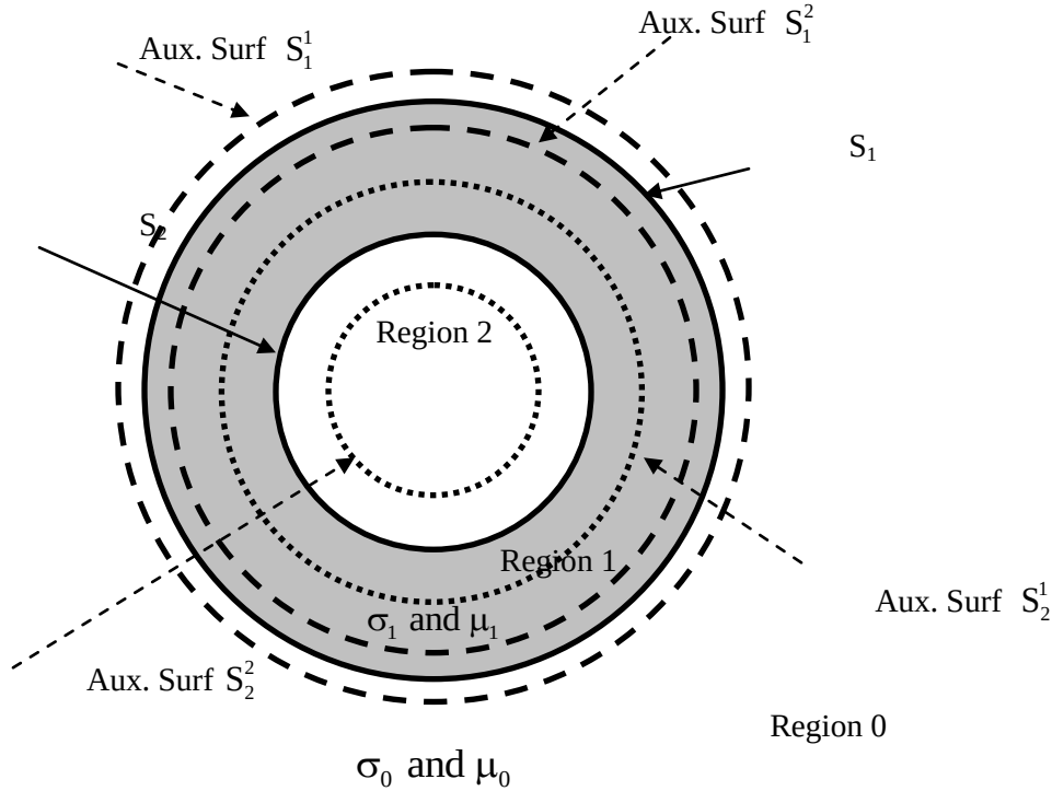
Figure 2-3: MAS diagram for a layered scattering object.
