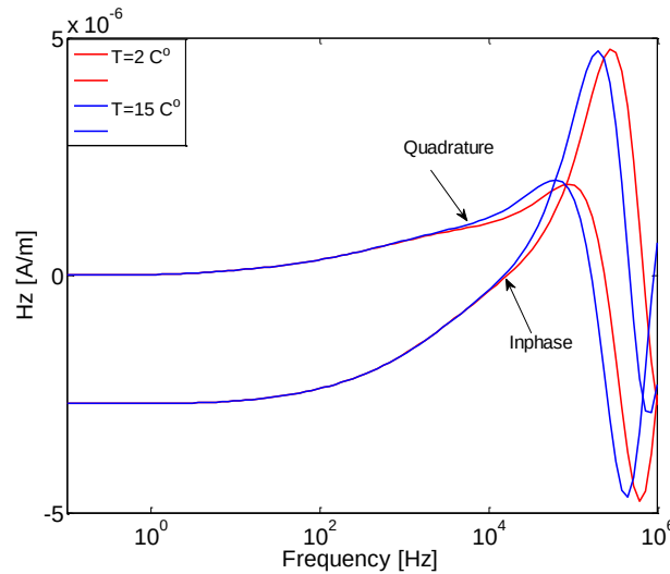
Figure 3-33: EMI response for a spheroid at temperatures T_1 = 2^\circ\text{C} (red curves) and T_1 = 15^\circ\text{C} (blue curves) in seawater of salinity S = 35 g/kg. Both inphase and quadrature parts are shown.
