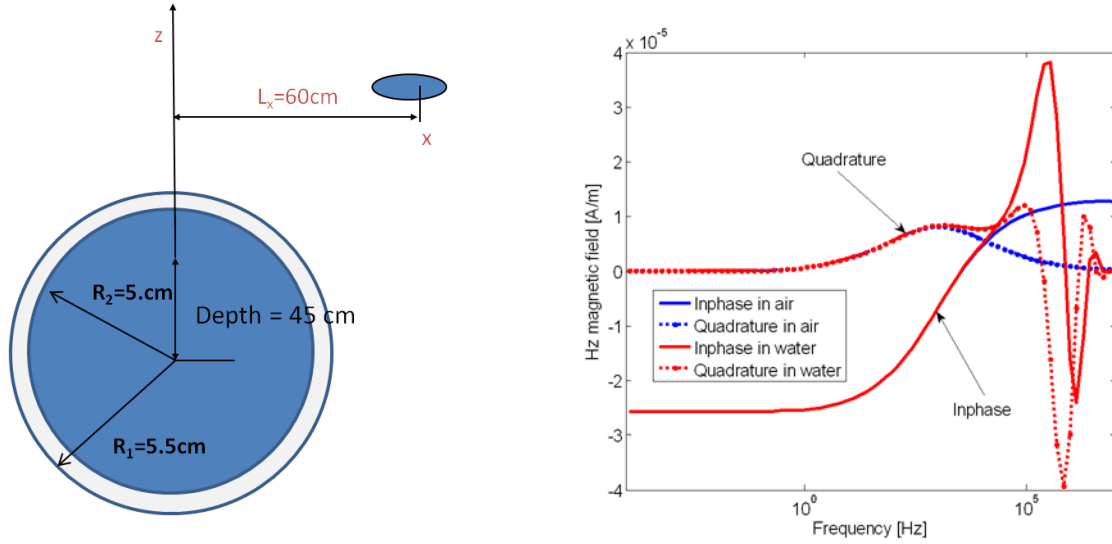
Figure 3-25: Studying the interaction between a conducting object and the surrounding conductive medium. (A) Geometry of the system; (B) Magnetic field measured by the sensor as a function of source frequency and the surrounding medium, for a solid conducting sphere with the radius R_2 = 5 cm.
