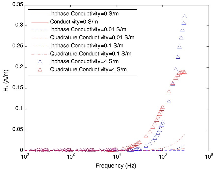
Figure 3-4: Scattered magnetic field vs. frequency for a conducting half-space illuminated by an EMI sensor.
