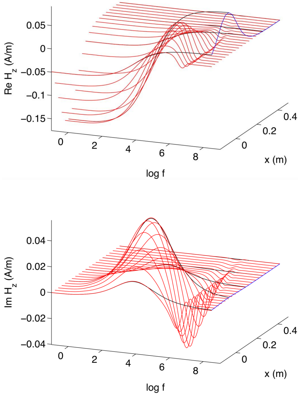
Figure 4-12: Inphase (top) and quadrature (bottom) parts of the secondary field, measured over a transect, of a ferromagnetic sphere of radius a = 5 cm under dipolar excitation and embedded in a medium of conductivity \sigma_2 = 4 S/m.
