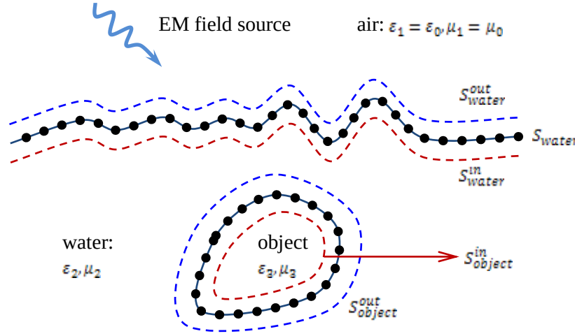
Figure 2-2: The MAS applied to the underwater detection problem.
