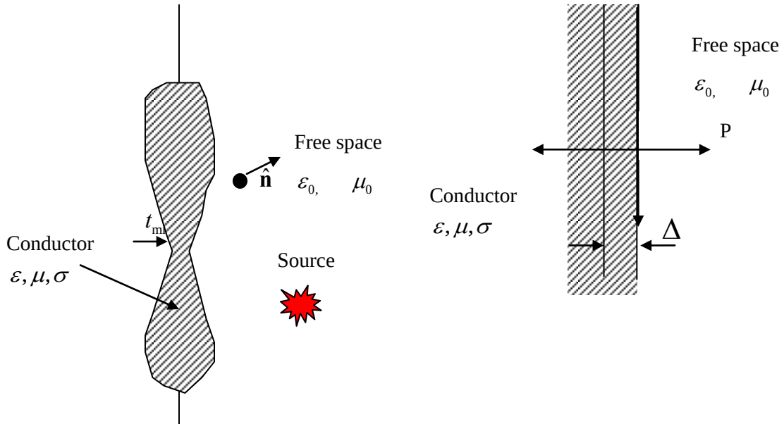
Figure 2-6: Skin effect
