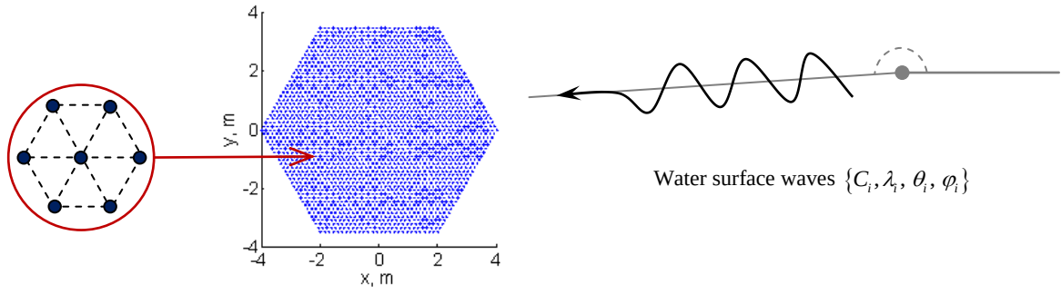
Figure 2-8: Initial flat water surface with uniformly distributed collocation points and a sample surface perturbation.
