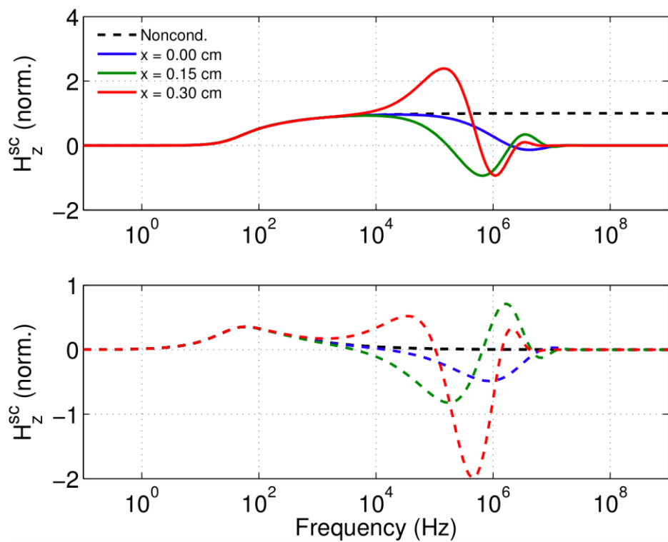
Figure 4-6: Three of the profiles of Figure 8-28 but seen from the side and normalized by the high-frequency limit of the profile in the nonconducting me-dium. The profile does not just diminish spatially; it also changes with transverse distance in a rather non-intuitive way.
