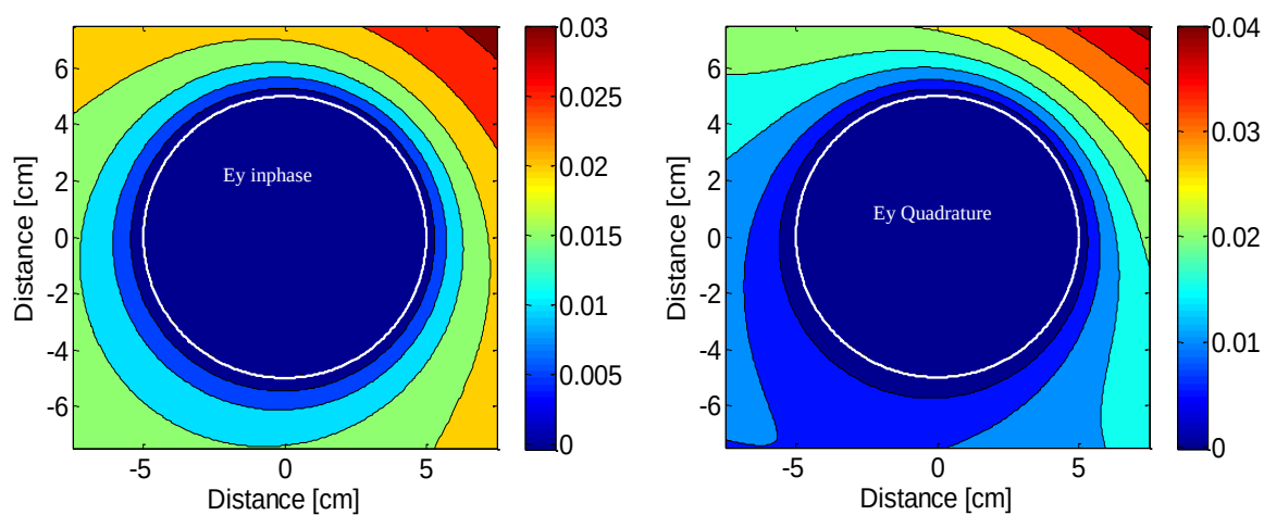
Figure 3-28: Electric field distribution inside and outside of a solid sphere.
