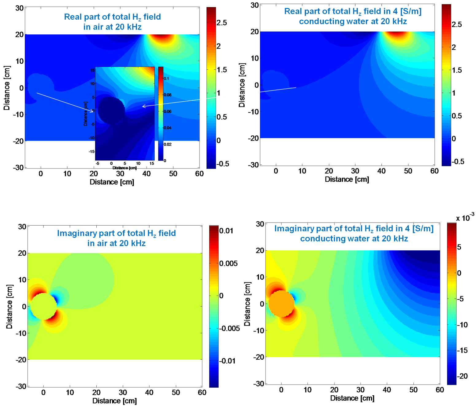
Figure 3-19: Total H_z magnetic field distributions inside and outside a sphere of radius 5 cm placed in air (left column) and in conducting water (right column).
