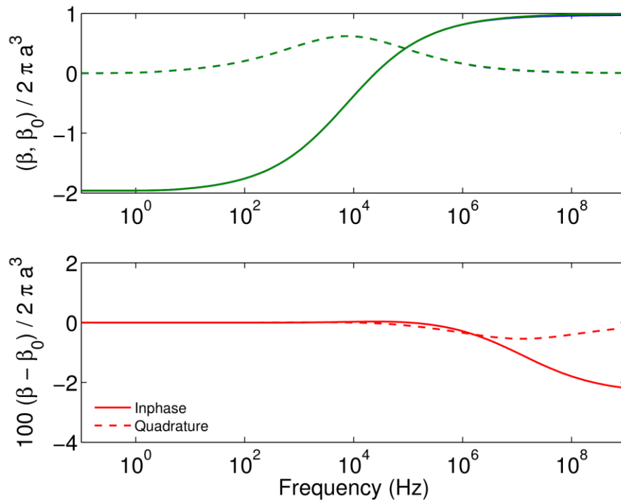
Figure 4-2: The polarizability of the sphere is affected when the surrounding medium has finite conductivity, but not by much.
