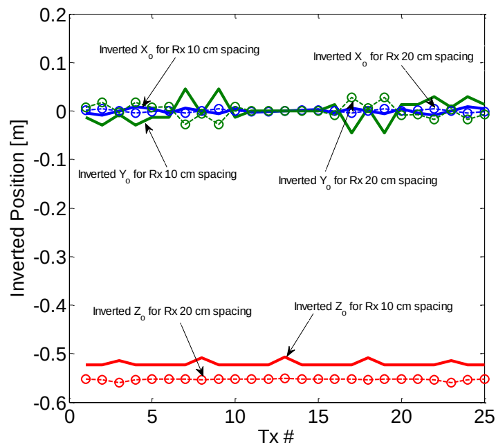
Figure 3-38: Inverted positions for different transmitters.
