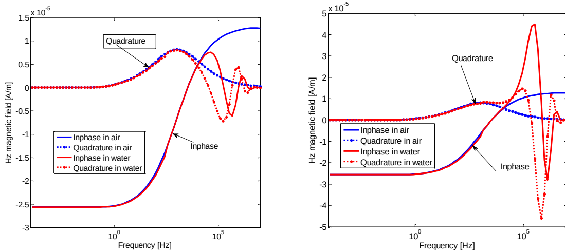
Figure 3-26: (A) Magnetic field in sensor as a function of source frequency and the surrounding medium, for a solid conducting sphere ( R_2 = 5 cm) surrounded by a thin insulating shell (total radius R_1 = 5.5 cm); (B) Magnetic field in sensor as a function of source frequency and the surrounding medium, for a solid conducting sphere ( R_2 = 5 cm) surrounded by a thin conducting shell (total radius R_1 = 5.5 cm).
