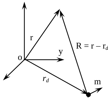
Figure 2-7: Geometry of the problem. The target is assumed to be a magnetic dipole located at \mathbf{r}_d .
