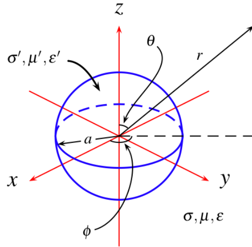
Figure 4-1: Problem geometry for a sphere embedded in a conducting medium.
