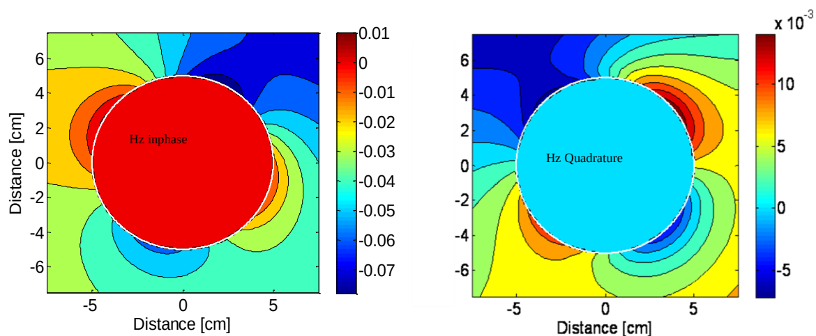
Figure 3-29: Magnetic field distribution inside and outside an insulated sphere (inphase at left, quadrature at right).
