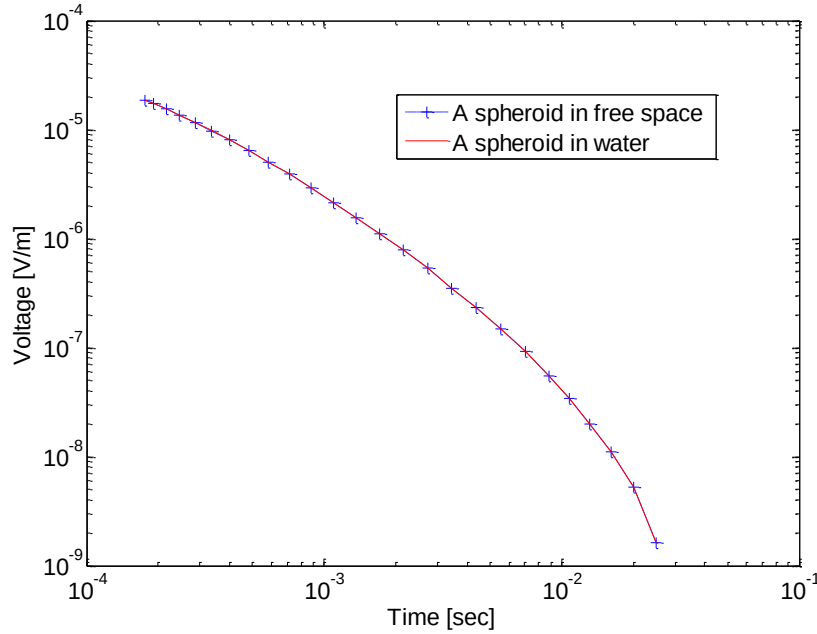
Figure 3-11: Time-domain EMI response of a prolate spheroid with conductivity 4 \times 10^6 S/m and permeability 100, illuminated with the EM-63 sensor placed at location L_y = 75 cm.
