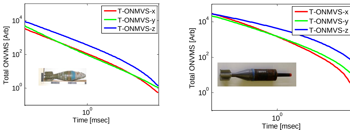
Figure 3-40: Inverted total ONVMS for a multi-target synthetic TEMTADS data set that includes a 60-mm mortar (left) and a 105-mm HEAT round (right).
