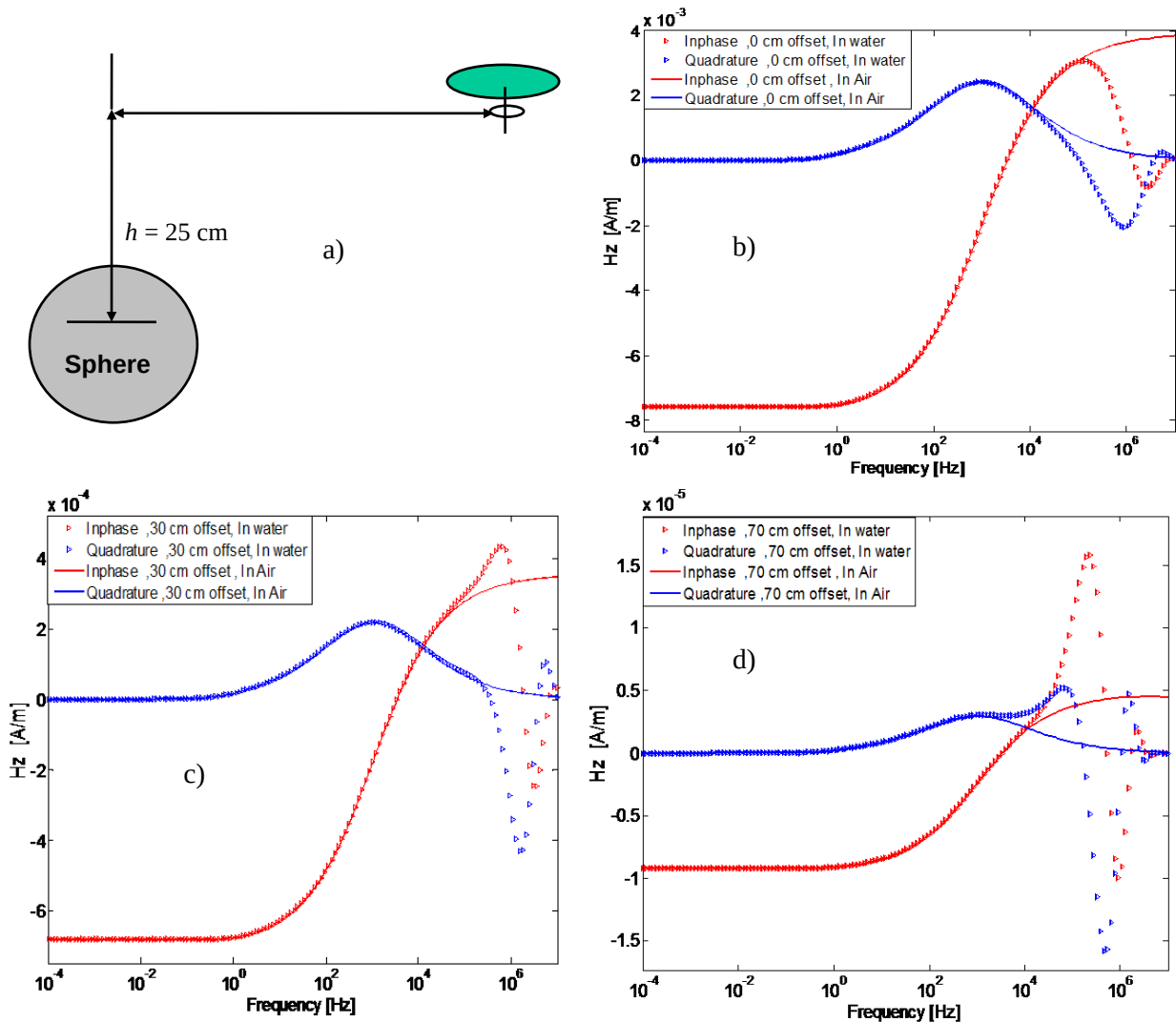
Figure 3-9: Scattering from a highly conducting and permeable sphere. b, c, d) EMI responses of the sphere illuminated by the GEM-3 sensor placed at different locations: L = 0, 30 and 70\text{ cm} .
