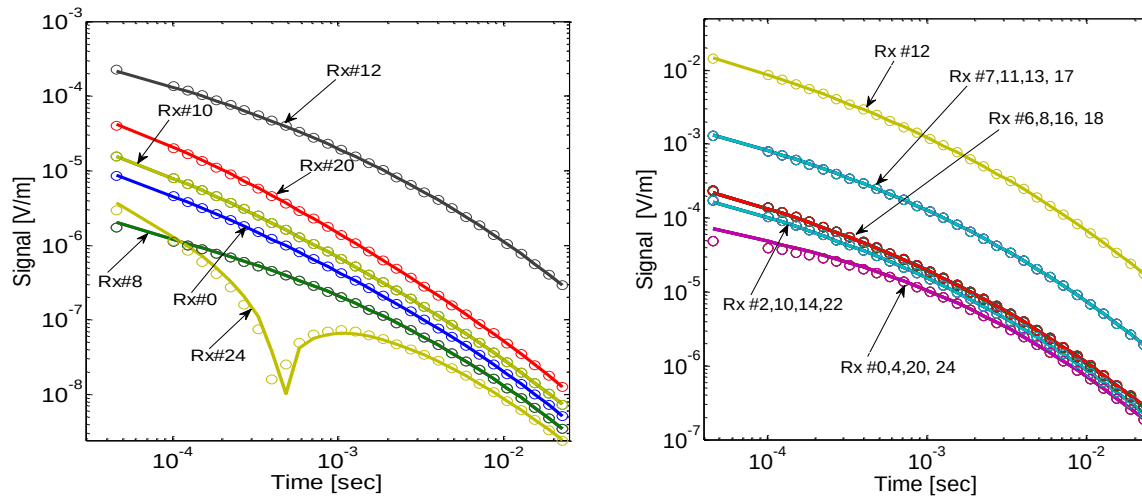
Figure 3-36: Spheroid oriented vertically and placed 45 cm below the center of the TEMTADS system in air (circles) and in conductive water with \sigma = 4 S/m (solid lines).
