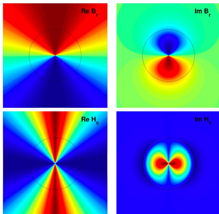
Figure 4-8: That the relevant boundary conditions are obeyed at the sphere surface is not surprising, since they are enforced explicitly in the analytic treatment.
