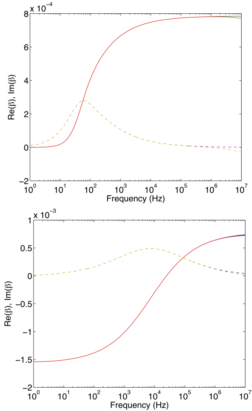
Figure 4-13: Real (solid) and imaginary (dashed) parts of the polarizability element \beta for a 5-cm-radius sphere in vacuum (blue and cyan), in a conducting medium (green and magenta), and in a conducting medium but surrounded by a relatively thin layer of vacuum (5 mm in this case, shown in red and yellow).
