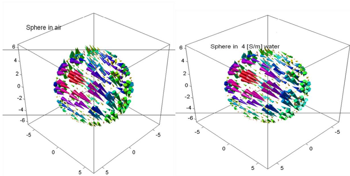
Figure 3-16: Induced eddy-current distributions inside and outside a sphere placed in air (Left) and within a 4-S/m conducting space (Right).
