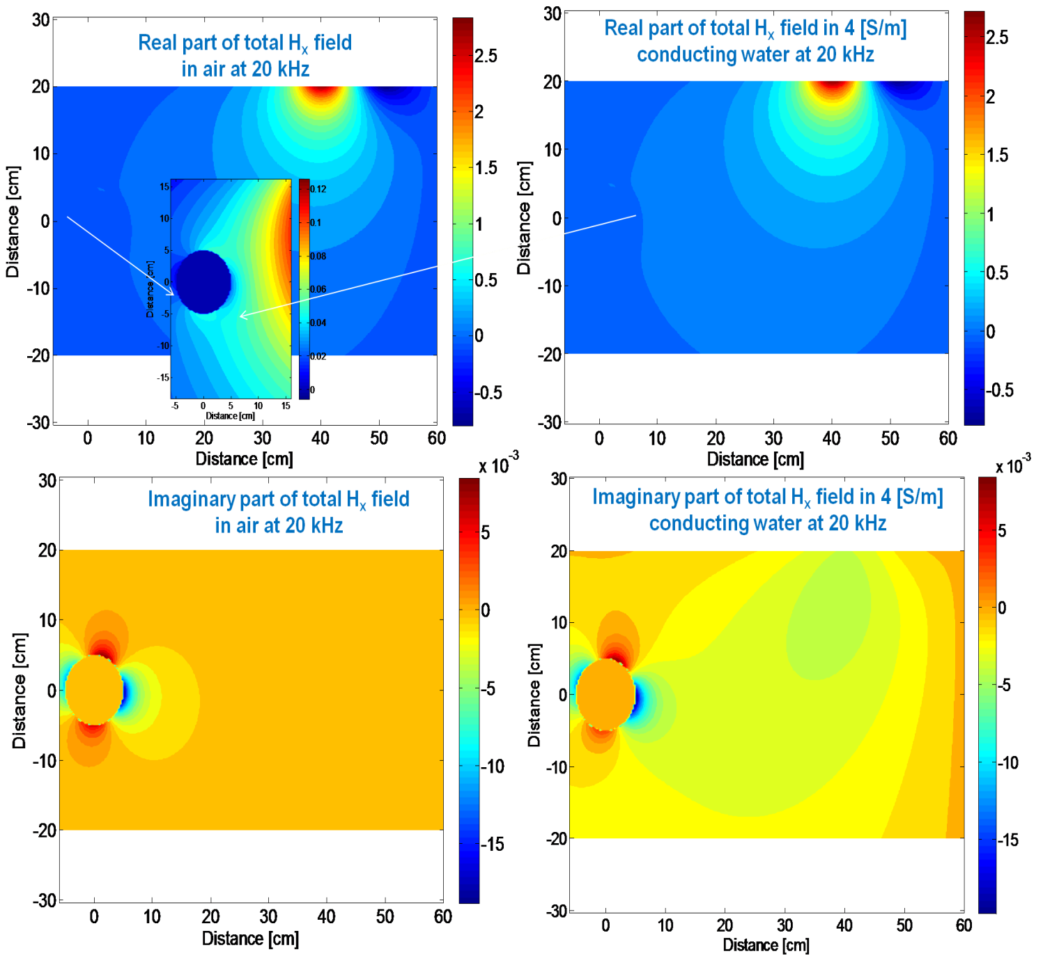
Figure 3-18: Total H_x magnetic field distributions inside and outside a sphere of radius 5 cm placed in air (left column) and in conducting water (right column).
