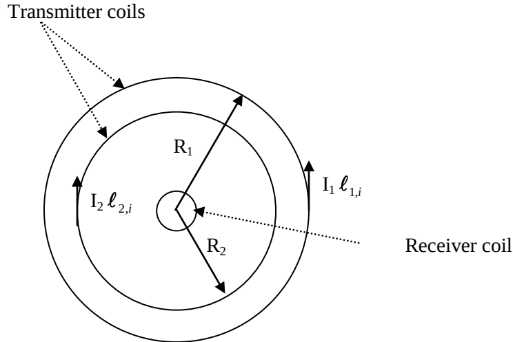
Figure 2-5: Loop geometry of antenna.
