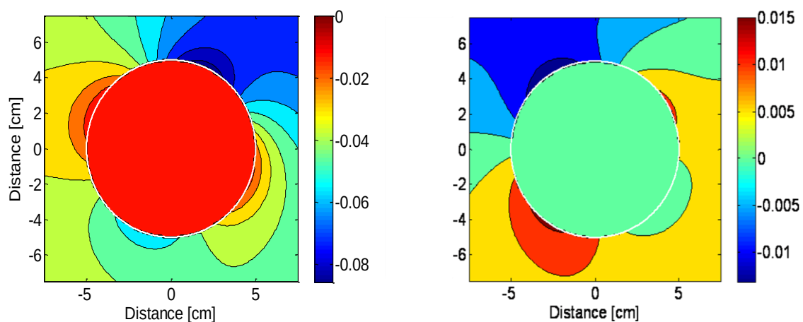
Figure 3-30: Magnetic field distribution inside and outside a solid sphere (inphase at left, quadrature at right).
