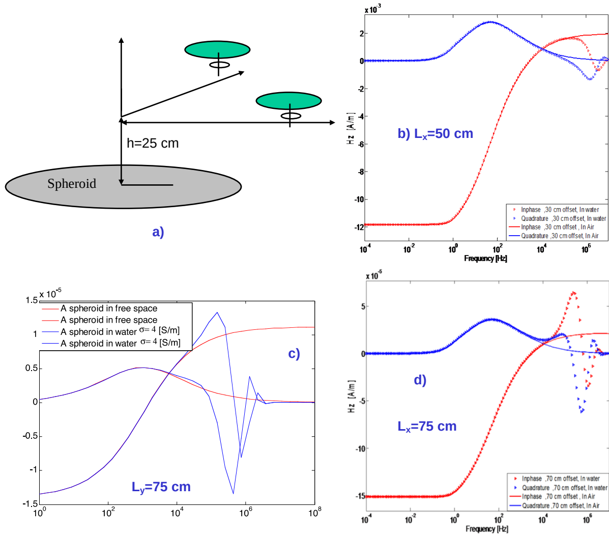
Figure 3-10: EMI response of a prolate spheroid with conductivity 4 \times 10^6 S/m and permeability \mu_r = 100 illuminated with the GEM-3 sensor when placed at three locations: b) ( L_x = 50 cm, L_y = 0 ), d) ( L_x = 75 cm, L_y = 0 ), c) ( L_x = 0 , L_y = 75 cm).
