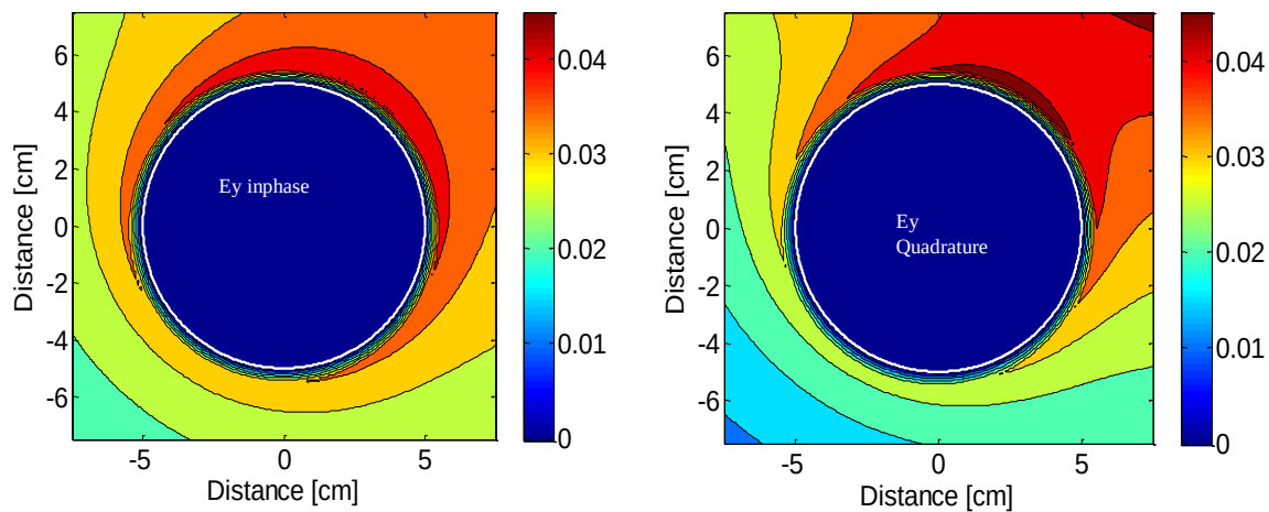
Figure 3-27: Electric field distribution inside and outside of an insulated sphere.
