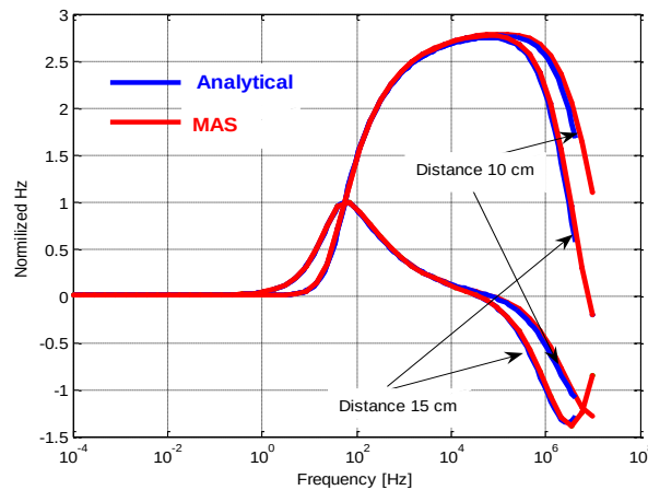
Figure 3-1: Normalized scattered magnetic field versus frequency for a sphere.
