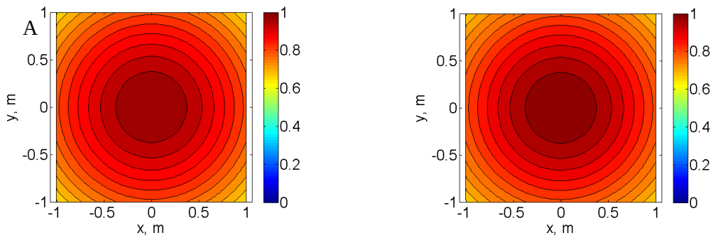
Figure 3-23 H-field distribution at depth 2 m below the (A) unperturbed water surface; (B) surface perturbed by multiple waves (Figure 2-8). Fields normalized to their maximal value in the unperturbed case.
