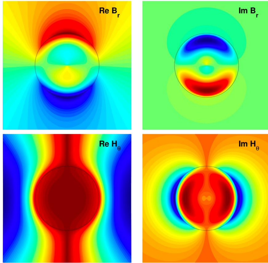
Figure 4-10: Same as the previous figure, but for a permeable sphere with \mu_r' = 1 and \sigma' = 5 \times 10^4 S/m. To obtain a clearer figure we have set the conductivity of the sphere to a low value. The medium has \sigma = 4 S/m and f = 500 Hz.
