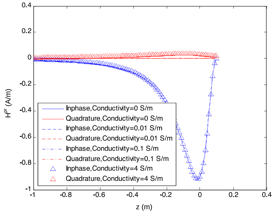
Figure 3-6: Primary magnetic field inside the conducting half-space along the line right below the sensor center for different half-space conductivities. The frequency is 100 kHz.
