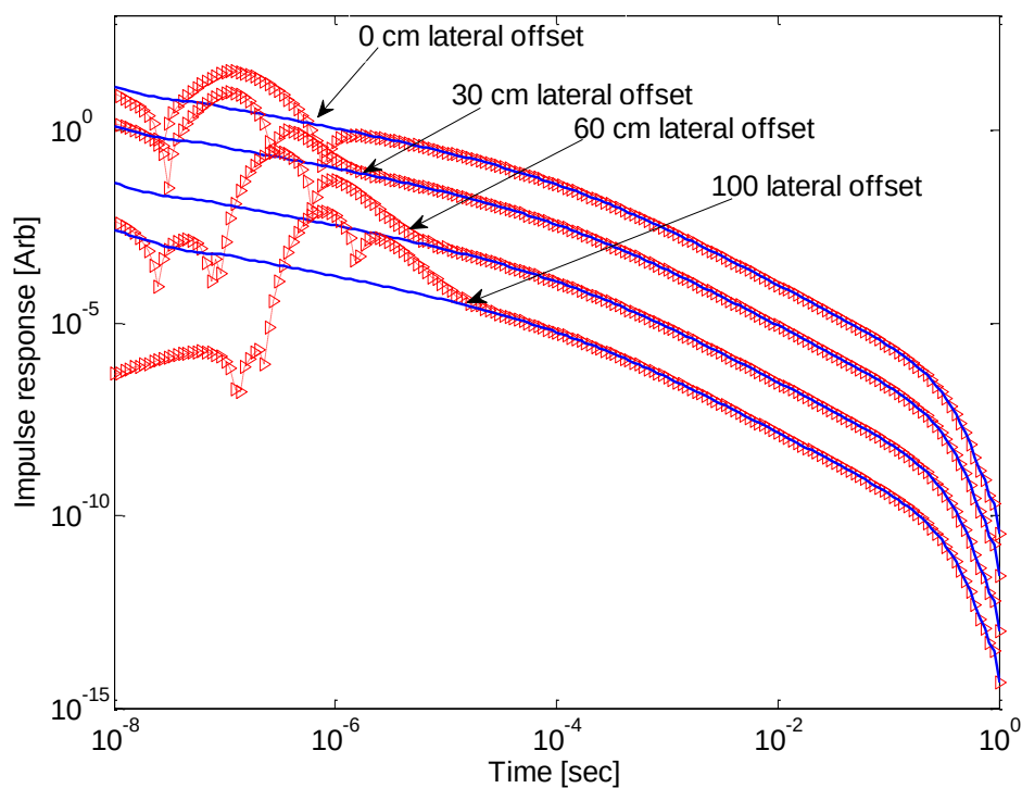
Figure 3-12: Impulse EMI response of a sphere with conductivity 4 \times 10^6 S/m and relative permeability 100, illuminated with the EM-63 time-domain sensor placed at different locations. Blue lines: the sphere is located in the free space; red dot/triangular lines: the sphere is placed in 4 S/m conducting space.
