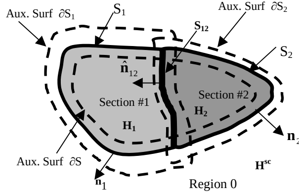
Figure 2-4: MAS diagram for a heterogeneous object.
