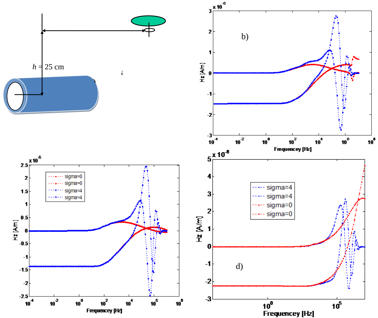
Figure 3-15: Scattering from a highly conducting and permeable pipe with 5 cm inner diameter and 5.7 cm length. The pipe is illuminated by the GEM-3D sensor placed at L_x=75 cm. Pipe thicknesses are b) 10 mm, c) 5 mm, and d) 1 mm.
