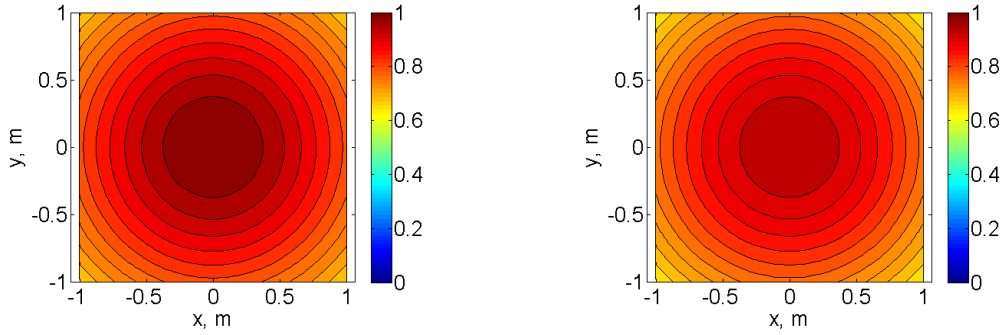
Figure 3-21 H-field distribution at depth 2 m below the (A) unperturbed water surface; (B) surface perturbed by a single cosine wave with wavelength of 5 m and height of 1 m. Fields normalized to their maximal value in the unperturbed case.
