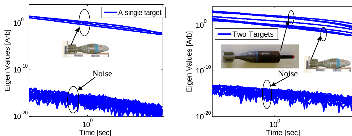
Figure 3-39 Joint-diagonalization eigenvalues vs. time for synthetic TEMTADS data sets with one target (60-mm mortar, left) and two (105-mm HEAT round and 60-mm mortar, right).
