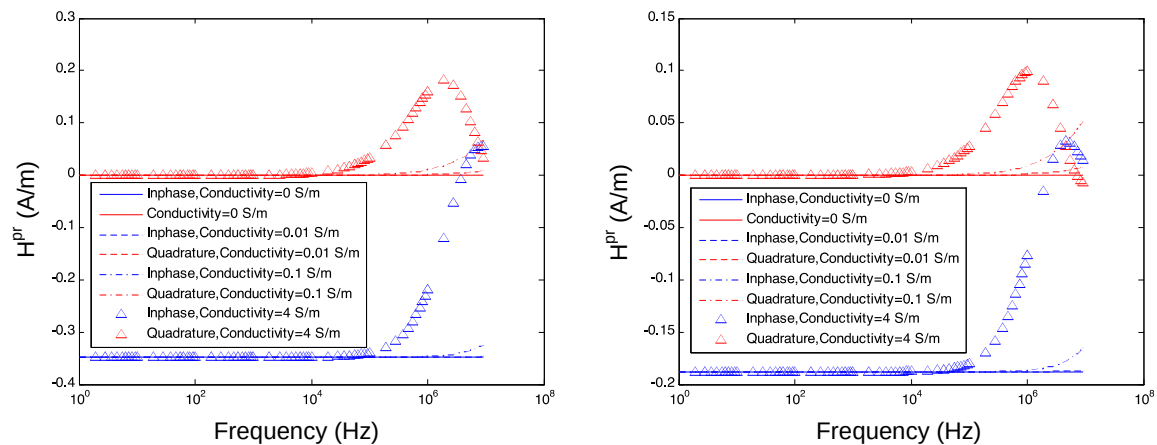
Figure 3-5: Transmitted primary magnetic field versus frequency inside the half-space for the EMI sensor at the two observation points of Figure 3-3.
