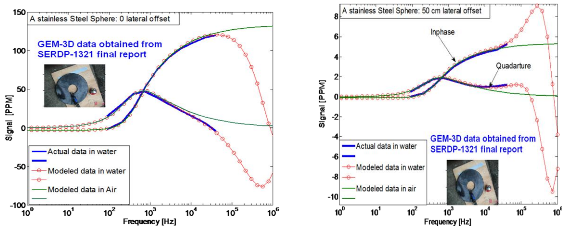
Figure 3-2: MAS/SIBC results and actual data for a sphere with the sensor at (a) zero and (b) 50-cm lateral offsets.
