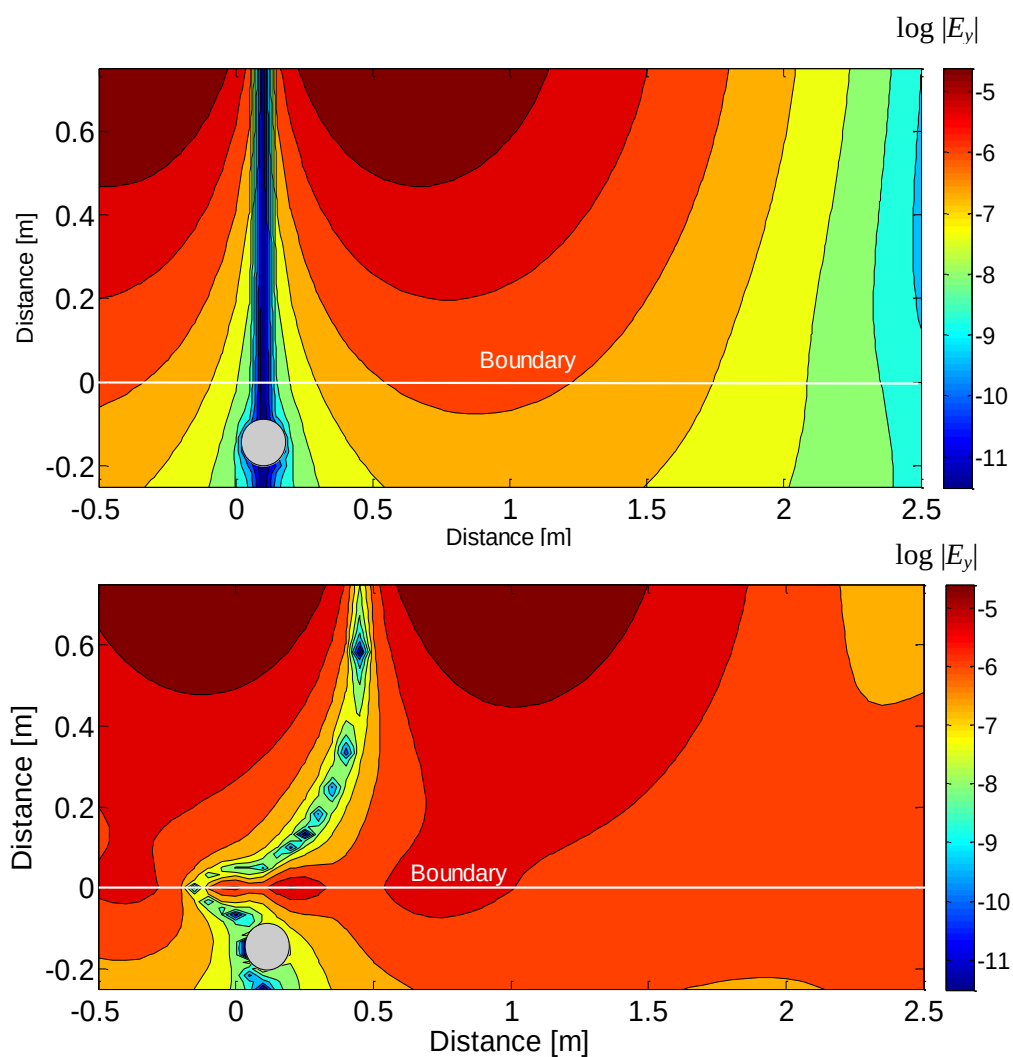
Figure 3-35: Electric field distribution for a sphere placed in a two-layer medium: a) zero lateral offset, b) 30-cm offset.
