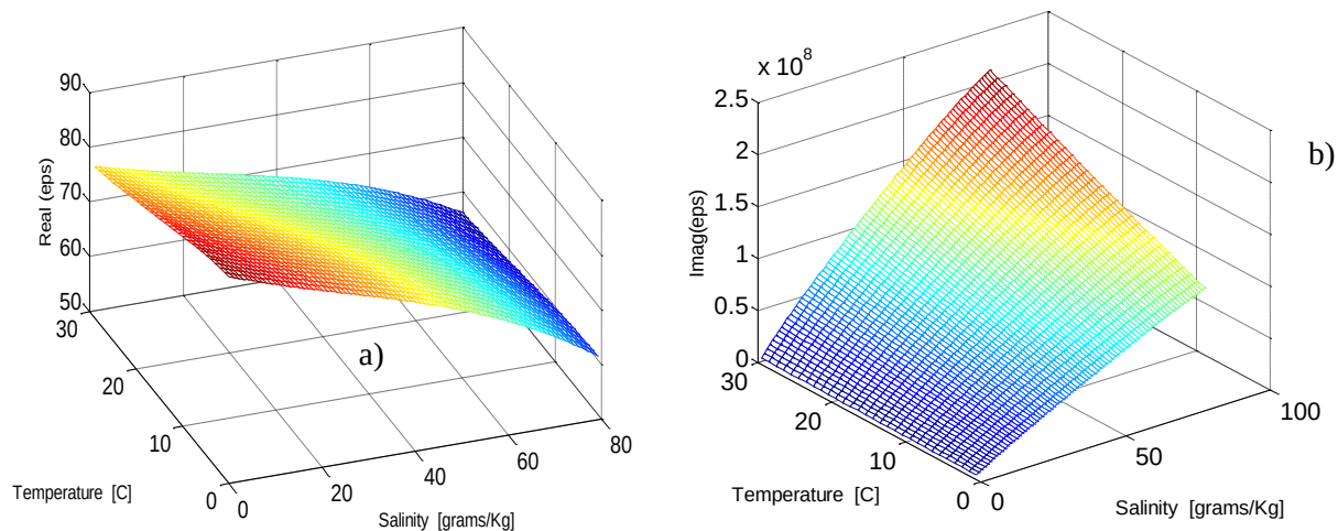
Figure 3-31: Seawater permittivity versus salinity and temperature: (a) Real and (b) Imaginary parts.
