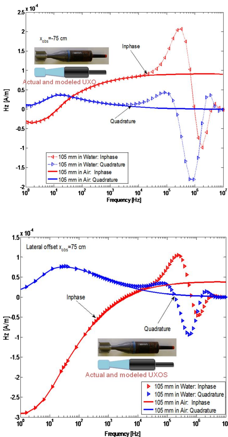
Figure 3-14: EMI response for a 105-mm UXO.
