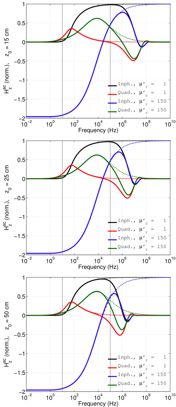
Figure 4-3: Secondary field produced by a sphere subjected to uniform excitation.
