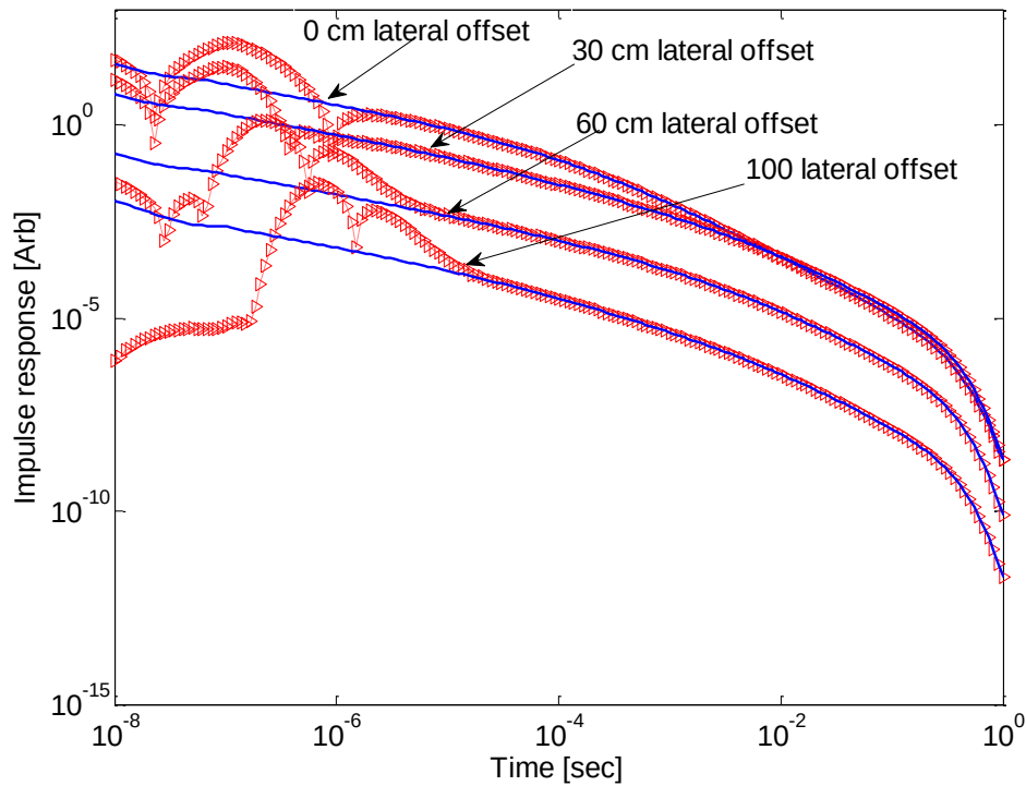
Figure 3-13: Impulse EMI response of a prolate spheroid with conductivity 4 \times 10^6 S/m and permeability 100, illuminated with the EM-63 time-domain sensor placed at different locations. Blue lines: the spheroid is located in the free space; red dot/triangular lines: the spheroid is placed in 4 S/m conducting space.
