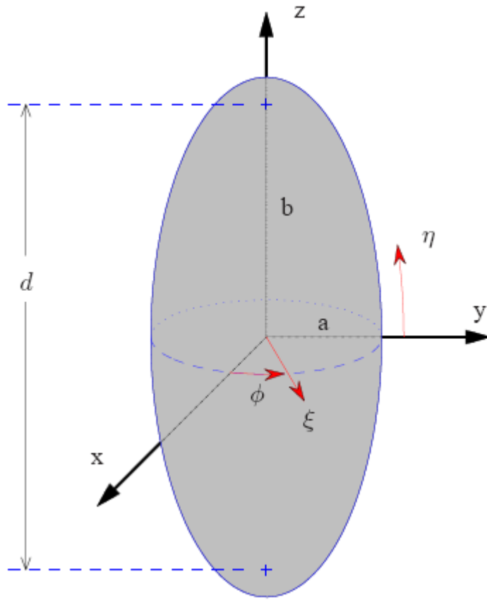
Figure 4-15: Spheroidal geometry.
