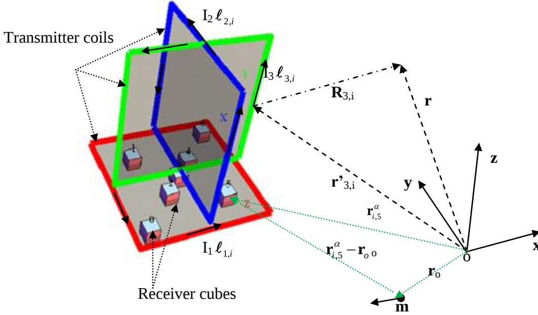
Figure 2. The MetalMapper geometry. The observation point \mathbf{r} is defined with respect to the global Cartesian coordinate system XYZO; \mathbf{r}'_{3,i} is the location of the i -th current element on (in this case) the T = 3 transmitter, which carries a current I_3 in the direction \ell_{3,i} .
