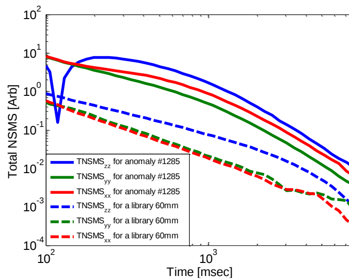
Figure 13: The total NSMS for MM anomaly #1285 (solid lines) and a library 60 mm mortar (dashed lines).
