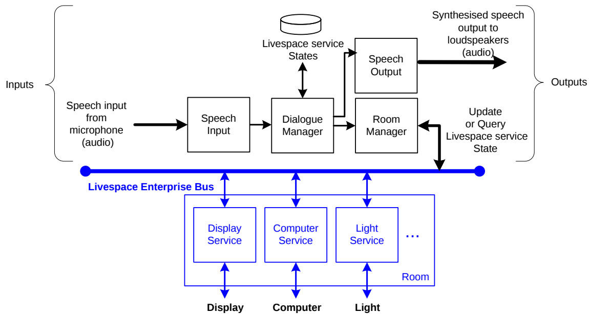
Figure 7 System components connecting room manager to Spoken Dialogue System and Livespaces
