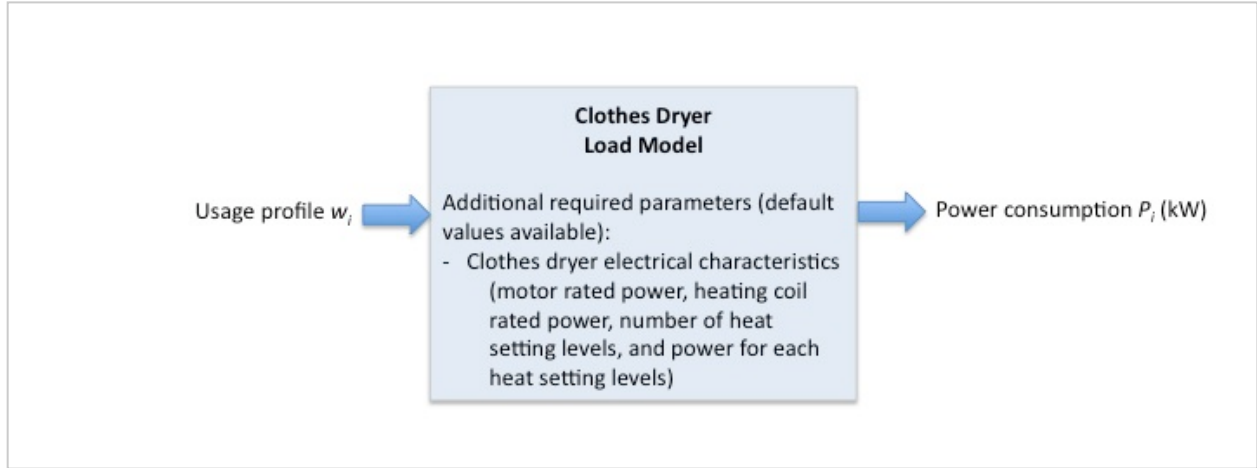
Fig. 4-22. Clothes dryer load model block diagram
