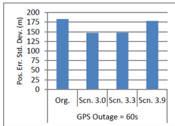
Figure 34: HG1700 inertial positioning errors with self-calibrated IMU errors according to different scenarios (see text) compared to the case without any prior self-calibration prior in the field.
