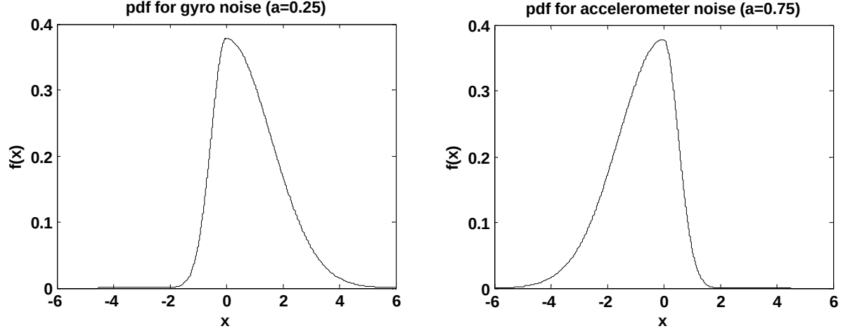
Figure 7: Asymmetric pdf's used for gyro noise ( l = 2 , a = 0.25 ) and accelerometer noise ( l = 2 , a = 0.75 ).
