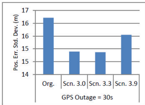
Figure 34: HG1700 inertial positioning errors with self-calibrated IMU errors according to different scenarios (see text) compared to the case without any prior self-calibration prior in the field.
