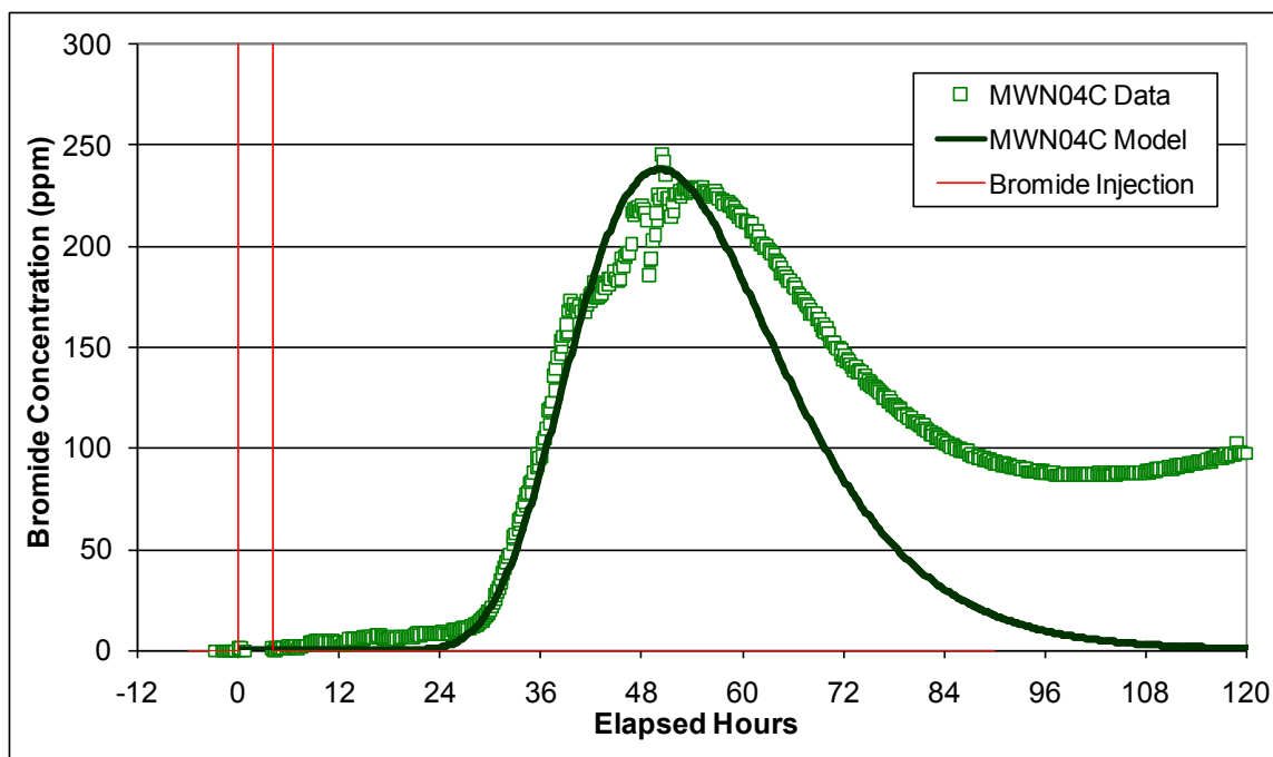
Figure D-29. Pre-TEE Tracer Tracer Response in the LSZ at MWN04C (Radius = 40.2 feet).
