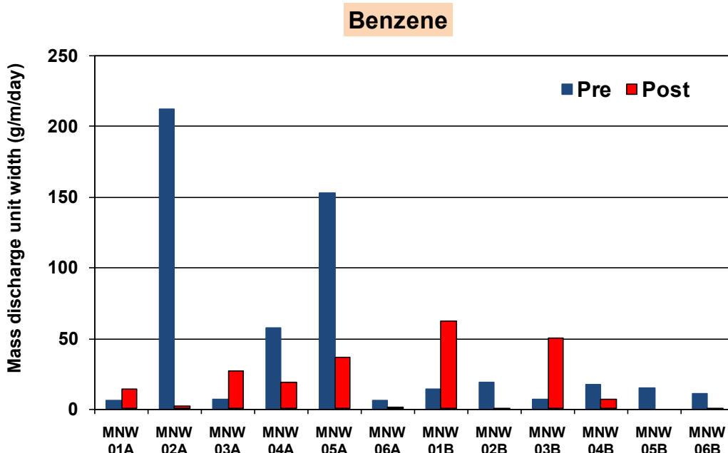
Figure D-39. Average Benzene Mass Fluxes for Pre- and Post-TEE Tests.
