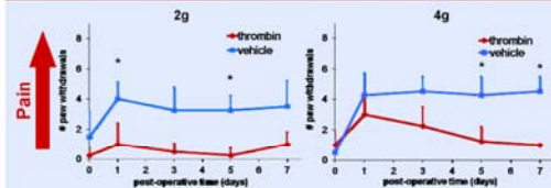
Fig. 2. Mechanical allodynia for testing with 2g and 4g von Frey filaments in the ipsilateral forepaw. Thrombin treated rats exhibit a significantly lower number of paw withdrawals overall for testing with the 2g ( p <0.004) and 4g ( p <0.009) filaments compared to those treated with vehicle. In addition, thrombin treatment significantly reduces allodynia on specific individual testing days compared to vehicle for both the 2g ( p <0.043) and the 4g ( p <0.026) filaments.
