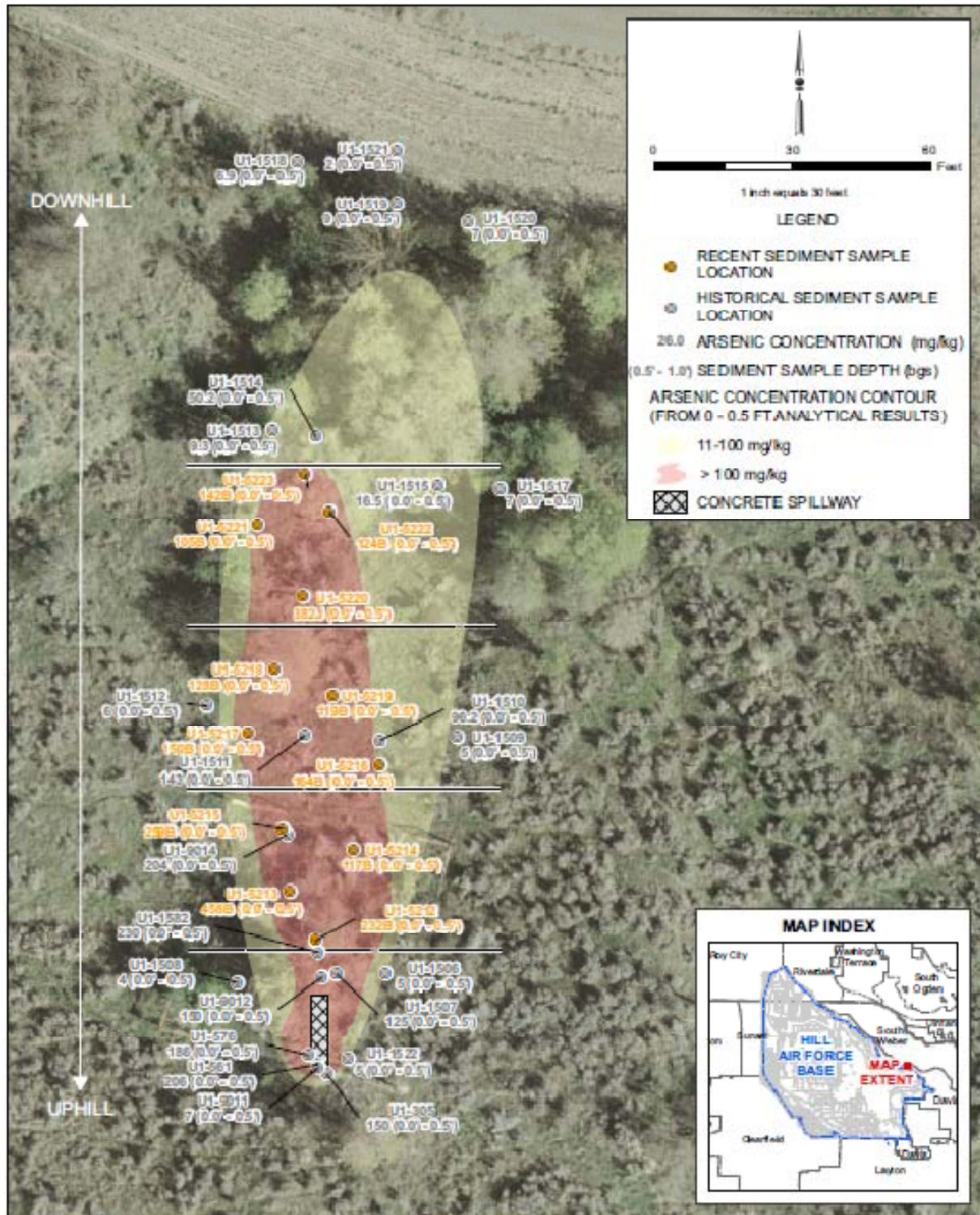
Figure 4-3. Site 2 Sediment Sample Locations
