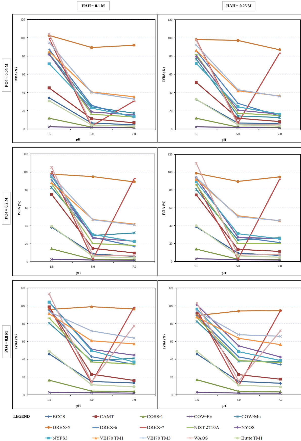
FIGURE 3-1b: IVBA vs pH (with PO 4 and HAH)
