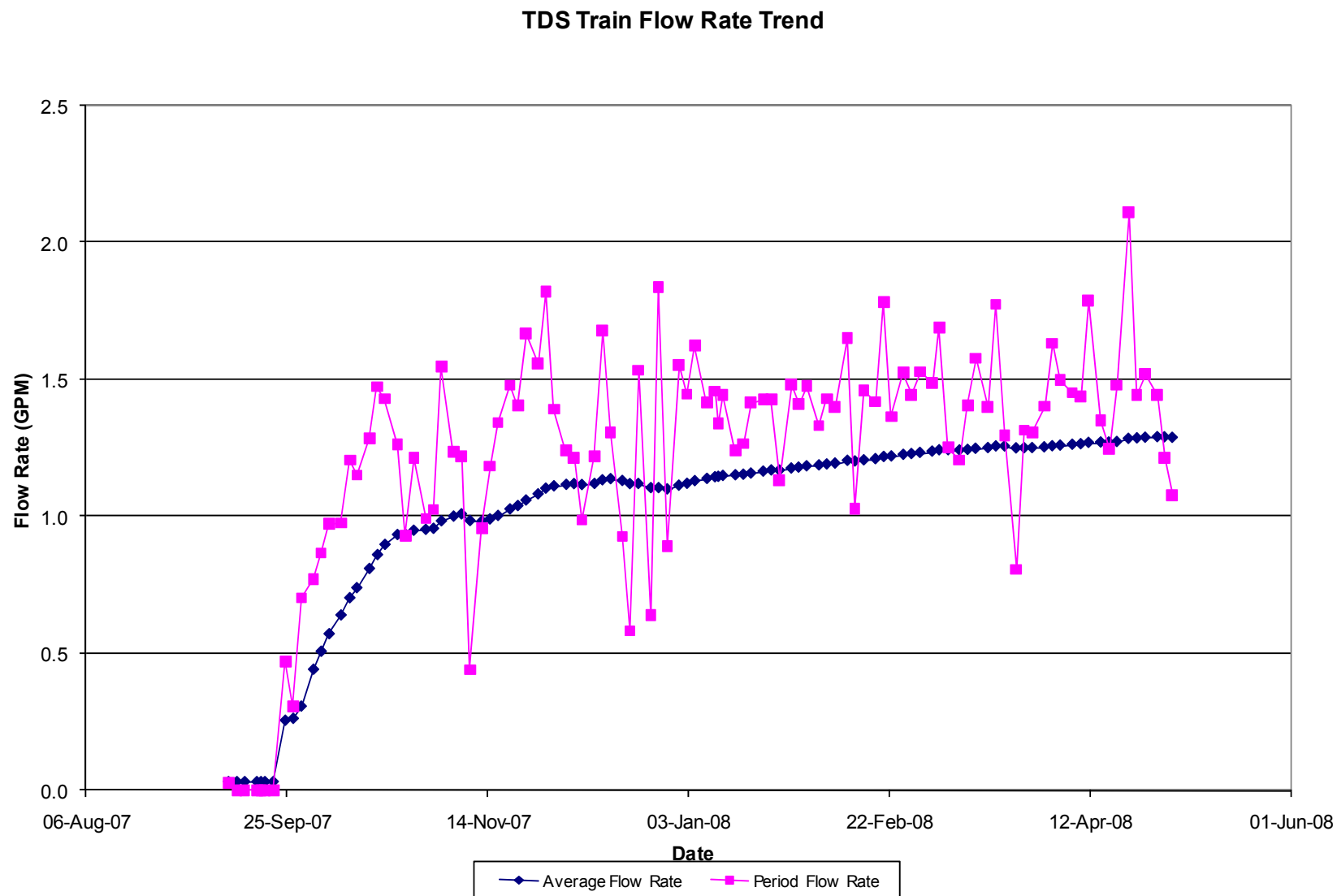
Figure 5-15. Flow Rate vs. Time TDS/Sulfate Train
