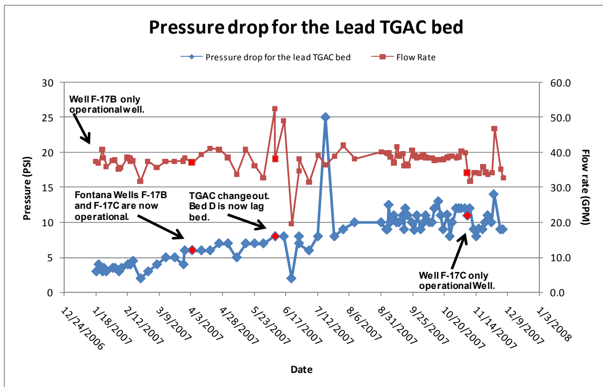
Figure 5-28. Pressure Drop across the Lead 38 GPM TGAC Bed vs. Time
