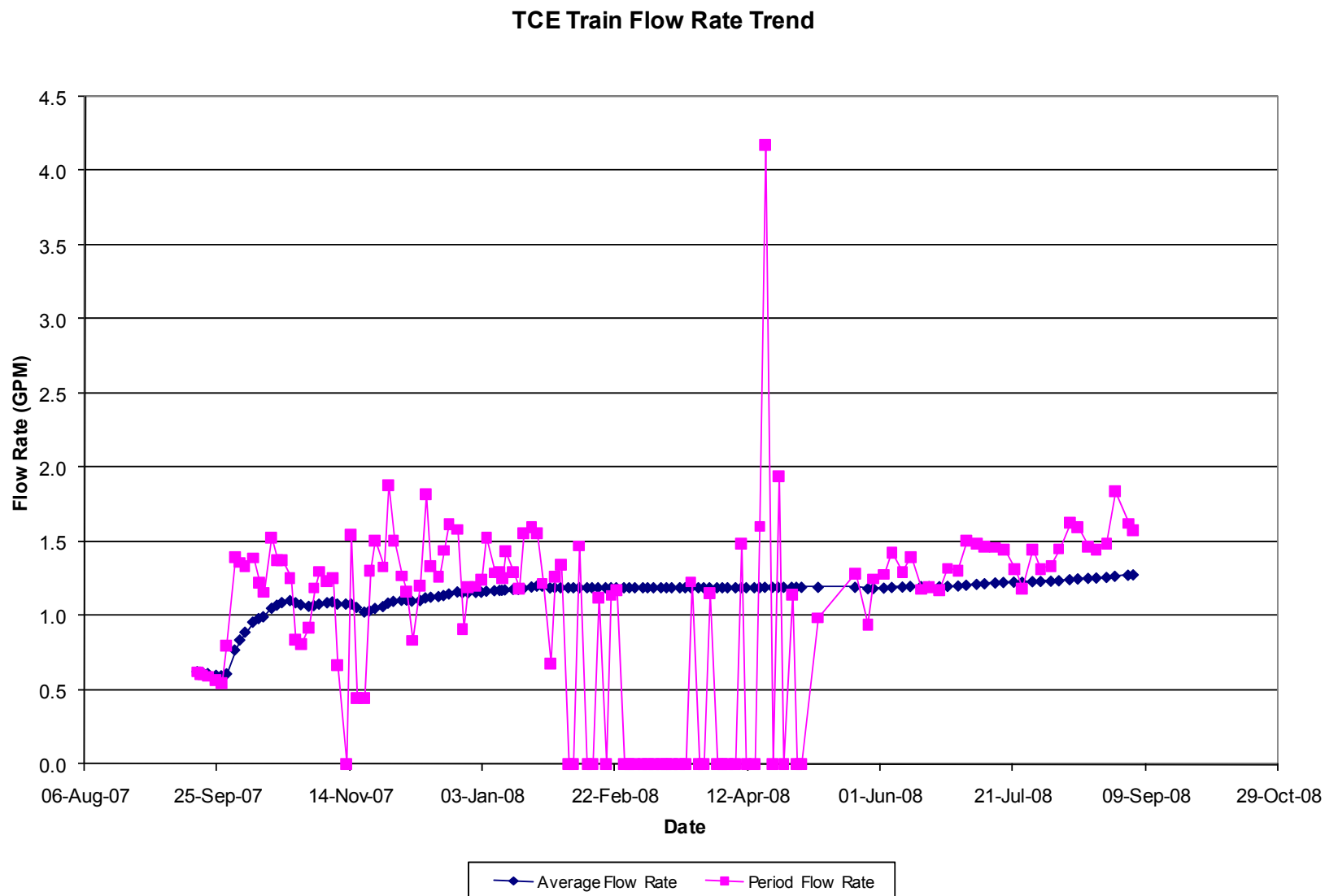
Figure 5-11. Flow Rate vs. Time TCE Spiked Train
