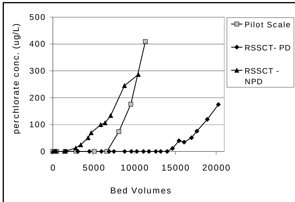
Figure 5. Comparison of RSSCT and pilot scale experiment for Perchlorate adsorption on TGAC using Penn State University tap water spiked with 500 µg/L perchlorate, using different intraparticle diffusion coefficients. PD is denotes that proportional diffusivity (exponent=1) was employed, while NPD denotes an exponent of 1.5
