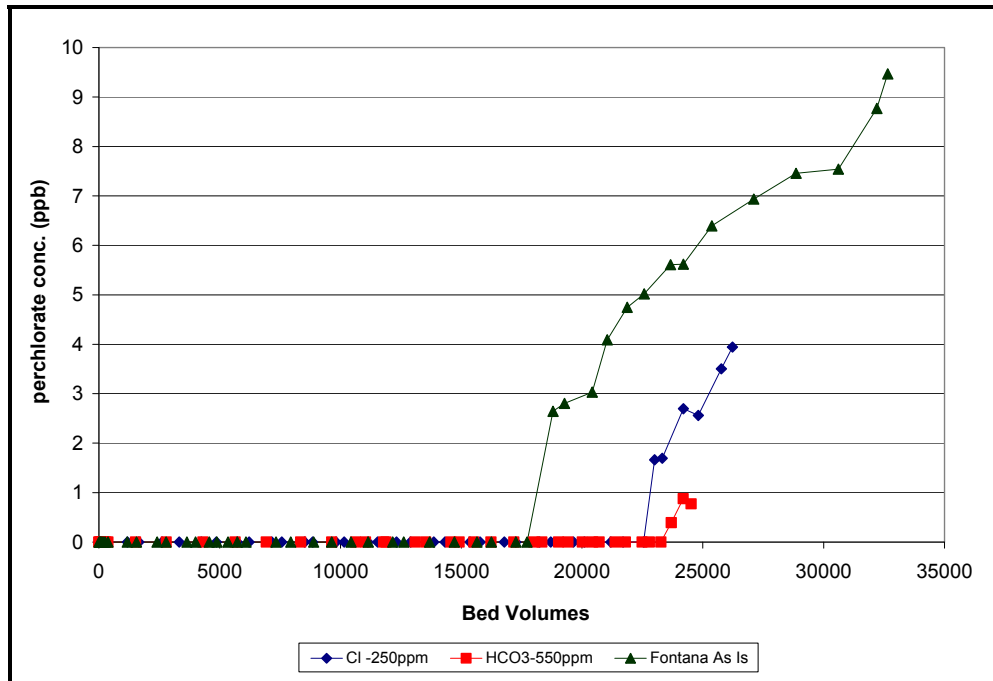
Figure 11. Graph Depicting the Effects of TDS on Perchlorate Adsorption to TGAC. Notation: - Cl- Chloride, HCO 3 - Bicarbonate
