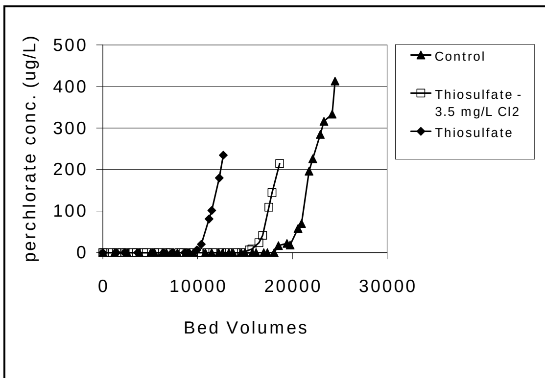
Figure - The effects of \text{S}_2\text{O}_3^{2-} concentration and pre-chlorination on \text{ClO}_4^- adsorption. Influent concentration was 500 \mu\text{g/L} \text{ClO}_4^- and 500 \mu\text{g/L} \text{S}_2\text{O}_3^{2-} with deionized distilled water.
