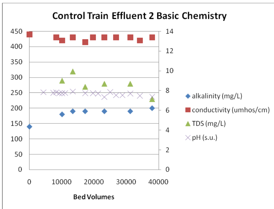
Figure 5-36. Effluent General Chemistry – Stratified Bed Control, Six Condition Pilot-Scale Test (BVs as measured through one bed)
