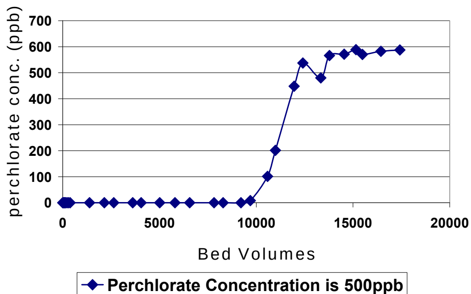
Figure 7. Perchlorate Breakthrough when Fontana Water is Spiked to 500 Ppb Perchlorate
