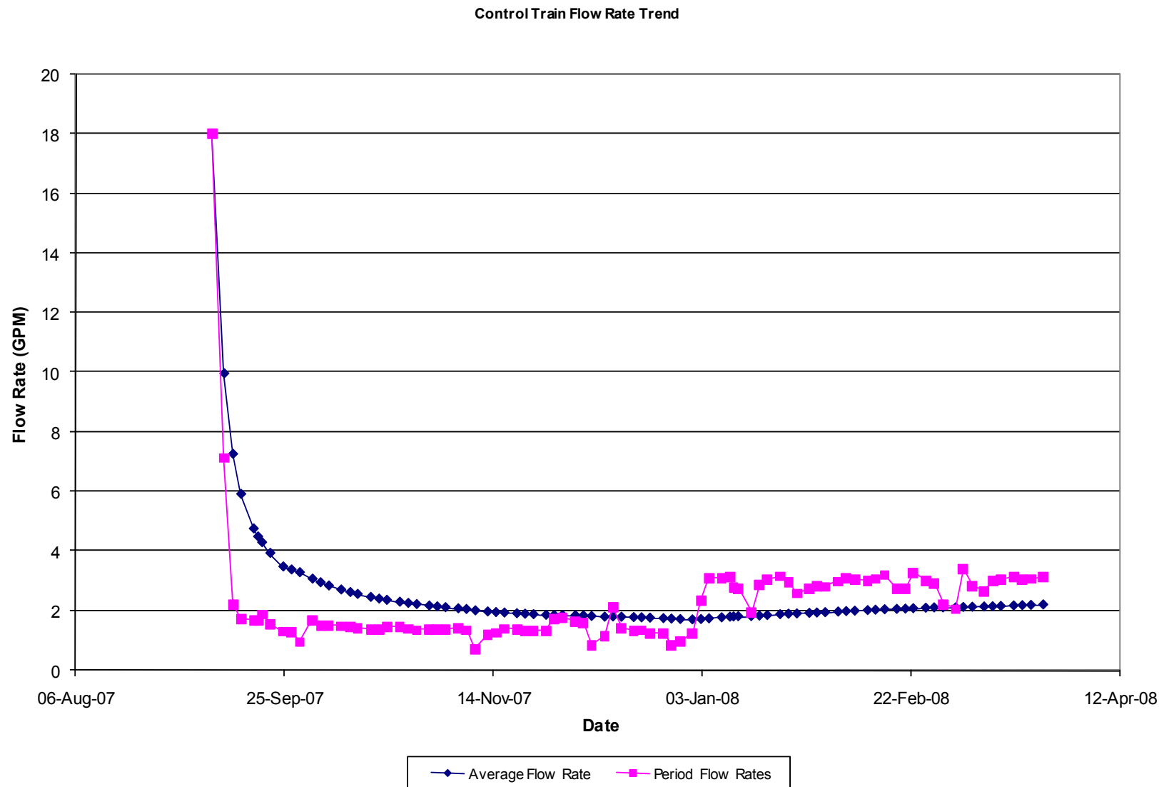
Figure 5-10. Flow Rate vs. Time Stratified Bed Control Train
