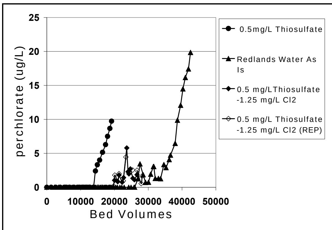
Figure - The effects of \text{S}_2\text{O}_3^{2-} and chlorine on the adsorption of \text{ClO}_4^- to surfactant tailored GAC when using Redlands water. Native \text{ClO}_4^- influent was 30 \mu\text{g/L} and Influent \text{S}_2\text{O}_3^{2-} spiked with 500 \mu\text{g/L} .
