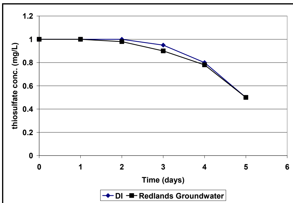
Figure - Rate of \text{S}_2\text{O}_3^{2-} oxidation in deionized distilled and Redlands groundwater, when the water source experienced incidental surface contact with air but with no mixing. Initial \text{S}_2\text{O}_3^{2-} is 1 mg/L.
