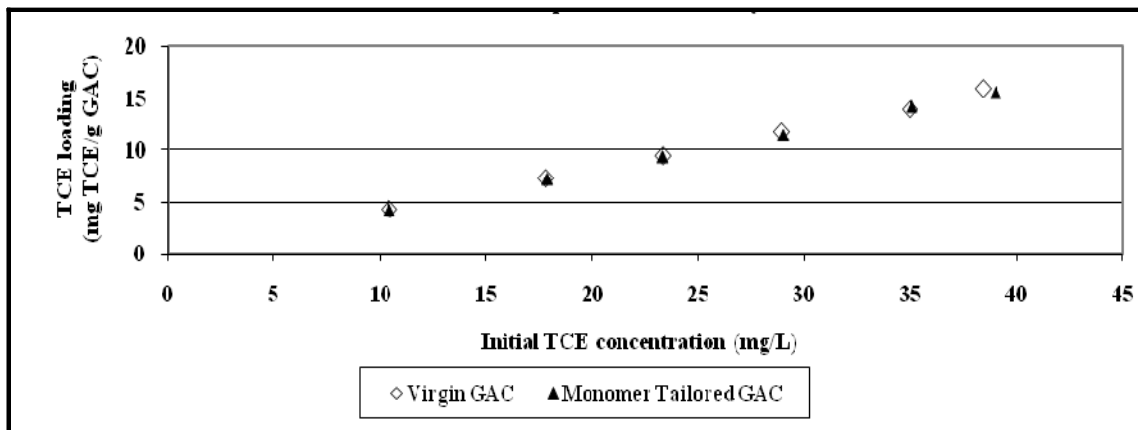
Figure 5-43. Isotherm Test for Effect of CTAC Preloading on Co-adsorption of TCE
