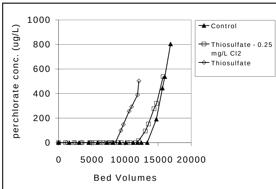
Figure - The effects \text{S}_2\text{O}_3^{2-} concentration and pre-chlorination on \text{ClO}_4^- adsorption. Influent concentration is 1000 \mu\text{g/L} \text{ClO}_4^- and 100 \mu\text{g/L} \text{S}_2\text{O}_3^{2-} , with deionized distilled water
