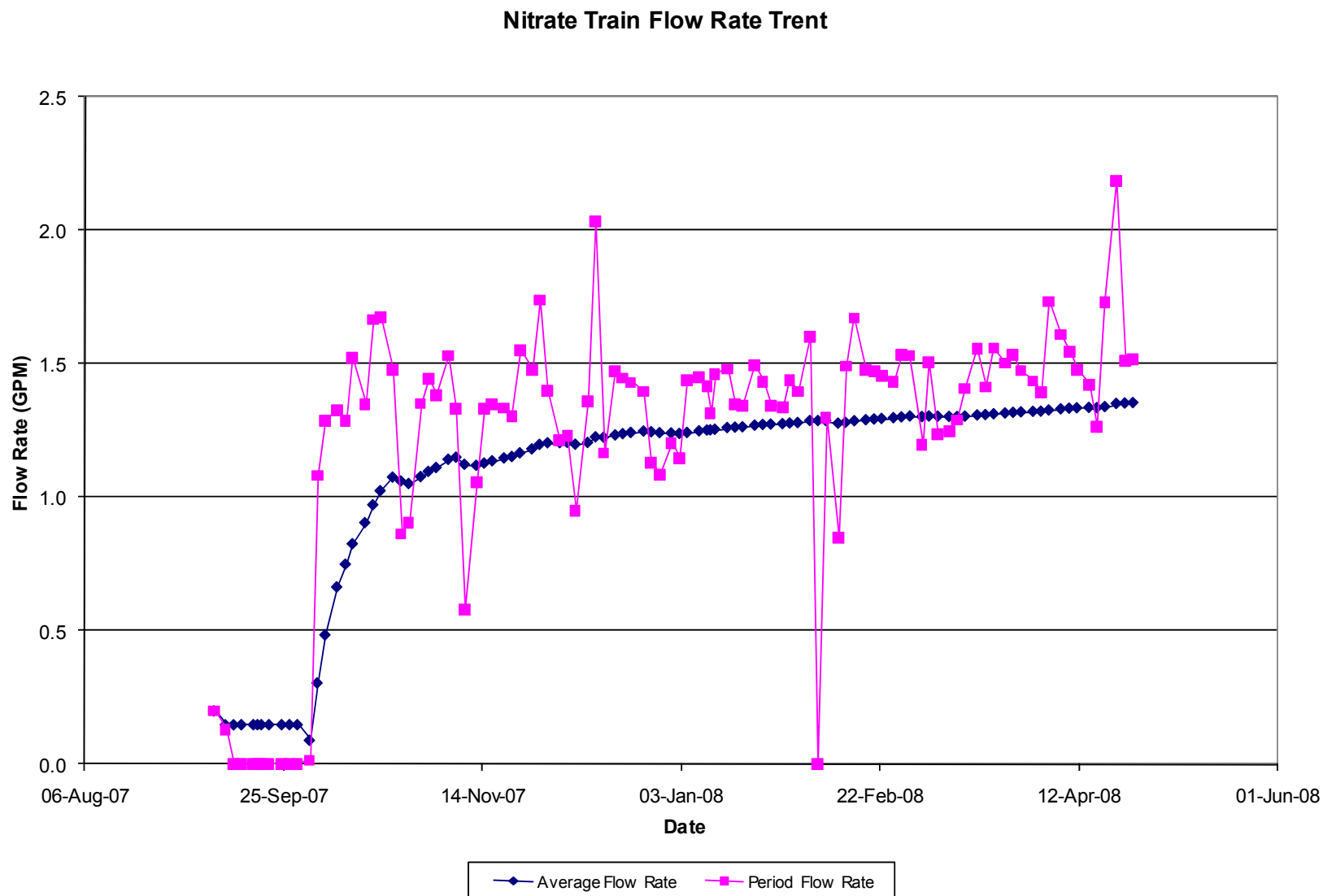
Figure 5-13. Flow Rate vs. Time Nitrate Spiked Train
