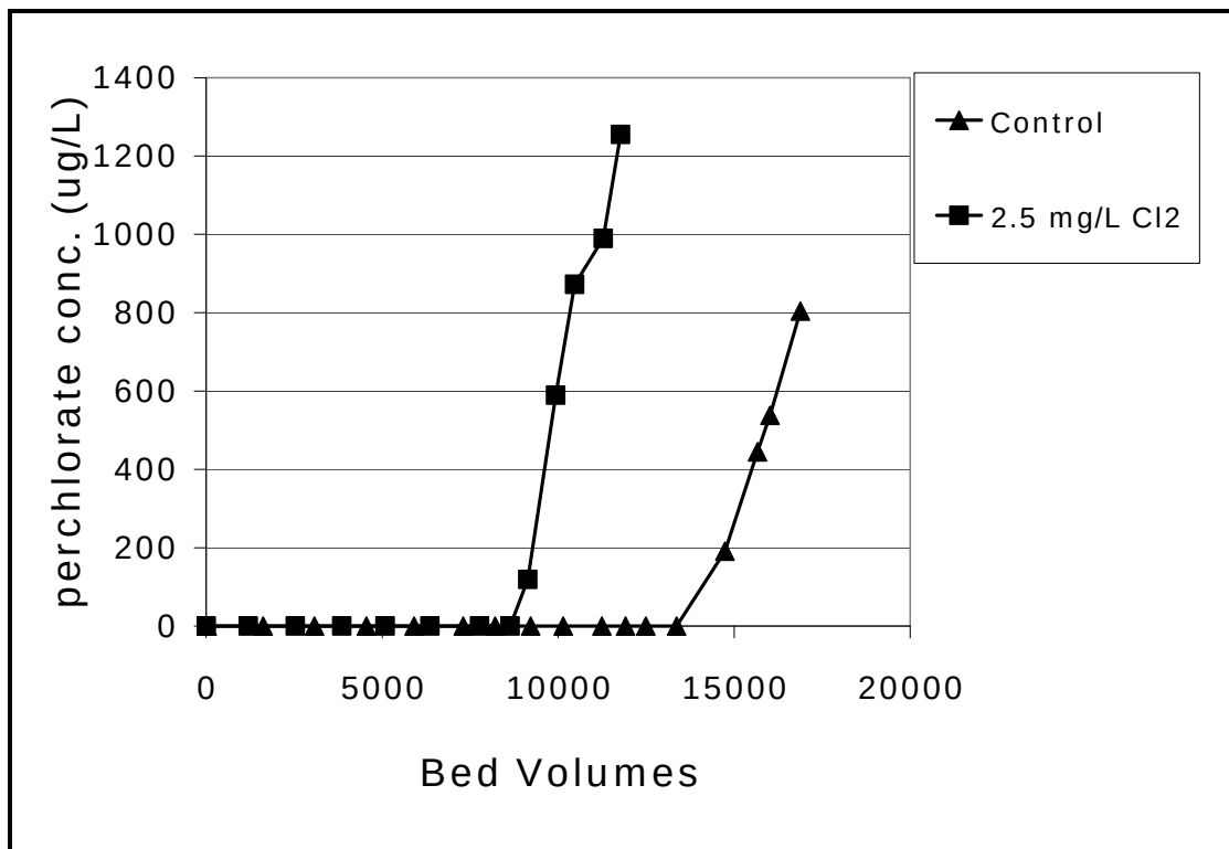
Figure - The effects of chlorination on \text{ClO}_4^- adsorption to the surfactant tailored GAC. The influent \text{ClO}_4^- concentration was 1,000 \mu\text{g/L} with deionized distilled water
