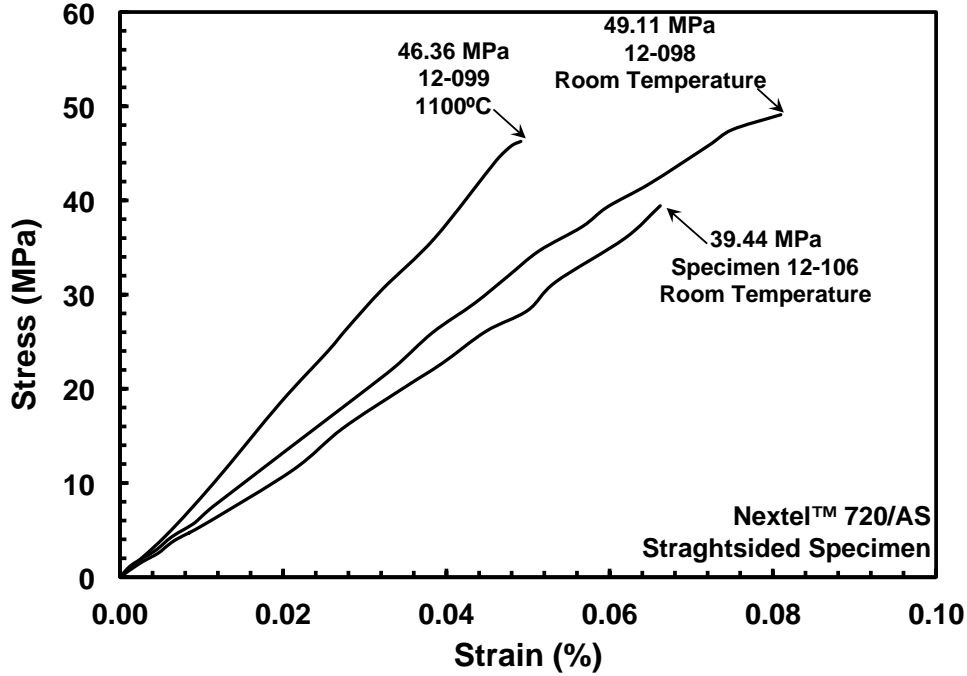
Figure 5.8: Stress vs. Strain curves obtained in tension test of Nextel™ 720/AS straghtsided specimens 12-098, 12-099, and 12-106
