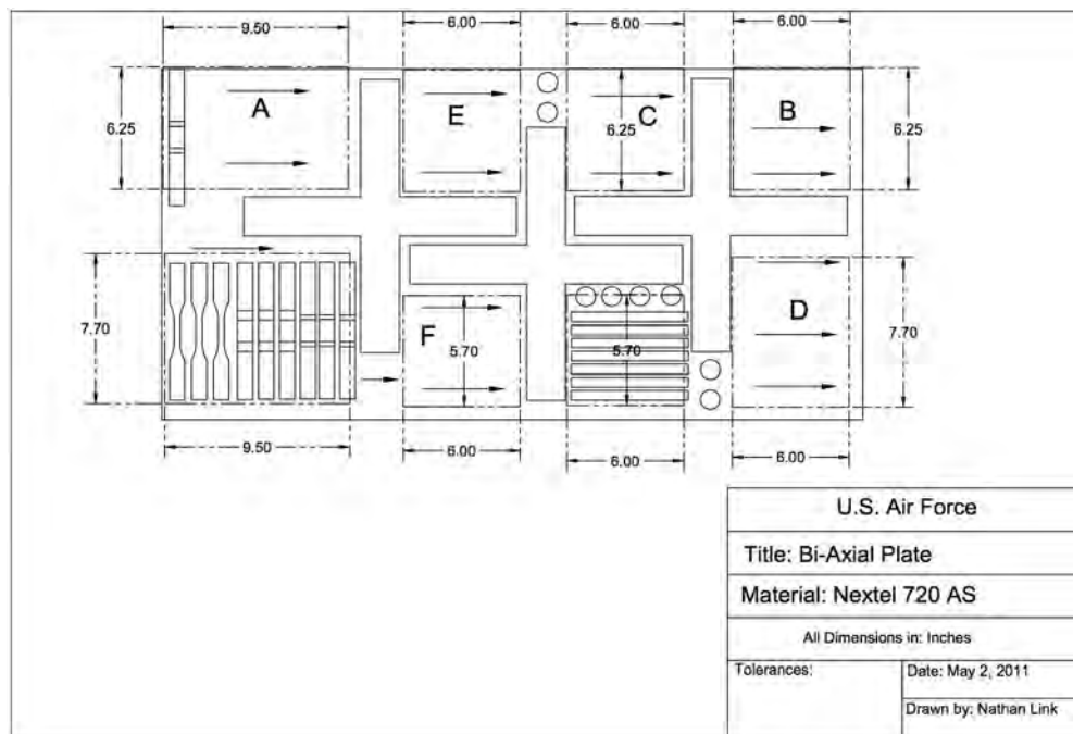
Figure 3.9: Baseline Nextel™ 720/AS Balanced 0°/90° plate
