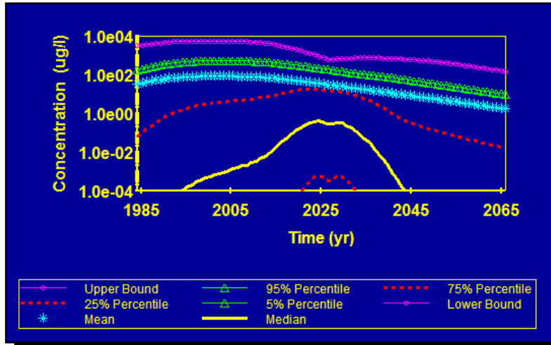
17d. Thermal Treatment – TCE Concentrations at River.
