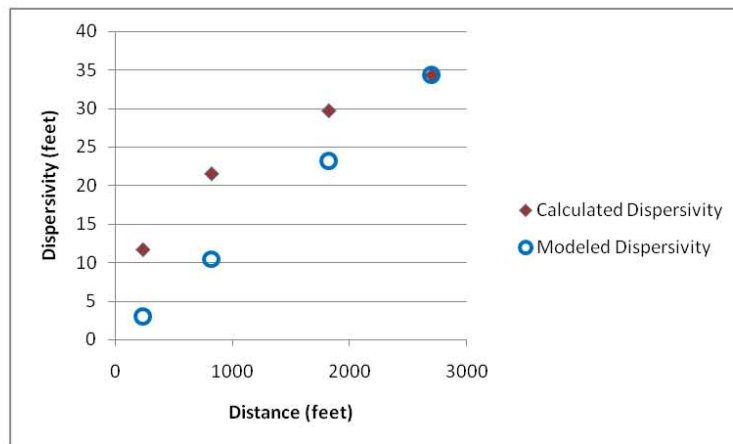
Figure 5: Modeled vs Calculated Dispersivity.
