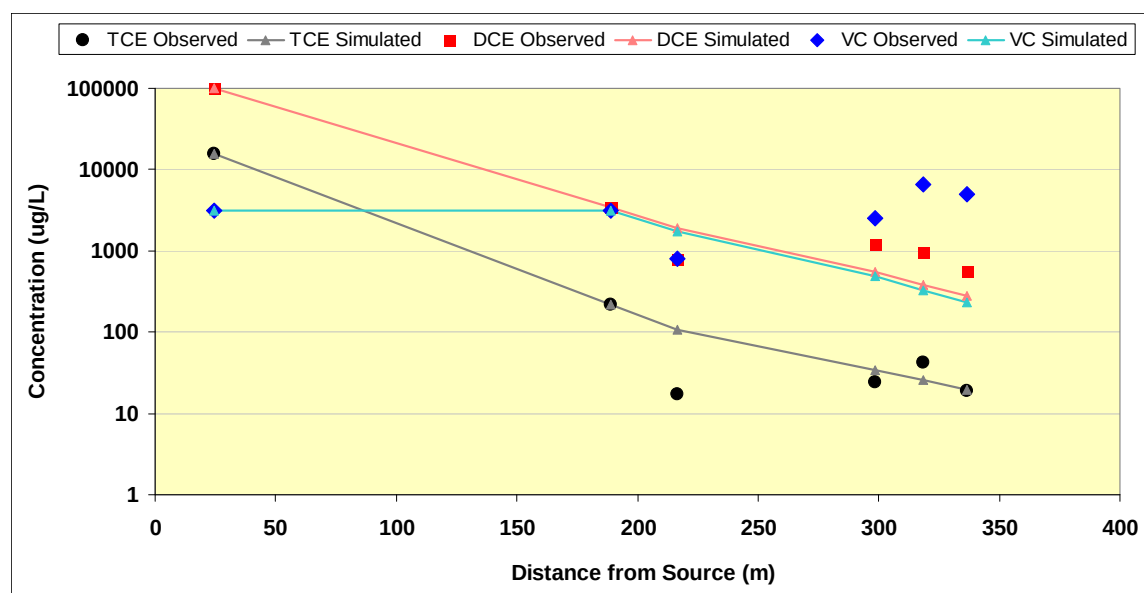
Figure 16. Final Calibration of TCE, DCE, and VC.
