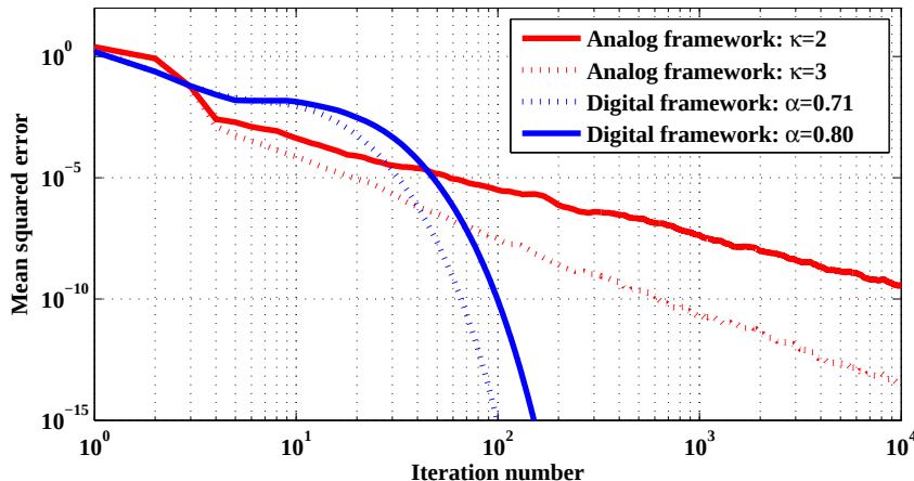
Figure 1. Mean squared error versus iteration number
