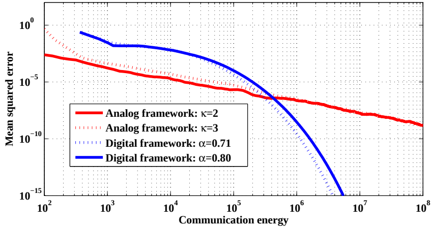
Figure 2. Mean squared error versus communication energy
