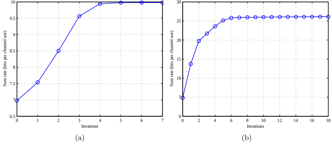
Figure 8. Convergence examples of the WMMSE algorithm: (a) SISO-IFC, K = 3 , \epsilon = 1e - 3 ; (b) MIMO-IFC, K = 4 , T = 3 , R = 2 , \epsilon = 1e - 2 .
