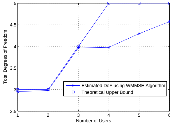
Figure 3. Achievable DoF and theoretical upper bound
