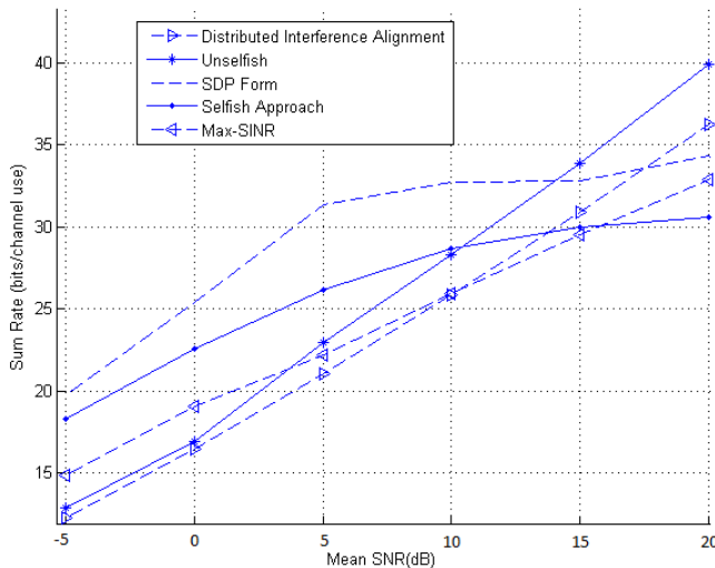
Figure 4. Sum-rate vs. SNR: K = 4, M = 3, d = 1
