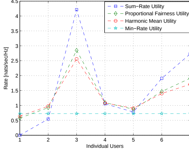
Figure 5. Individual rate distribution with K = 7, L = 4 and P = 30 dBm.
