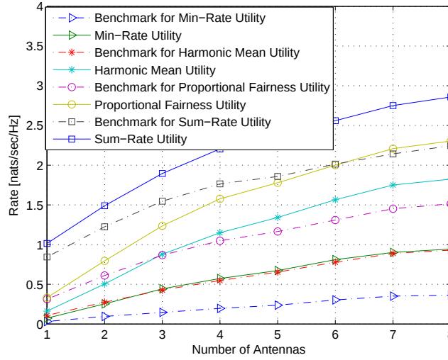
Figure 6. Performance comparison of coordinated beamformers and space matched beamformers with K = 7, P = 30 dBm.
