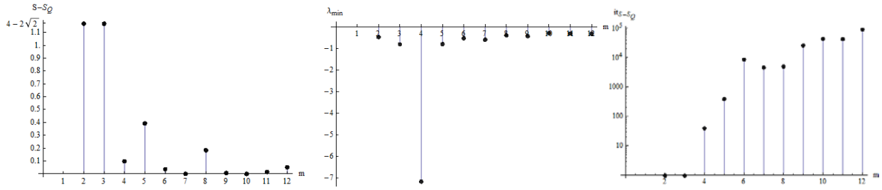
Figure 4. (left) Numerical simulations for m = \{2, 3, 4, \dots, 12\} measurement vectors yielding valid joint probabilities 0 \leq P(a, b | x = \vec{m}_i, y = \vec{n}_j) \leq 1 for all pairs of measurement vectors \{\vec{m}_i, \vec{n}_j\}_{i, j \in \{0, 1, \dots, m-1\}} and supra-correlations S - S_Q > 0 . (middle) Minimum eigenvalue \lambda_{\min} of O in (18). The negative values indicates that O is not a proper quantum state (positive, Hermitian operator, \rho \geq 0 ). (right) Iteration number (out of 10^5 random trials) at which the first set of m measurements vectors were found for Alice and Bob producing supra-correlation shown in the leftmost figure.
