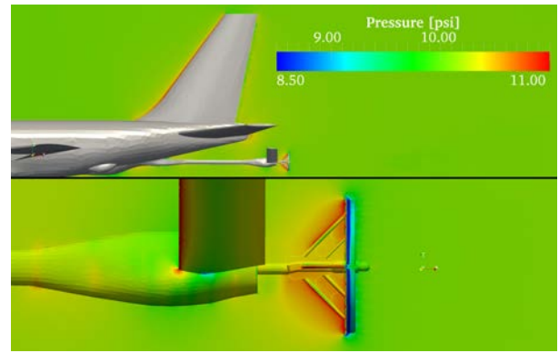
(b) Pressure Contours
