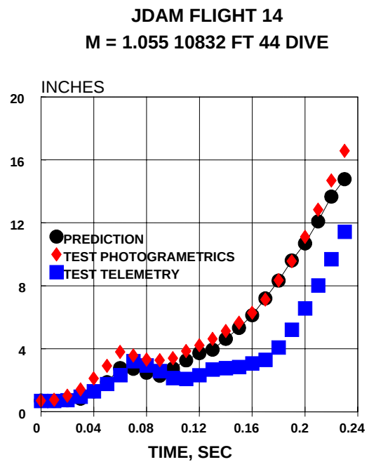
FIGURE 7 JDAM MISS DISTANCE
