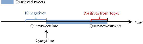
Figure 2: Illustration of constructing training data for classification.
