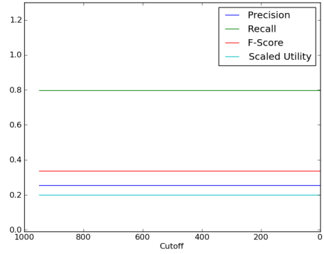
Figure 2: DbPedia.
