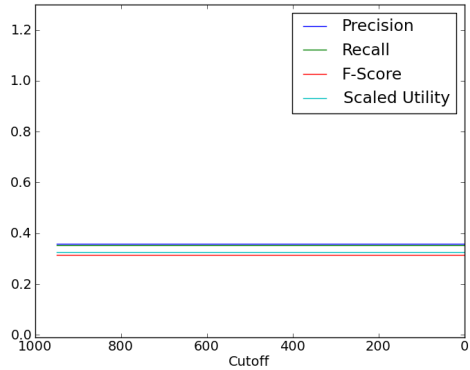
Figure 3: Prefix-suffix learning.
